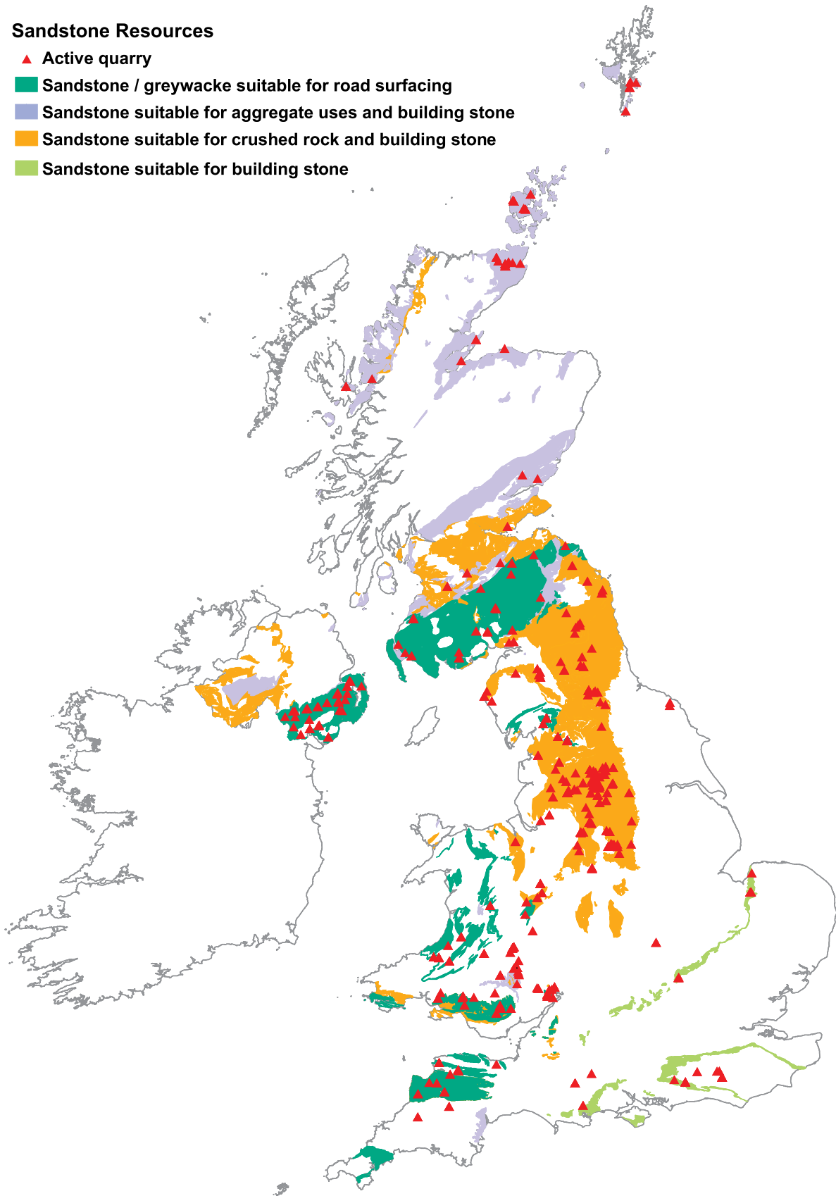
Figure 6 Sandstone resources and workings in the UK in 2010.
