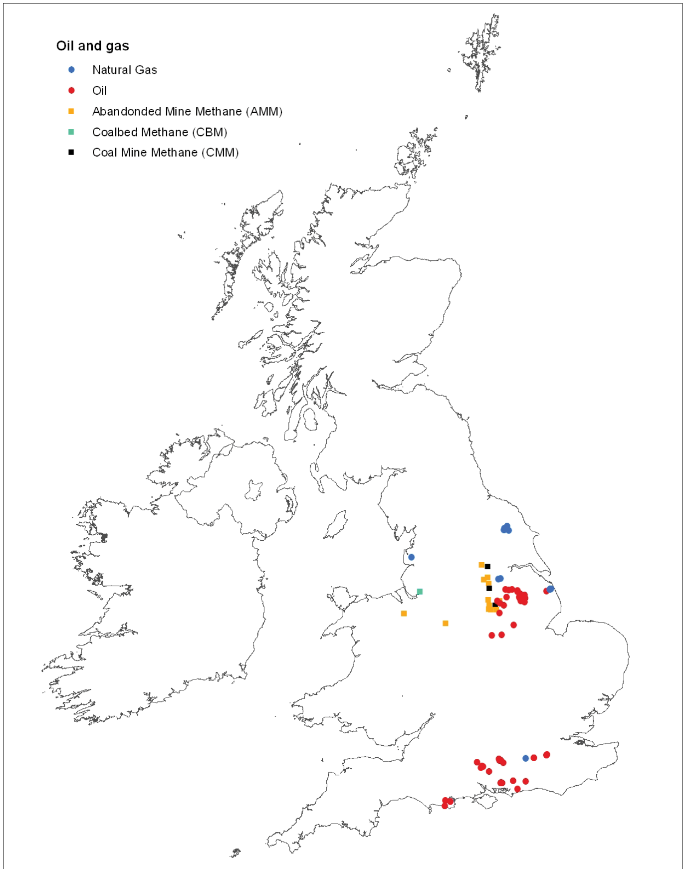
Figure 8 Onshore Oil and Natural Gas workings in the UK in 2010.
