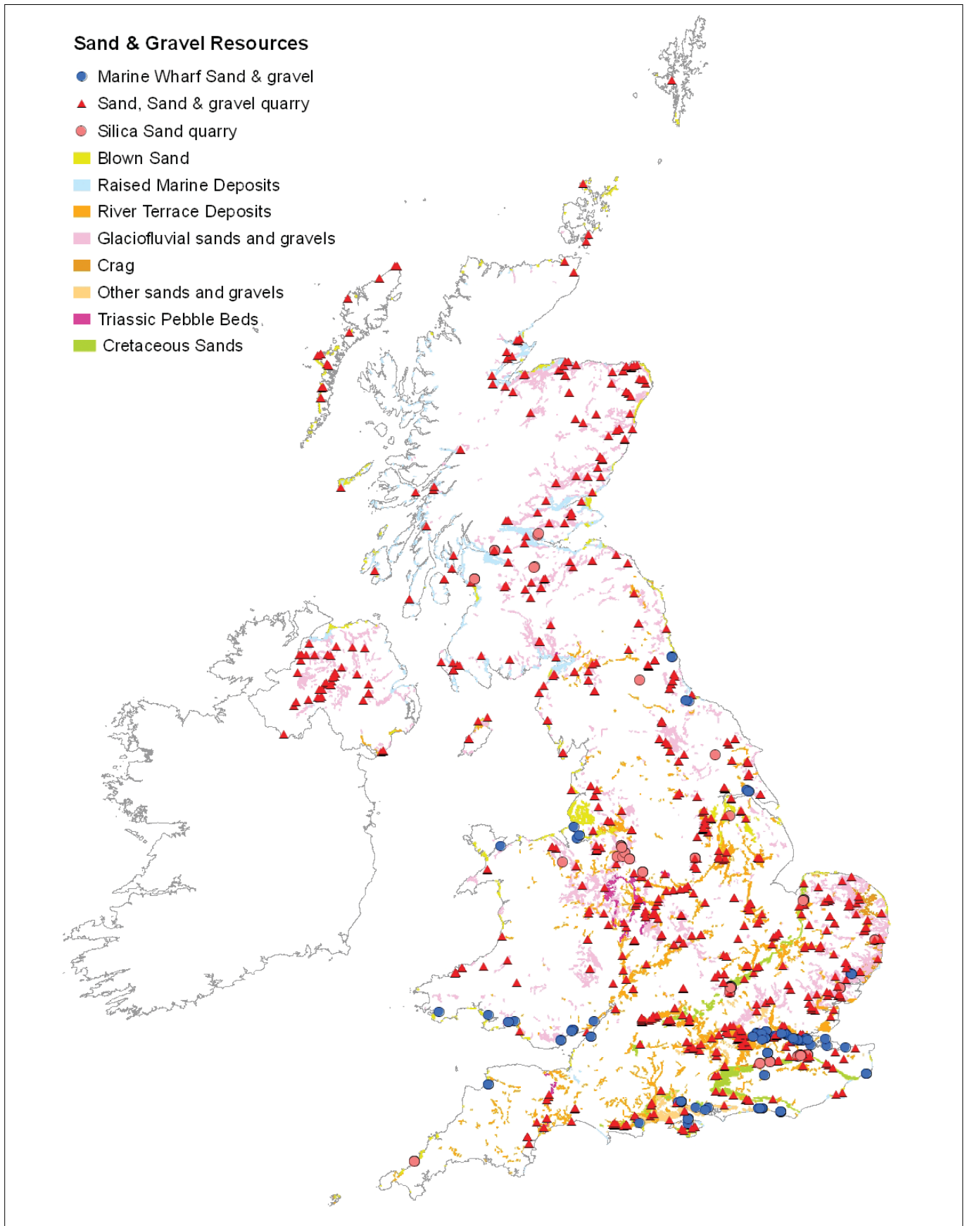
Figure 5 Sand and gravel resources and workings in the UK in 2010.
