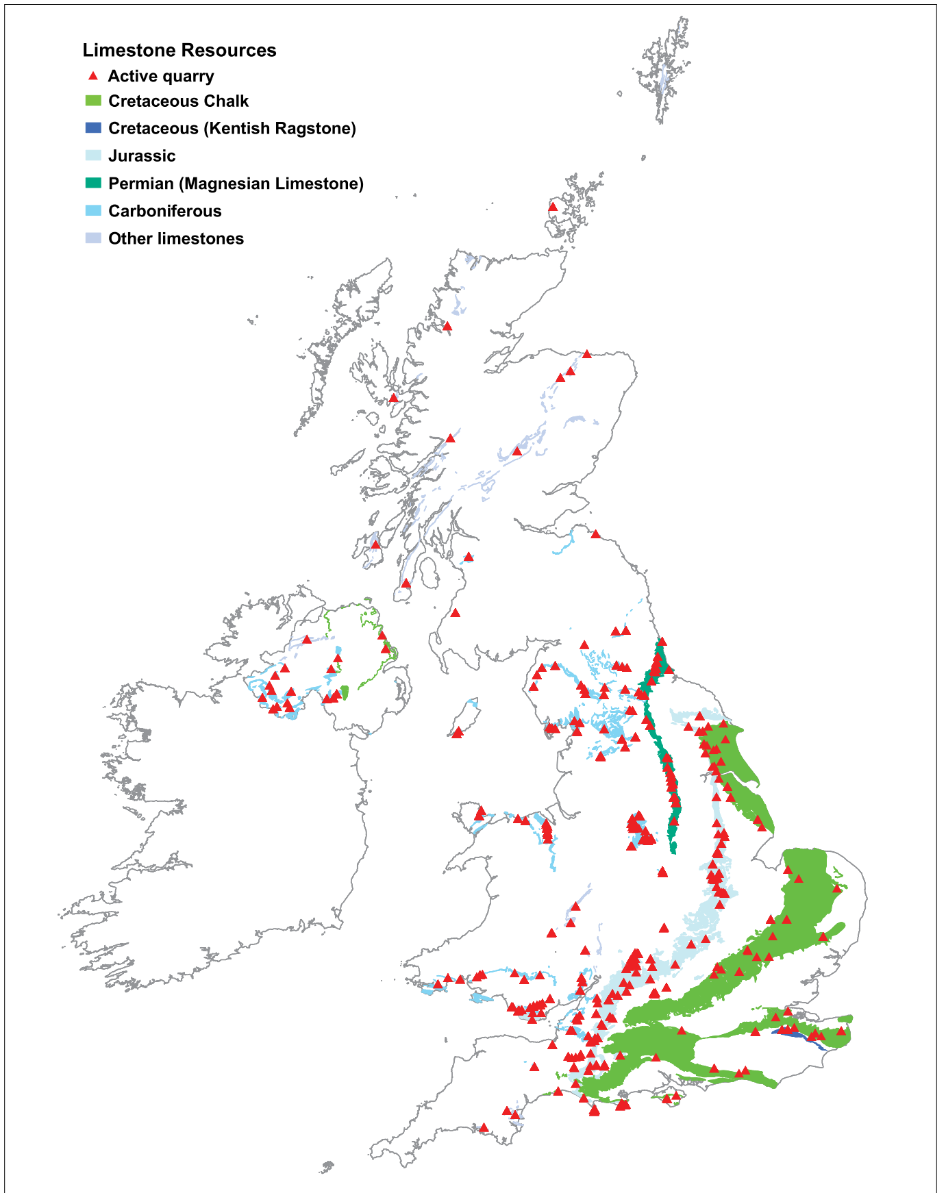
Figure 4 Limestone resources and workings in the UK in 2010.
