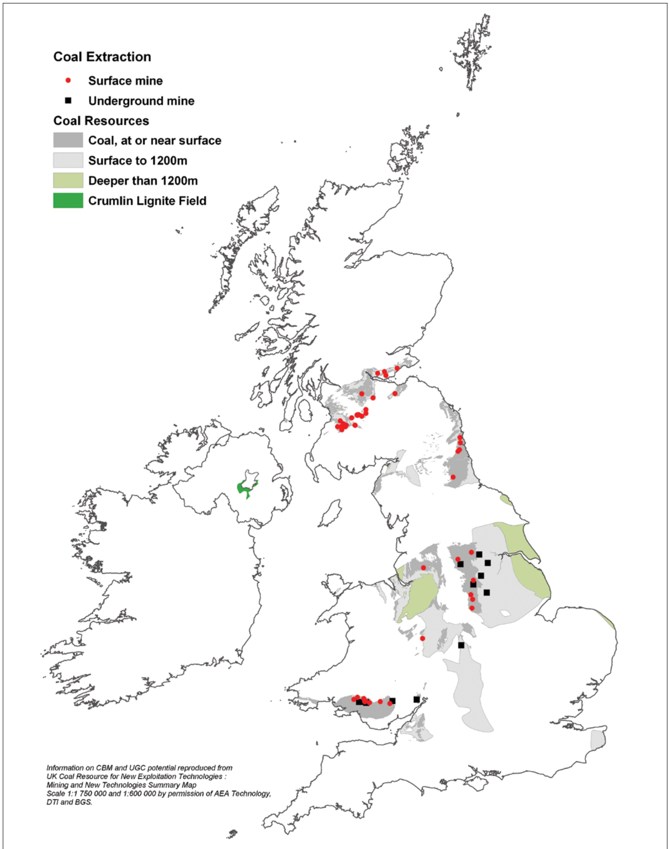
Figure 7 Coal resources and workings in the UK in 2010.
