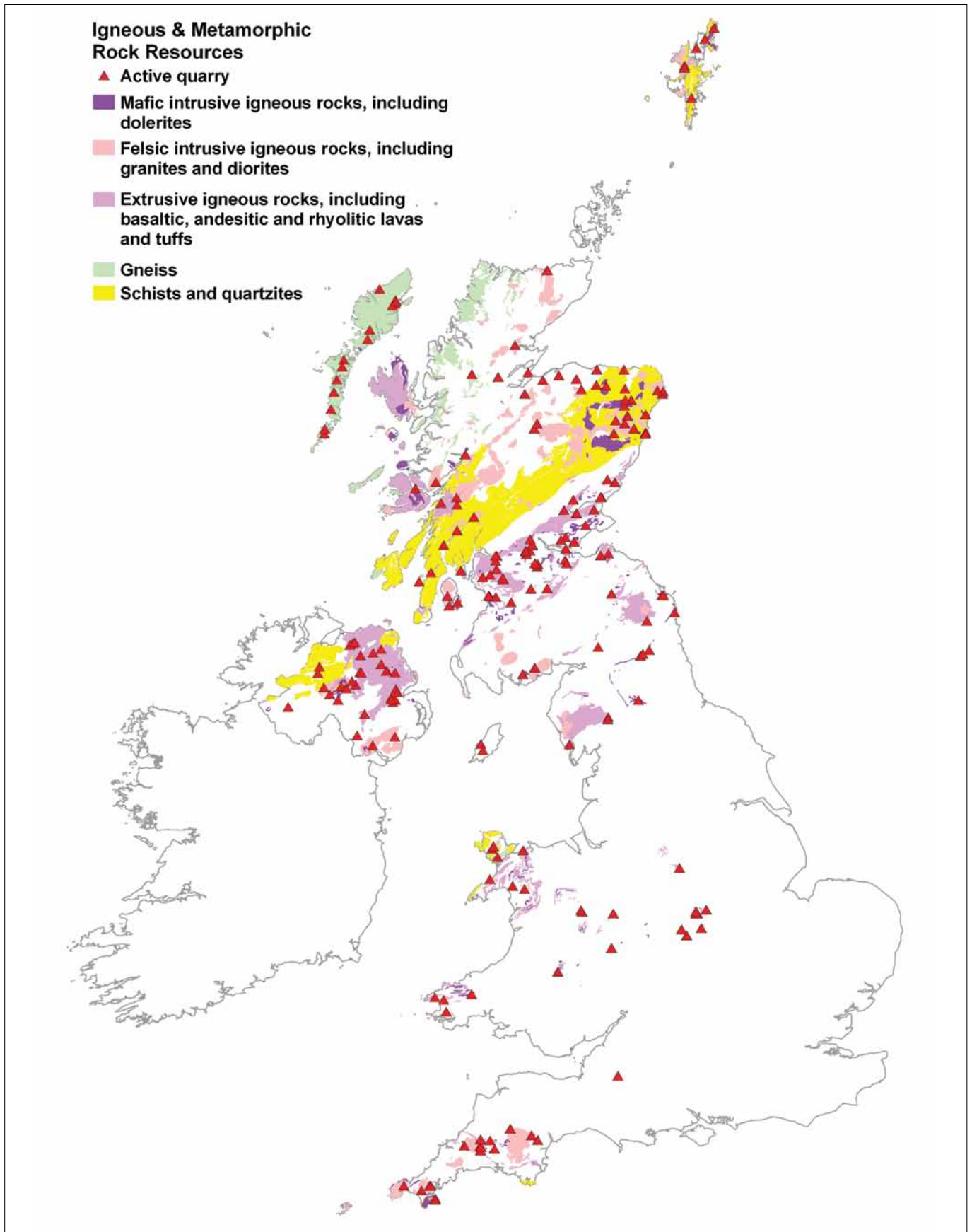
Figure 3 Igneous & metamorphic rock resources and workings in the UK in 2010.
