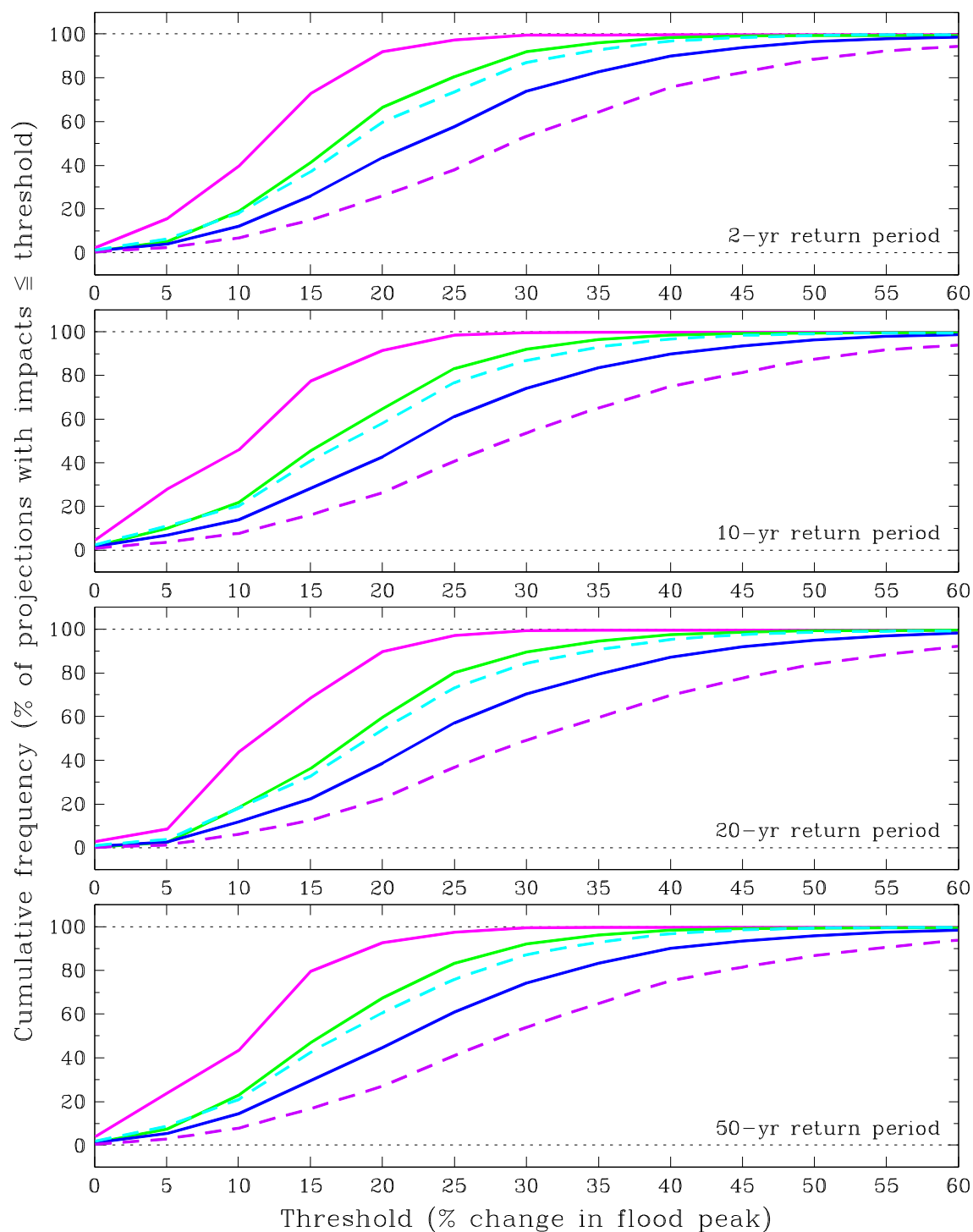
Figure B.48 As Figure B.45 but for the Forth river-basin region.
