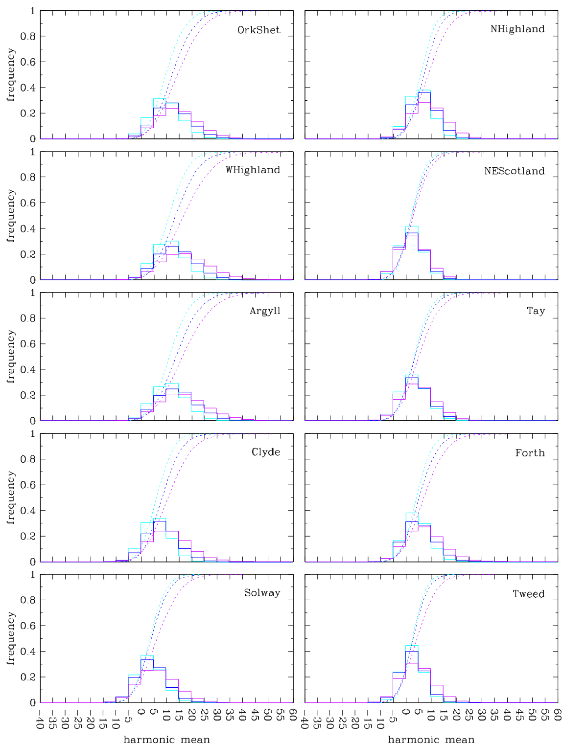
Figure A.5 Histograms and cdfs of the means of the harmonic functions fitted to the UKCP09 precipitation Sampled Data (2080s: Low emissions – cyan, Medium emissions – blue, High emissions – purple), for each of the 10 river-basin regions in Scotland.
