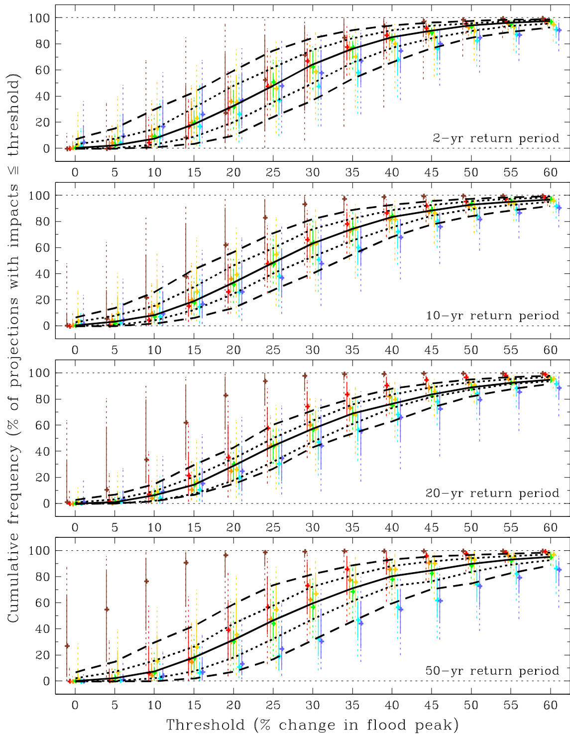
Figure B.33 As Figure B.31 but for the Tay river-basin region (2080s High).
