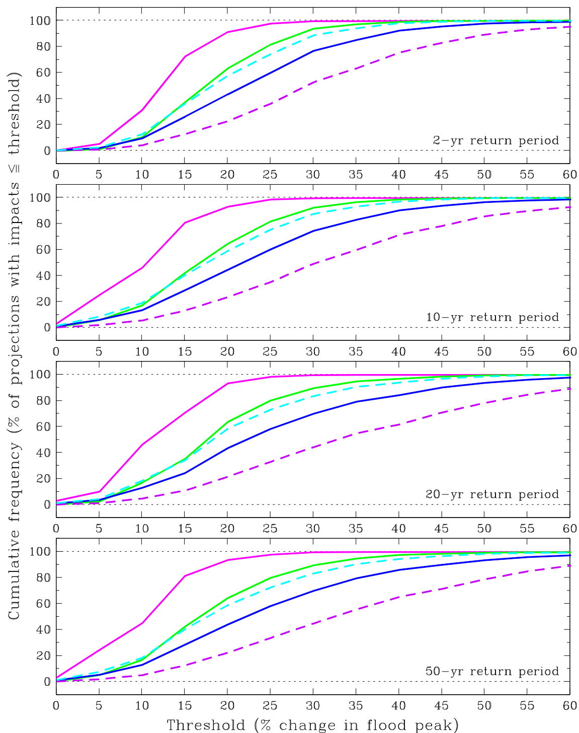
Figure B.50 As Figure B.45 but for the Solway river-basin region.
