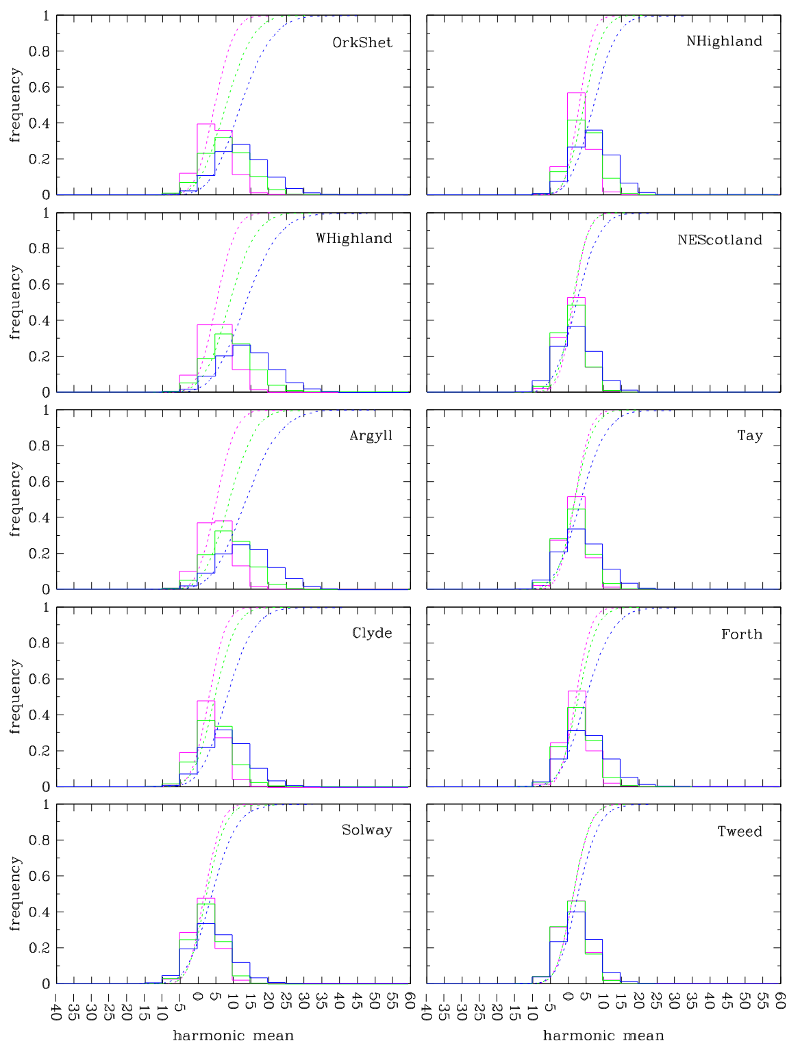
Figure A.1 Histograms and cdfs of the means of the harmonic functions fitted to the UKCP09 precipitation Sampled Data (Medium emissions: 2020s – magenta, 2050s – green, 2080s – blue), for each of the 10 river-basin regions in Scotland.
