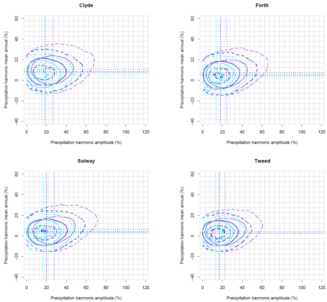
Figure A.8 continued.
