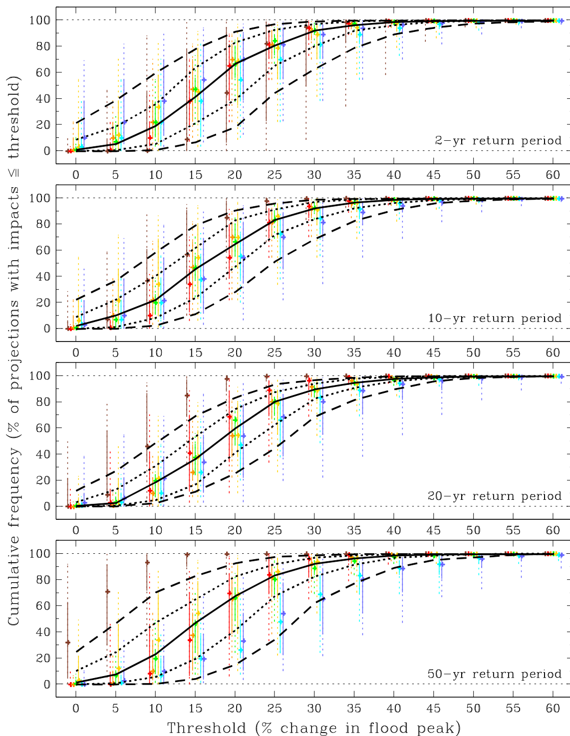
Figure B.14 As Figure B.11 but for the Forth river-basin region (2050s Medium).
