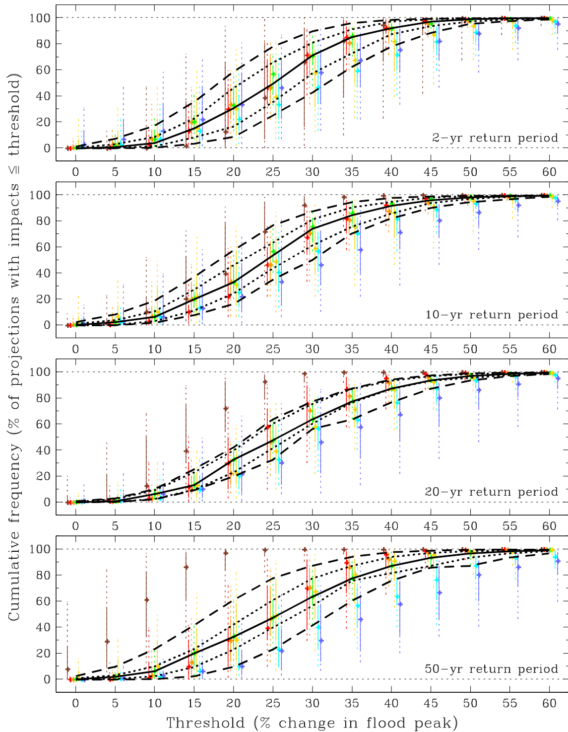
Figure B.18 As Figure B.11 but for the Argyll river-basin region (2050s Medium).
