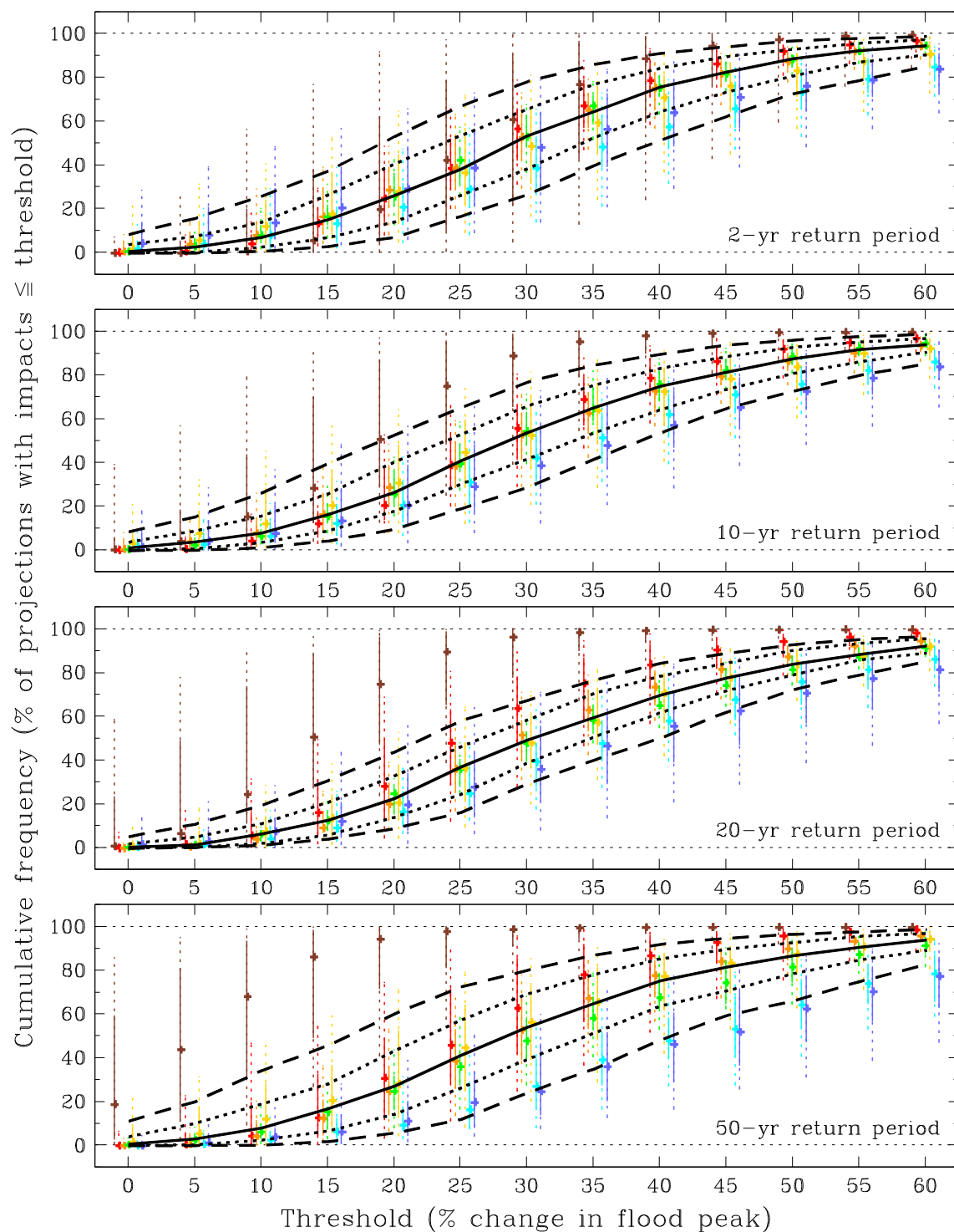
Figure B.34 As Figure B.31 but for the Forth river-basin region (2080s High).
