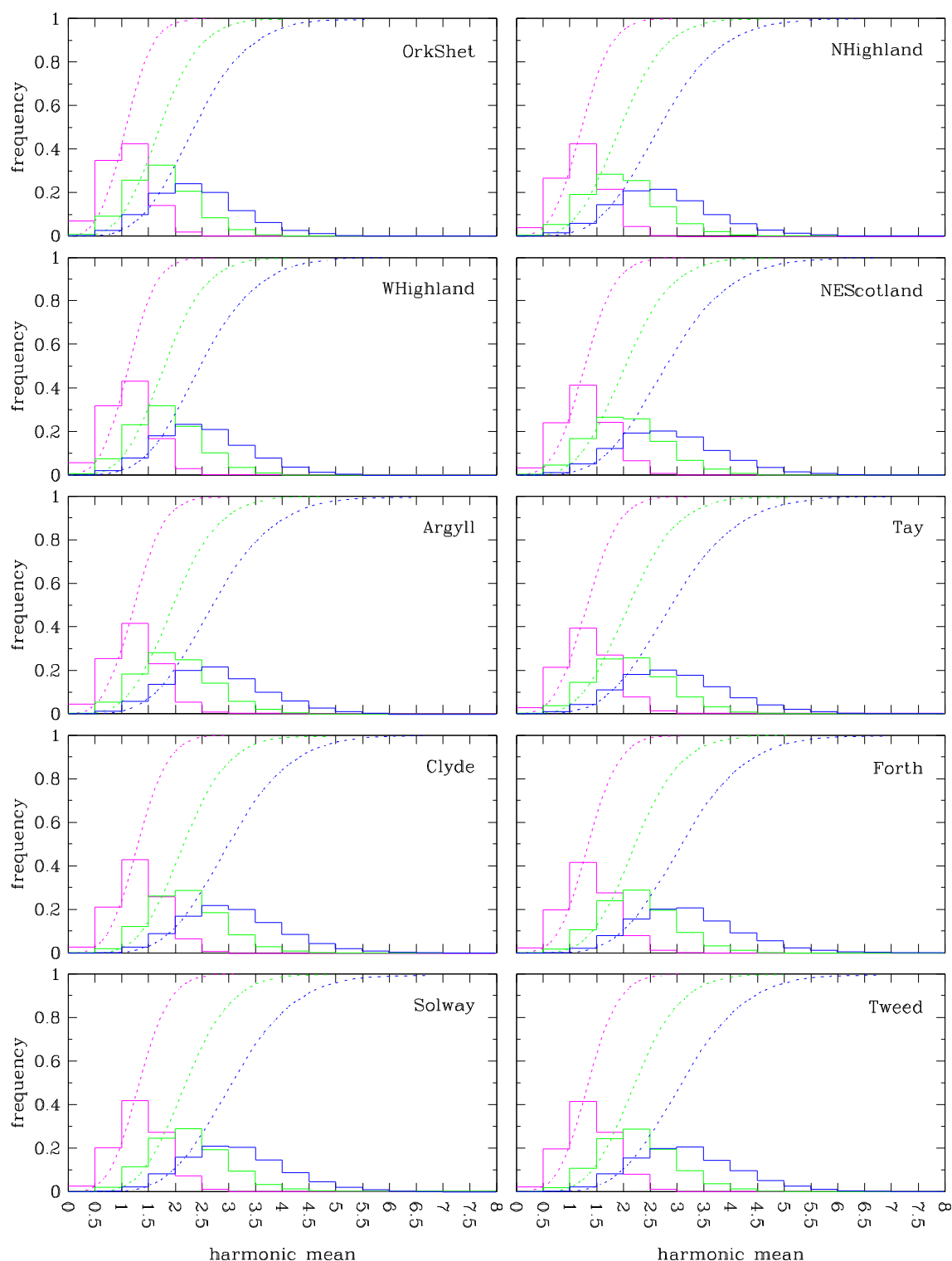
Figure A.9 Histograms and cdfs of the means of the harmonic functions fitted to the UKCP09 temperature Sampled Data (Medium emissions: 2020s – magenta, 2050s – green, 2080s – blue), for each of the 10 river-basin regions in Scotland.
