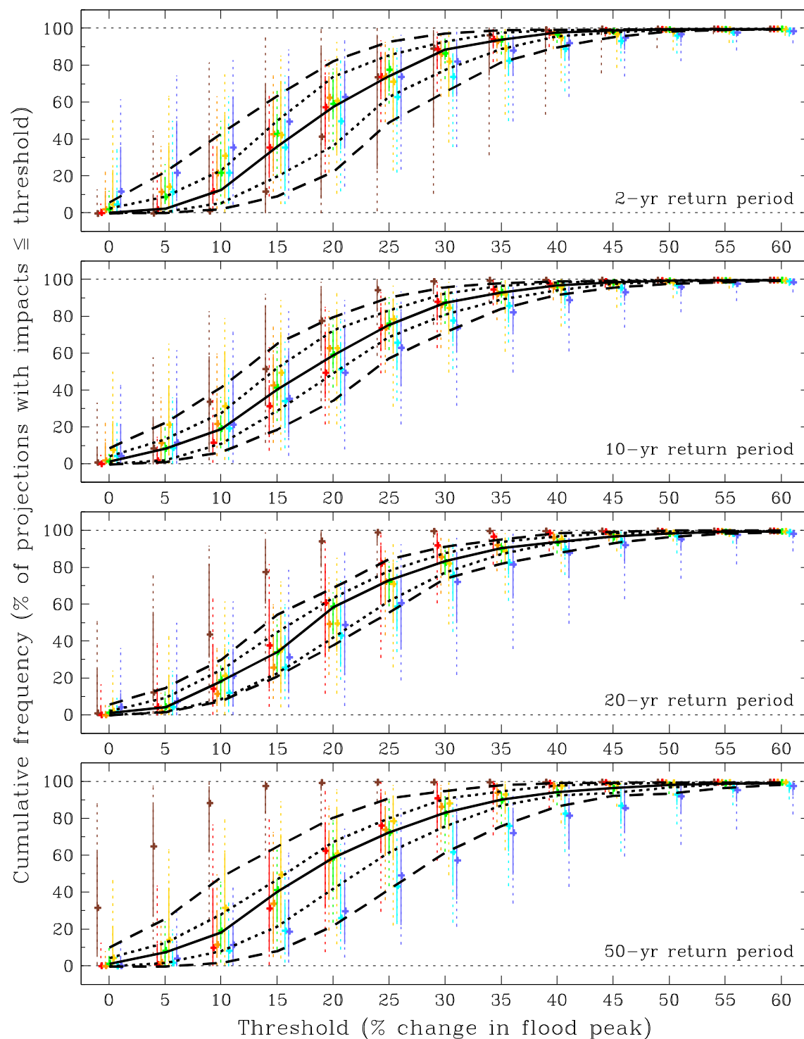
Figure B.26 As Figure B.21 but for the Solway river-basin region (2080s Low).
