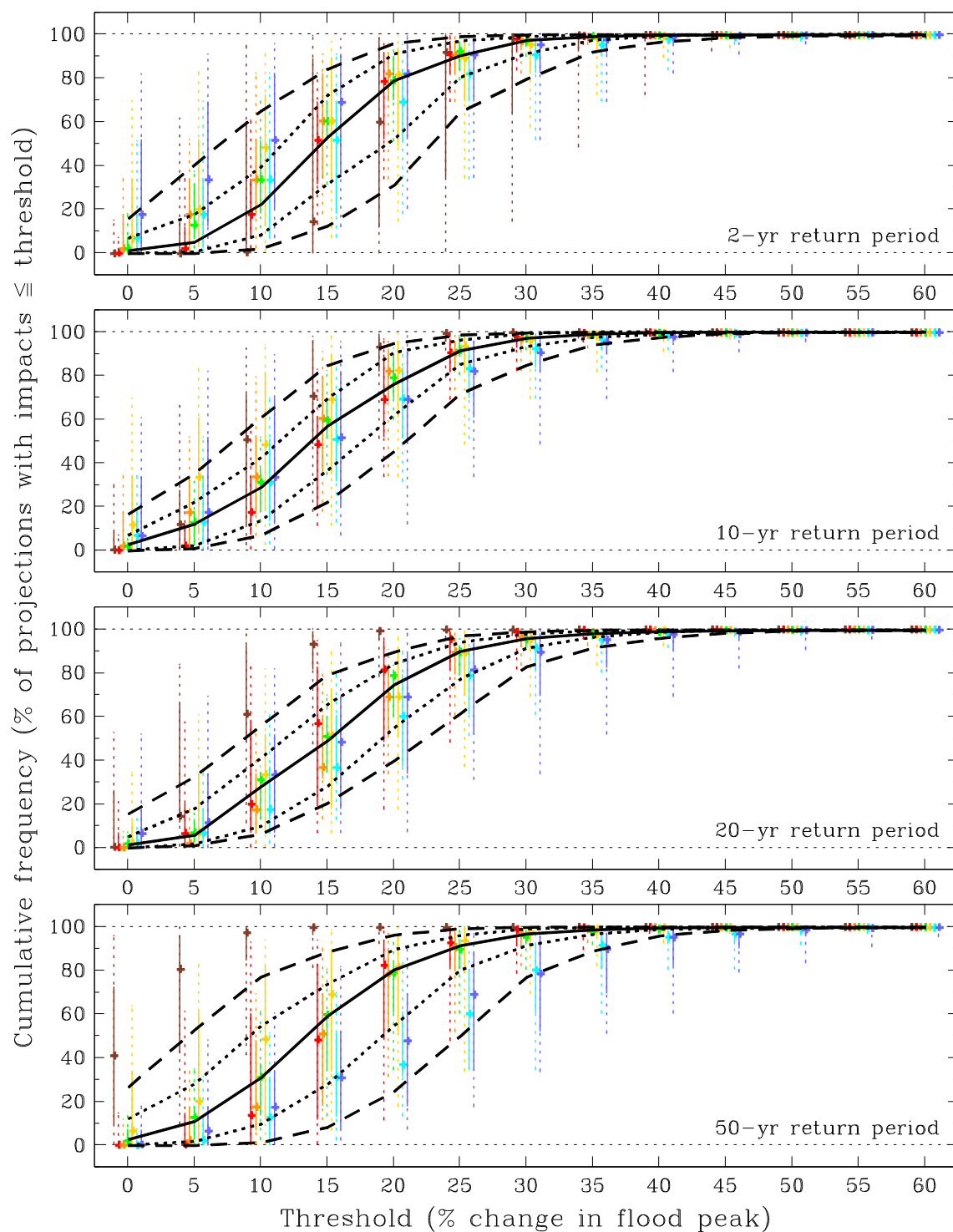
Figure B.15 As Figure B.11 but for the Tweed river-basin region (2050s Medium).
