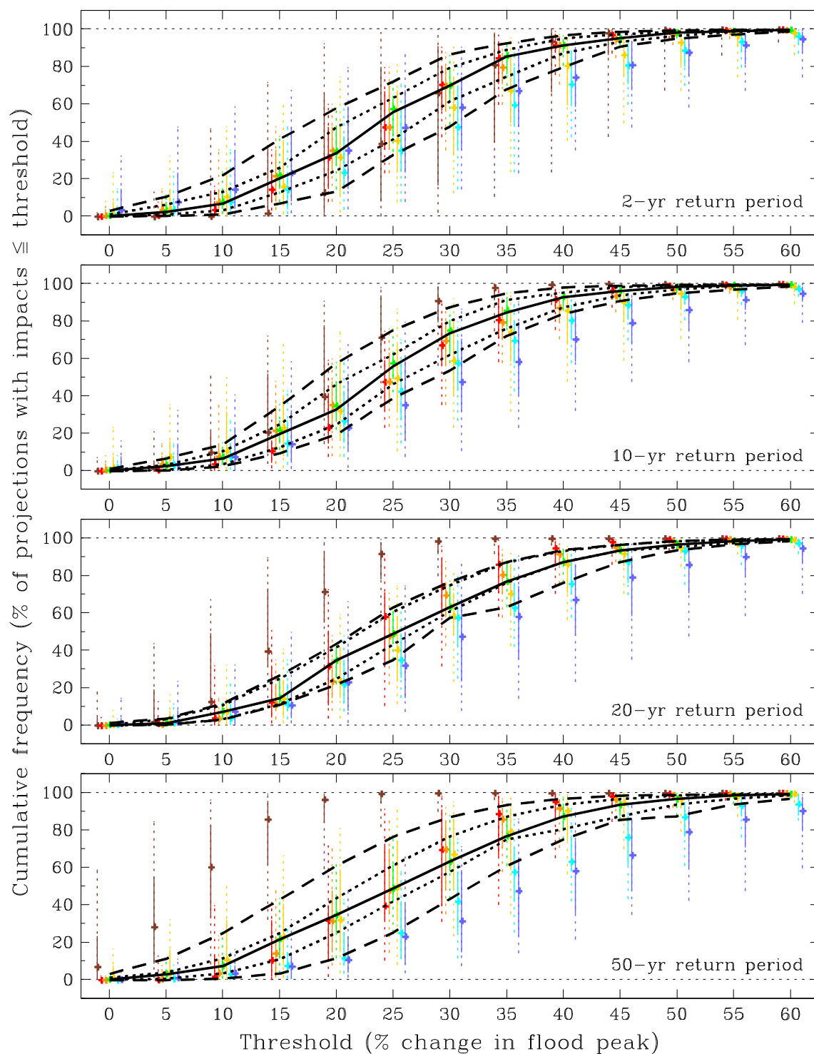
Figure B.19 As Figure B.11 but for the West Highland river-basin region (2050s Medium).
