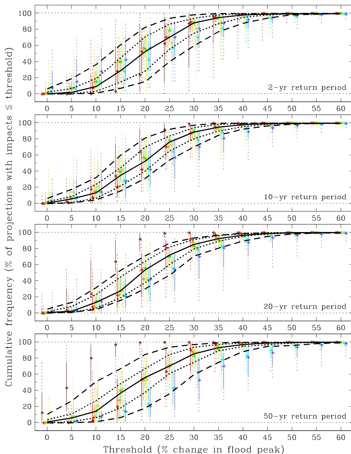
Figure B.21 Summary of the impacts obtained from each of the key response patterns using the UKCP09 Sampled Data (2080s Low) for the North Highland river-basin region. Response-type risk (colours): Damped-High (red), Damped-Low (orange), Neutral (green), Mixed (gold), Enhanced-Low (cyan), Enhanced-Medium (blue), Enhanced-High (purple), Sensitive (magenta); central-estimate (plus sign), \pm 1\text{sd} (solid vertical line), \pm 2\text{sd} (dotted vertical line). Regional risk (black): central-estimate (solid curve), \pm 1\text{sd} (dotted curves), \pm 2\text{sd} (dashed curves).
