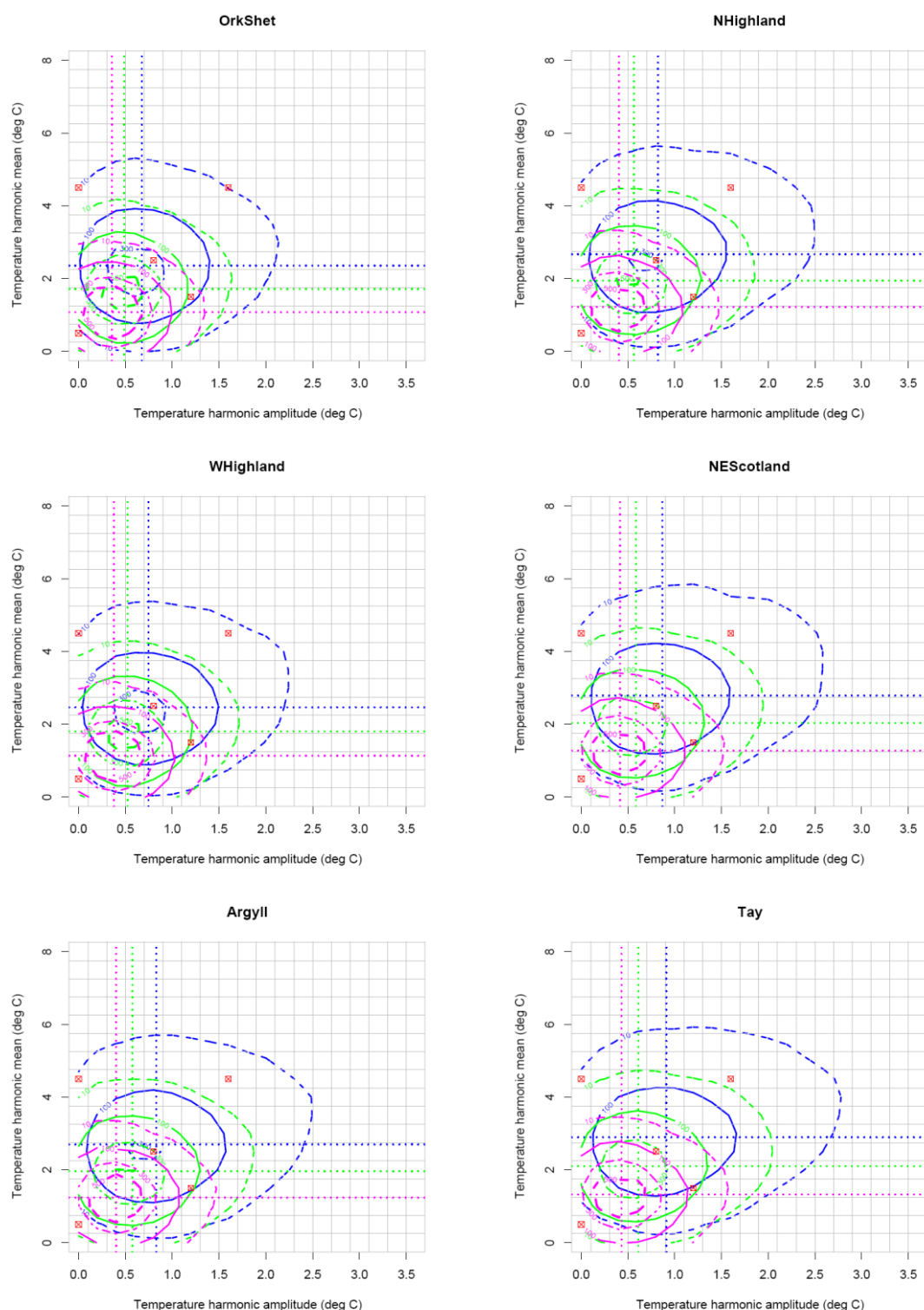
Figure A.12 Contours plots of the mean versus the amplitude of the harmonic functions fitted to the UKCP09 temperature Sampled Data (Medium emissions: 2020s – magenta, 2050s – green, 2080s – blue), for each of the 10 river-basin regions in Scotland. The median of each harmonic parameter is shown by the dotted horizontal/vertical lines. The temperature scenarios of the FD2020 sensitivity framework (Table 1.1) are shown by the red boxes. The contours mark densities of 10, 100, 300 and 500 scenarios per grid square, where required. Figure continued on next page.
