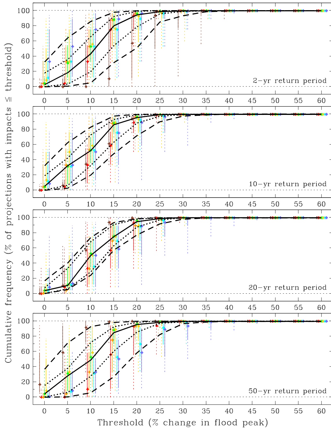
Figure B.3 As Figure B.1 but for the Tay river-basin region (2020s Medium).
