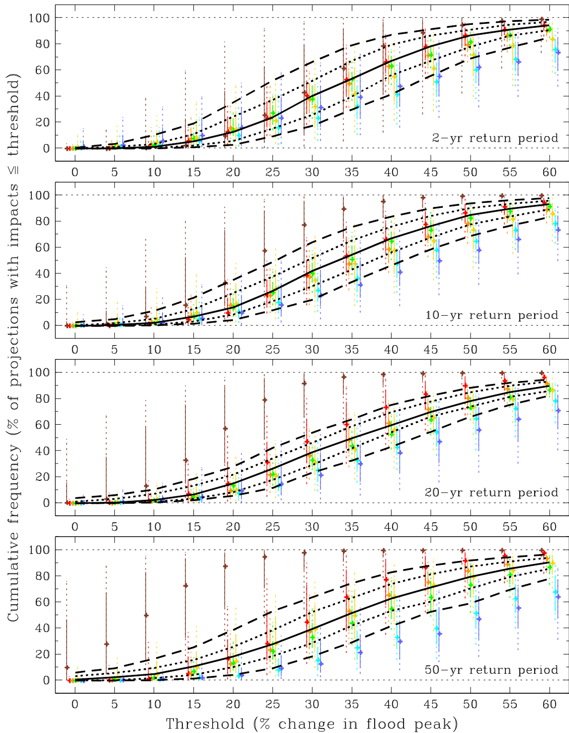
Figure B.37 As Figure B.31 but for the Clyde river-basin region (2080s High).
