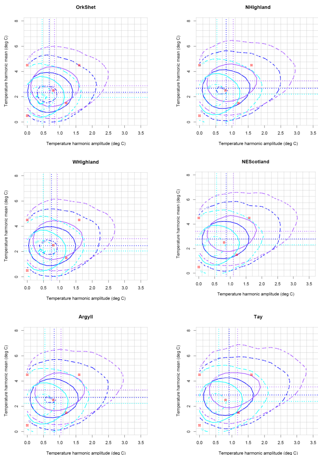
Figure A.16 Contours plots of the mean versus the amplitude of the harmonic functions fitted to the UKCP09 temperature Sampled Data (2080s: Low emissions – cyan, Medium emissions – blue, High emissions – purple), for each of the 10 river-basin regions in Scotland. The median of each harmonic parameter is shown by the dotted horizontal/vertical lines. The temperature scenarios of the FD2020 sensitivity framework (Table 1.1) are shown by the red boxes. The contours mark densities of 10, 100, 300 and 500 scenarios per grid square, where required. Figure continued on next page.
