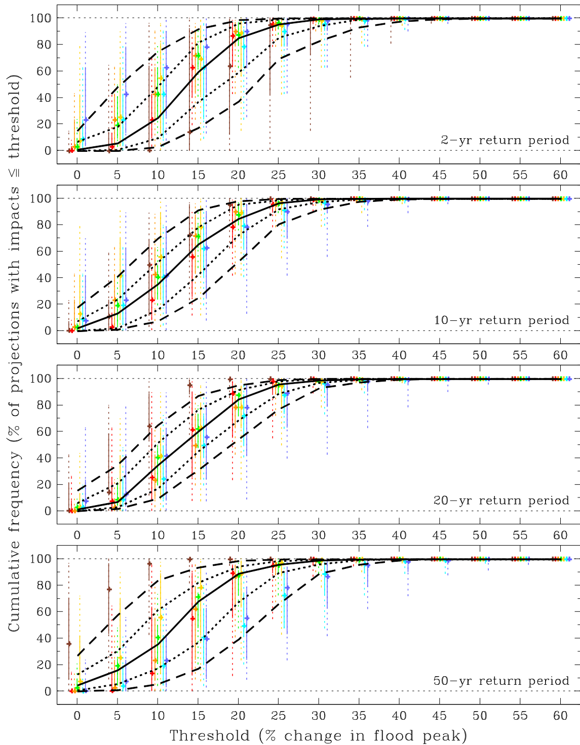
Figure B.12 As Figure B.11 but for the North-East Scotland river-basin region (2050s Medium).
