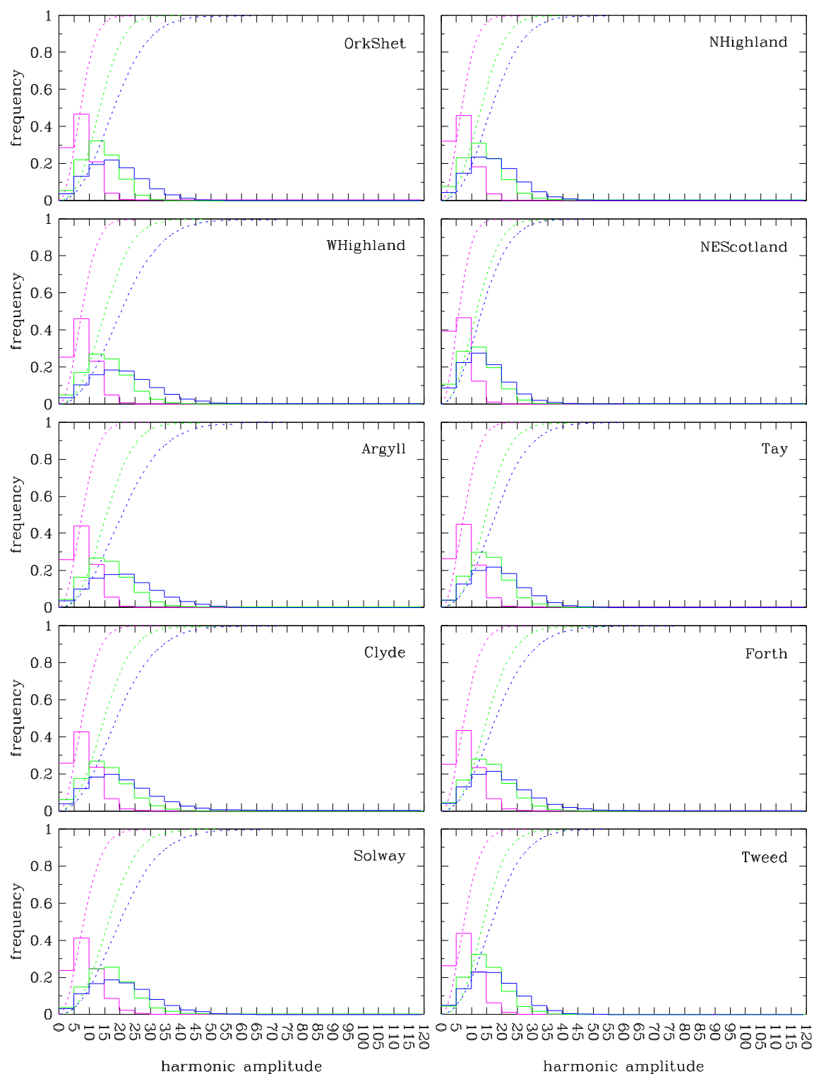
Figure A.2 Histograms and cdfs of the amplitudes of the harmonic functions fitted to the UKCP09 precipitation Sampled Data (Medium emissions: 2020s – magenta, 2050s – green, 2080s – blue), for each of the 10 river-basin regions in Scotland.
