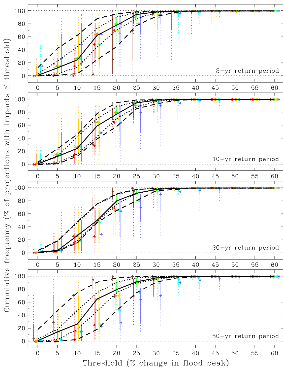
Figure B.9 As Figure B.1 but for the West Highland river-basin region (2020s Medium).
