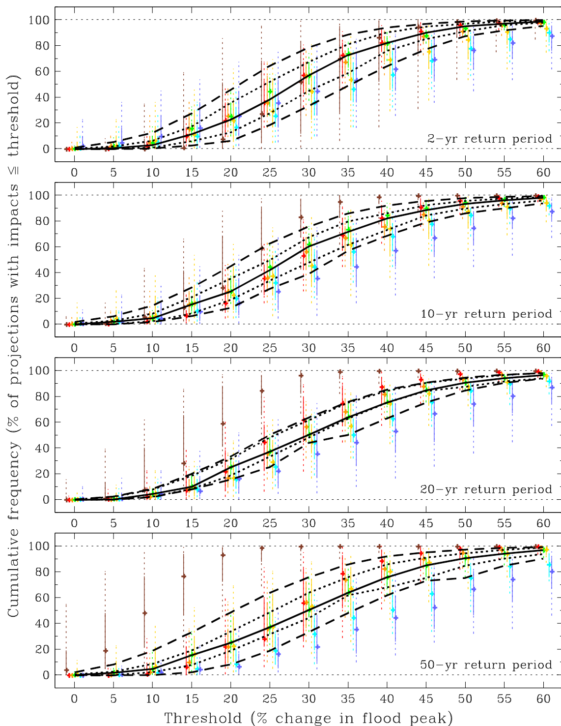
Figure B.28 As Figure B.21 but for the Argyll river-basin region (2080s Low).
