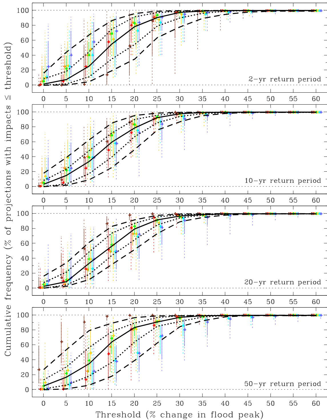
Figure B.22 As Figure B.21 but for the North-East Scotland river-basin region (2080s Low).
