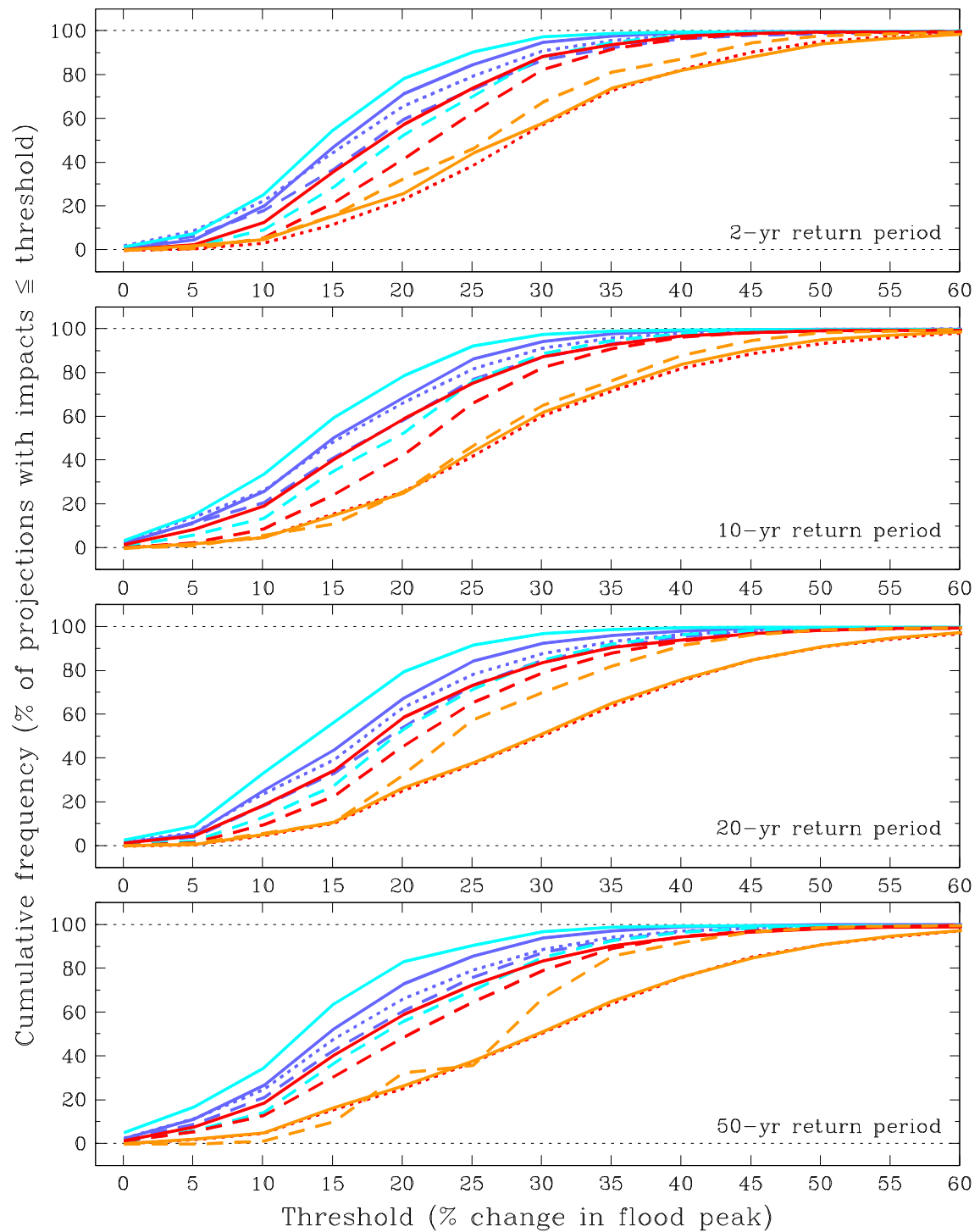
Figure B.43 As Figure B.41 but for the 2080s time-horizon under the Low emissions scenario.
