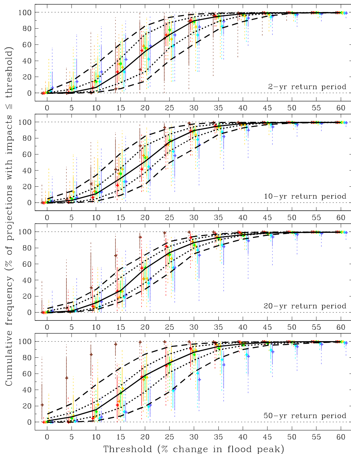
Figure B.17 As Figure B.11 but for the Clyde river-basin region (2050s Medium).
