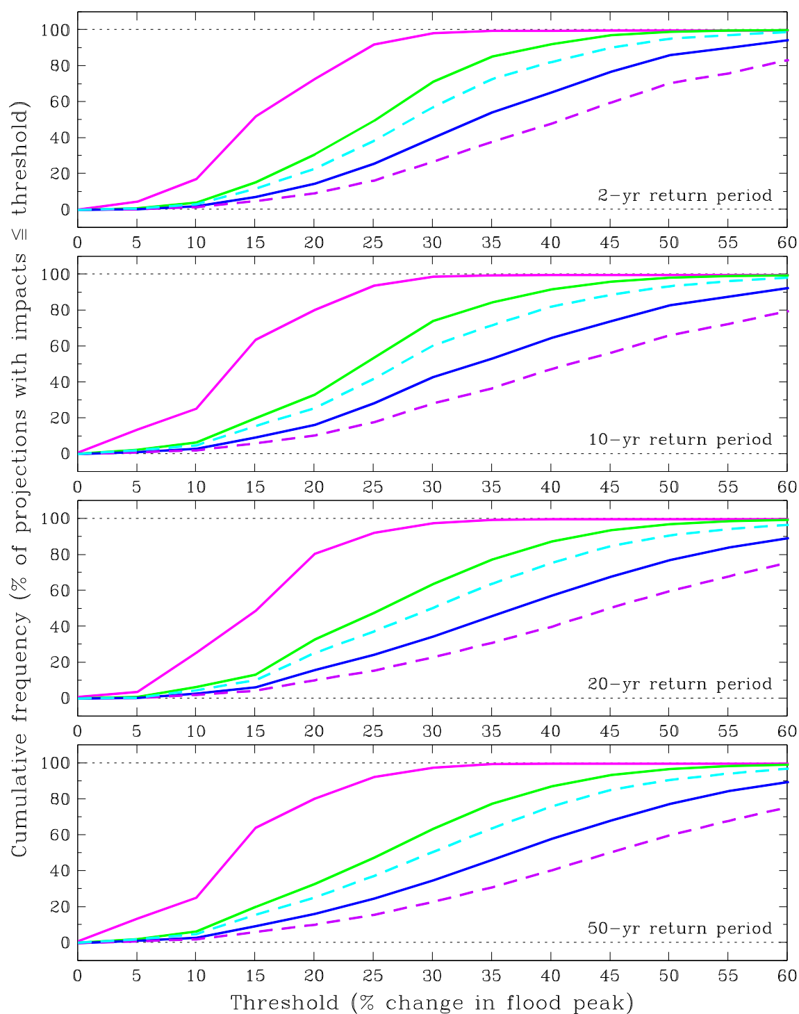
Figure B.52 As Figure B.45 but for the Argyll river-basin region.
