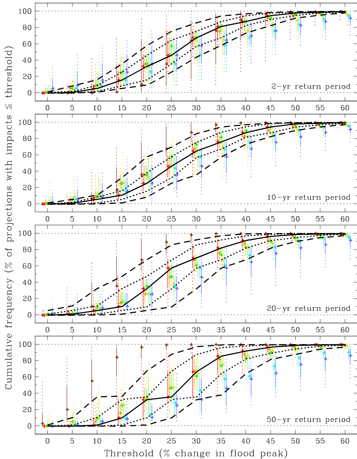
Figure B.30 As Figure B.21 but for the Orkney and Shetland river-basin region (2080s Low).
