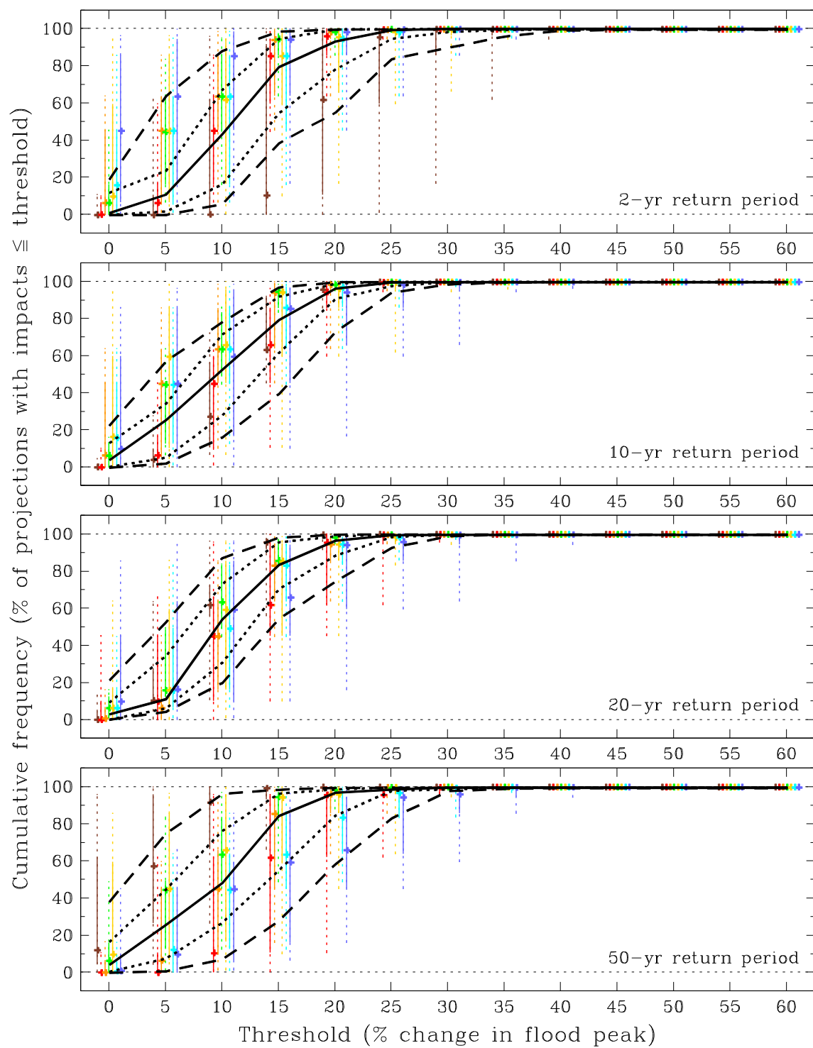
Figure B.2 As Figure B.1 but for the North-East Scotland river-basin region (2020s Medium).
