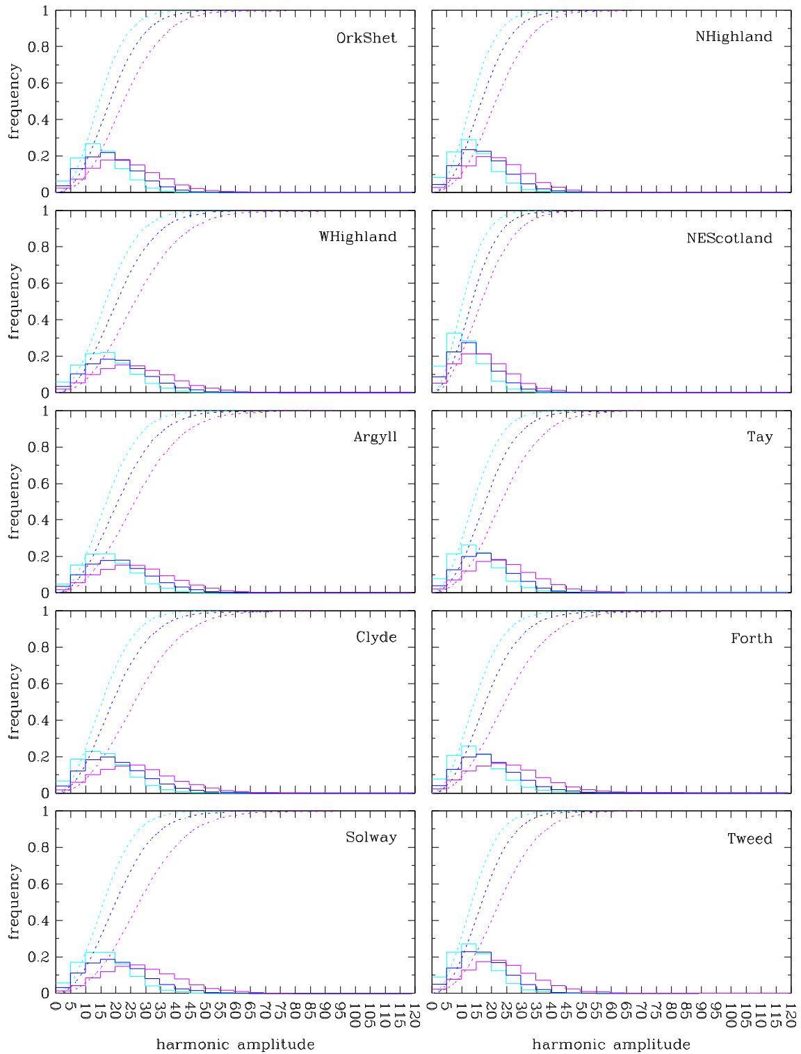
Figure A.6 Histograms and cdfs of the amplitudes of the harmonic functions fitted to the UKCP09 precipitation Sampled Data (2080s: Low emissions – cyan, Medium emissions – blue, High emissions – purple), for each of the 10 river-basin regions in Scotland.
