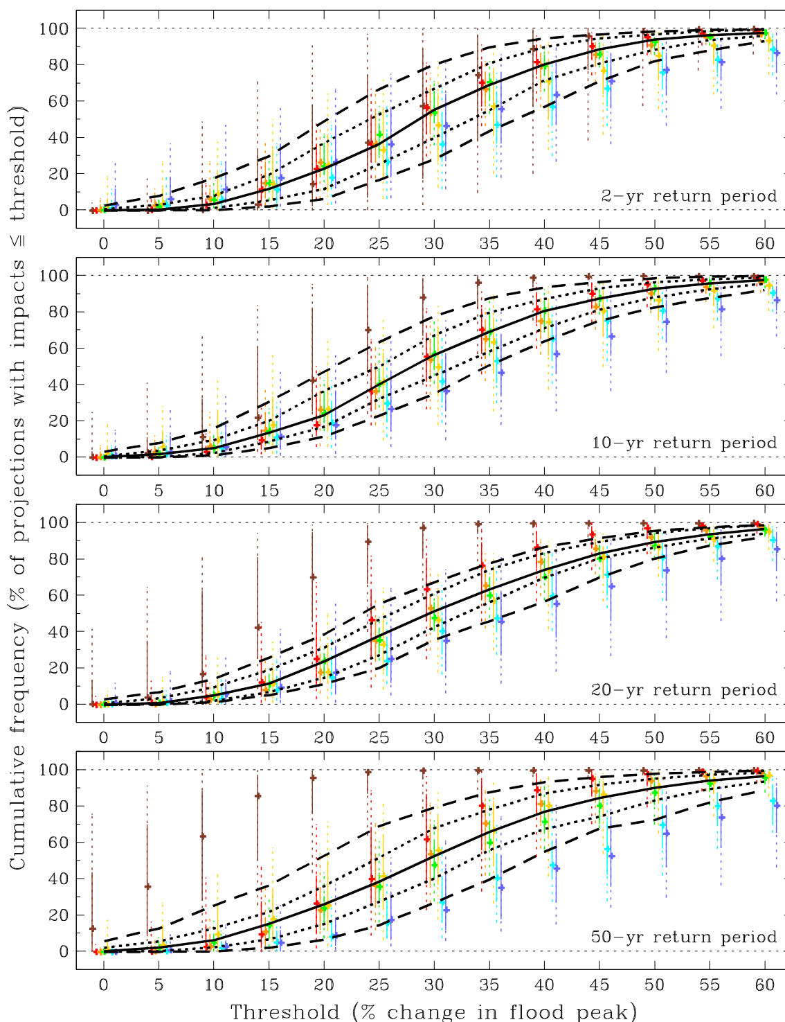
Figure B.31 Summary of the impacts obtained from each of the key response patterns using the UKCP09 Sampled Data (2080s High) for the North Highland river-basin region. Response-type risk (colours): Damped-High (red), Damped-Low (orange), Neutral (green), Mixed (gold), Enhanced-Low (cyan), Enhanced-Medium (blue), Enhanced-High (purple), Sensitive (magenta); central-estimate (plus sign), \pm 1 sd (solid vertical line), \pm 2 sd (dotted vertical line). Regional risk (black): central-estimate (solid curve), \pm 1 sd (dotted curves), \pm 2 sd (dashed curves).
