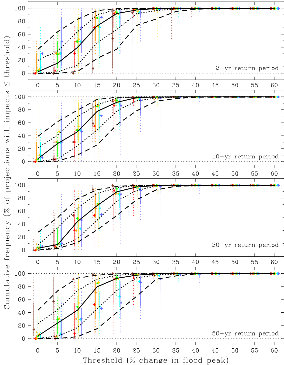
Figure B.4 As Figure B.1 but for the Forth river-basin region (2020s Medium).
