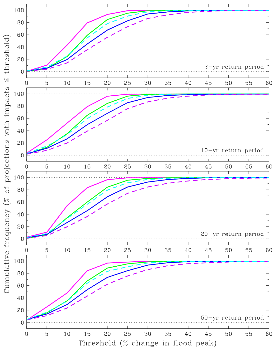
Figure B.46 As Figure B.45 but for the North-East Scotland river-basin region.
