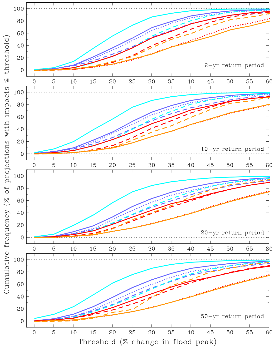
Figure B.44 As Figure B.41 but for the 2080s time-horizon under the High emissions scenario.
