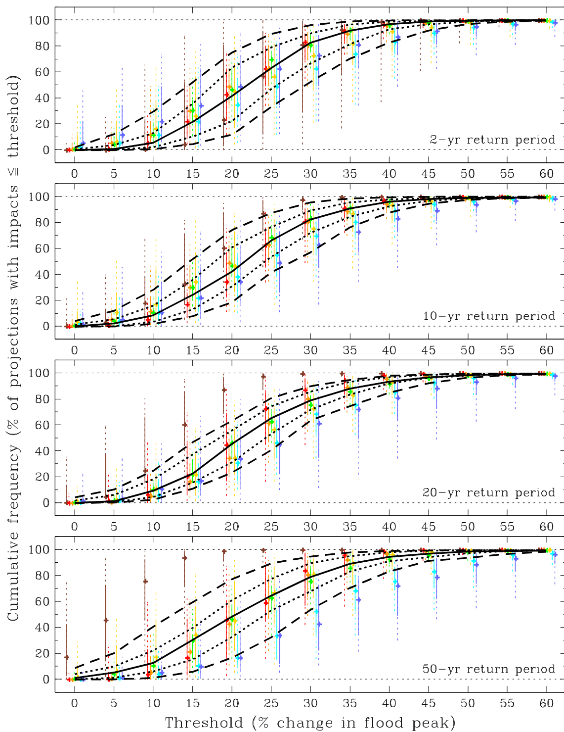
Figure B.27 As Figure B.21 but for the Clyde river-basin region (2080s Low).
