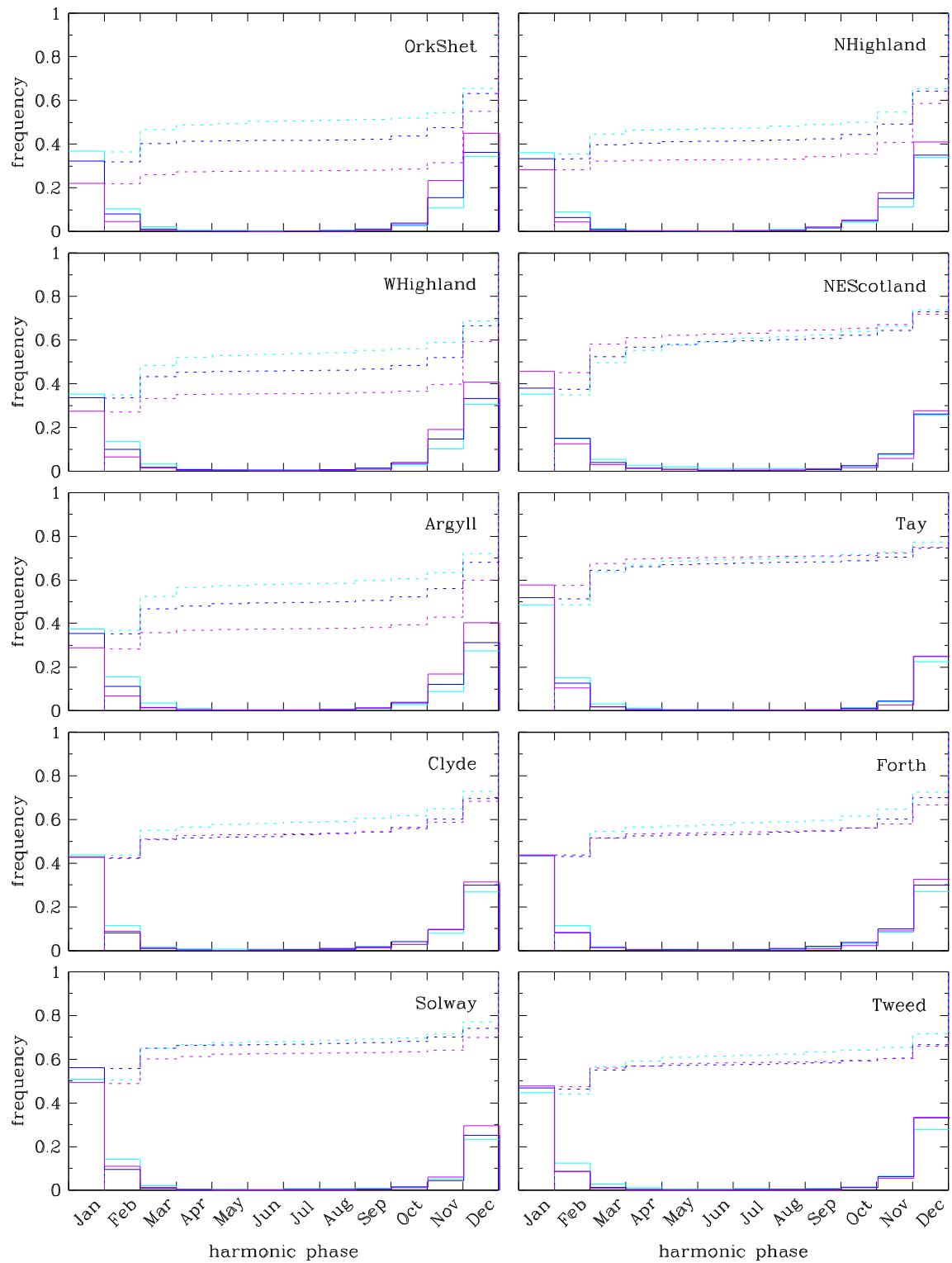
Figure A.7 Histograms and cdfs of the phases of the harmonic functions fitted to the UKCP09 precipitation Sampled Data (2080s: Low emissions – cyan, Medium emissions – blue, High emissions – purple), for each of the 10 river-basin regions in Scotland.
