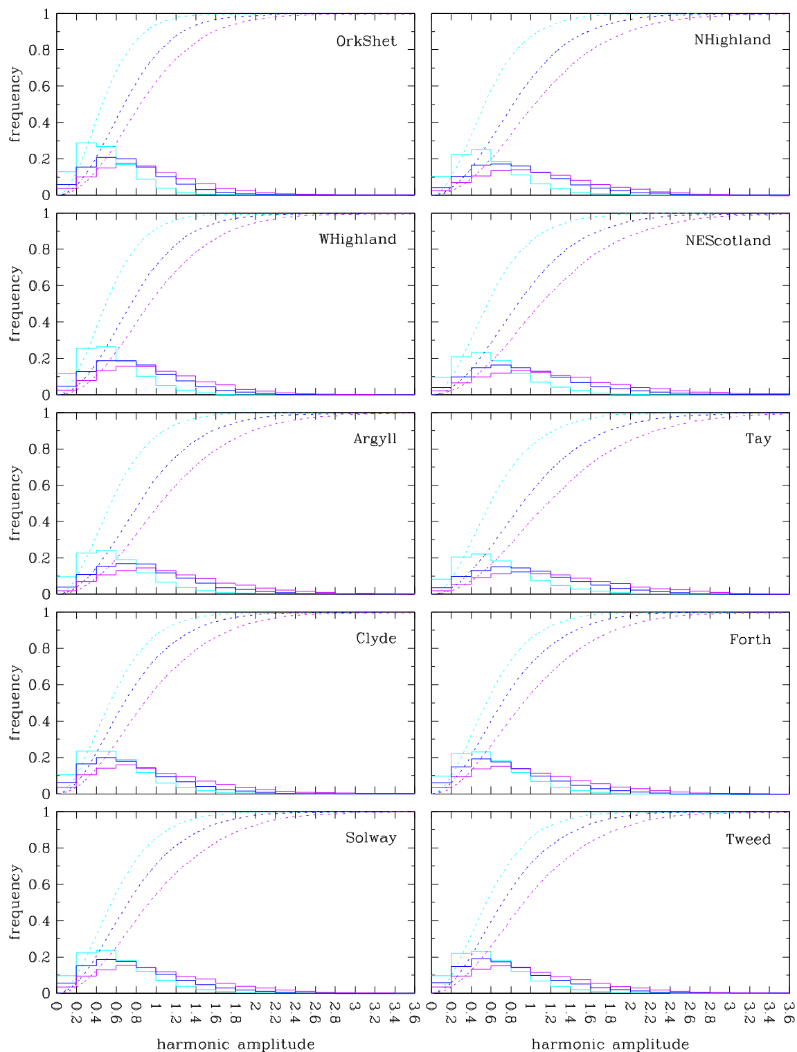
Figure A.14 Histograms and cdfs of the amplitudes of the harmonic functions fitted to the UKCP09 temperature Sampled Data (2080s: Low emissions – cyan, Medium emissions – blue, High emissions – purple), for each of the 10 river-basin regions in Scotland.
