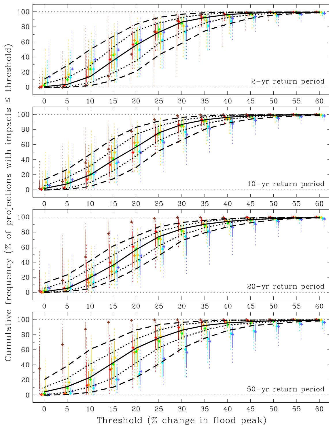
Figure B.32 As Figure B.31 but for the North-East Scotland river-basin region (2080s High).
