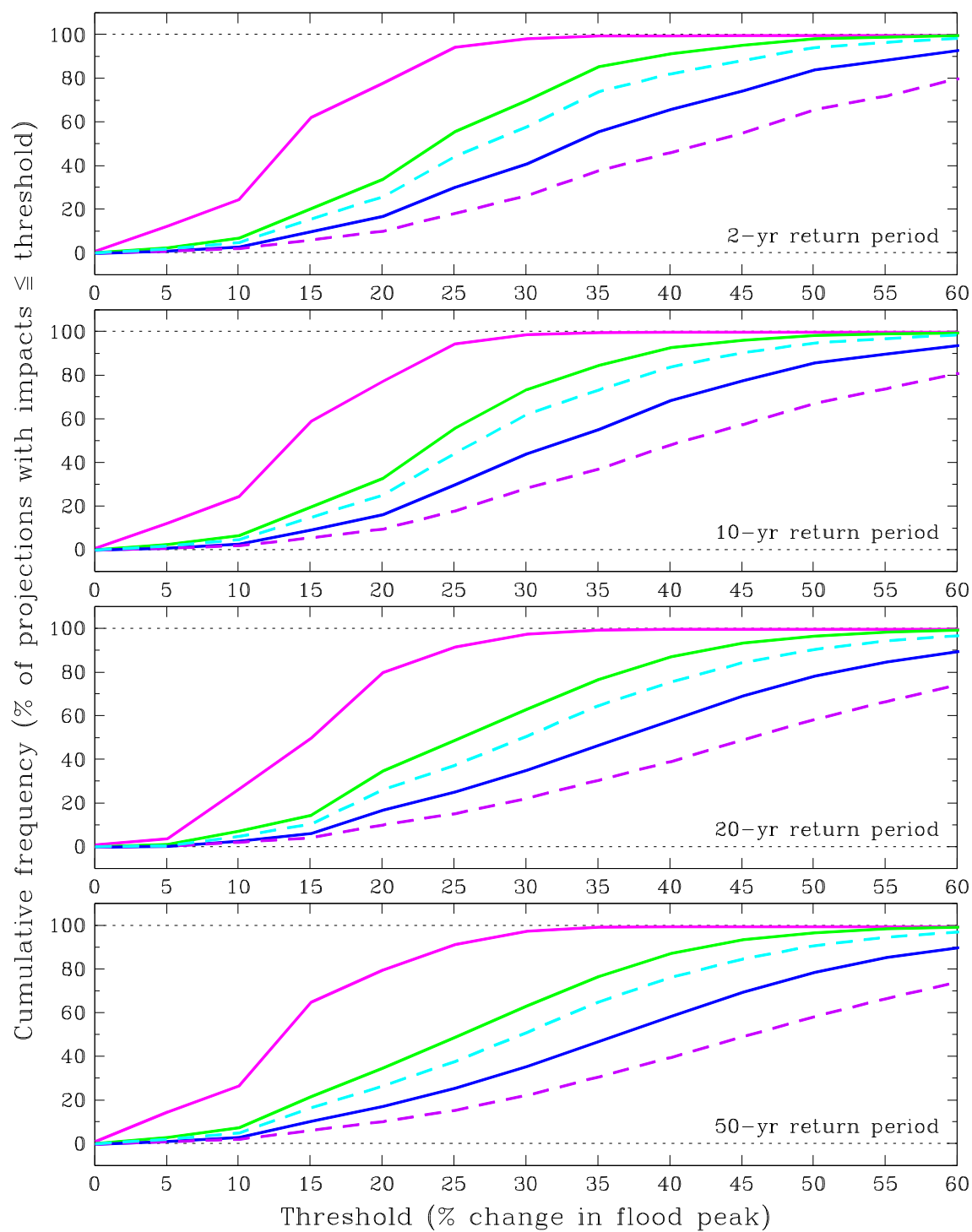
Figure B.53 As Figure B.45 but for the West Highland river-basin region.
