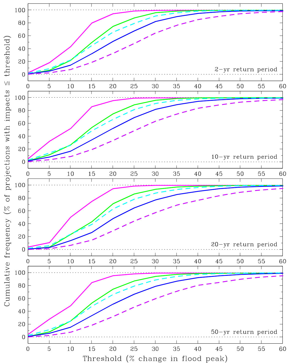
Figure B.47 As Figure B.45 but for the Tay river-basin region.
