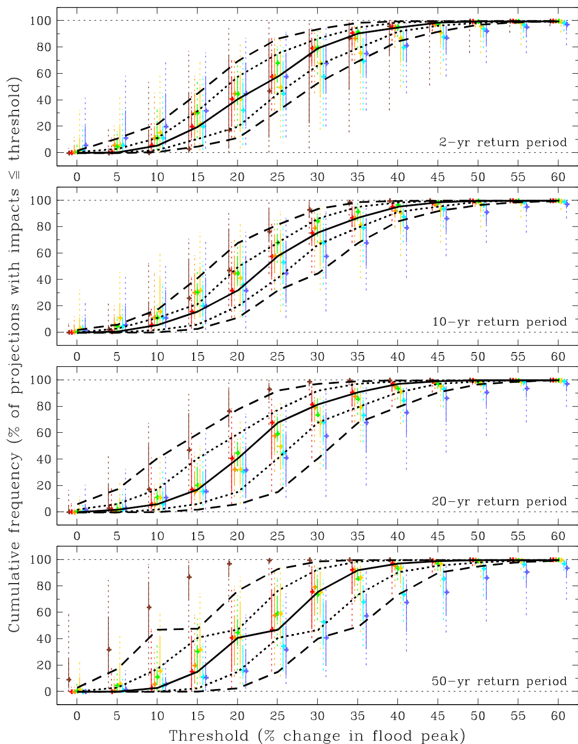
Figure B.20 As Figure B.11 but for the Orkney and Shetland river-basin region (2050s Medium).
