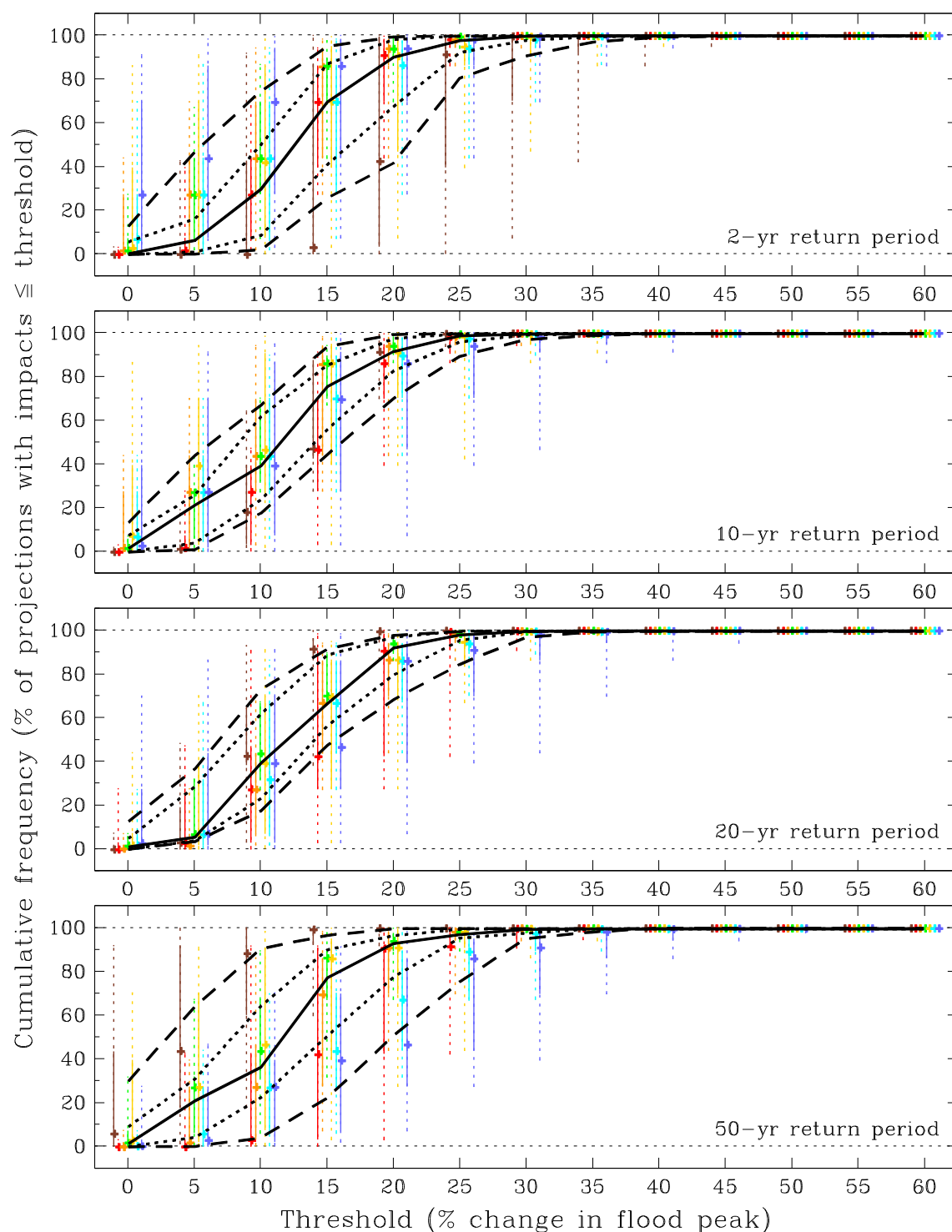
Figure B.1 Summary of the impacts obtained from each of the key response patterns using the UKCP09 Sampled Data (2020s Medium) for the North Highland river-basin region. Response-type risk (colours): Damped-High (red), Damped-Low (orange), Neutral (green), Mixed (gold), Enhanced-Low (cyan), Enhanced-Medium (blue), Enhanced-High (purple), Sensitive (magenta); central-estimate (plus sign), \pm 1\text{sd} (solid vertical line), \pm 2\text{sd} (dotted vertical line). Regional risk (black): central-estimate (solid curve), \pm 1\text{sd} (dotted curves), \pm 2\text{sd} (dashed curves).
