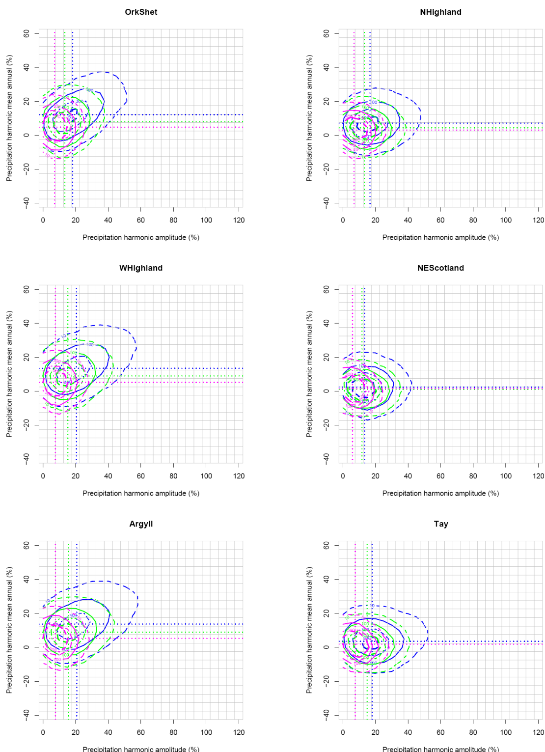
Figure A.4 Contour plots of the mean versus the amplitude of the harmonic functions fitted to the UKCP09 precipitation Sampled Data (Medium emissions: 2020s – magenta, 2050s – green, 2080s – blue), for each of the 10 river-basin regions in Scotland. The median of each harmonic parameter is shown by the dotted horizontal/vertical lines. Note that the grid on these plots is the same as that of the FD2020 sensitivity framework (Table 1.1) and thus of the response patterns and standard deviation patterns (Figure 1.3 and Figure 1.4). The contours mark densities of 10, 100, 300 and 500 scenarios per grid square, where required. Figure continued on next page.
