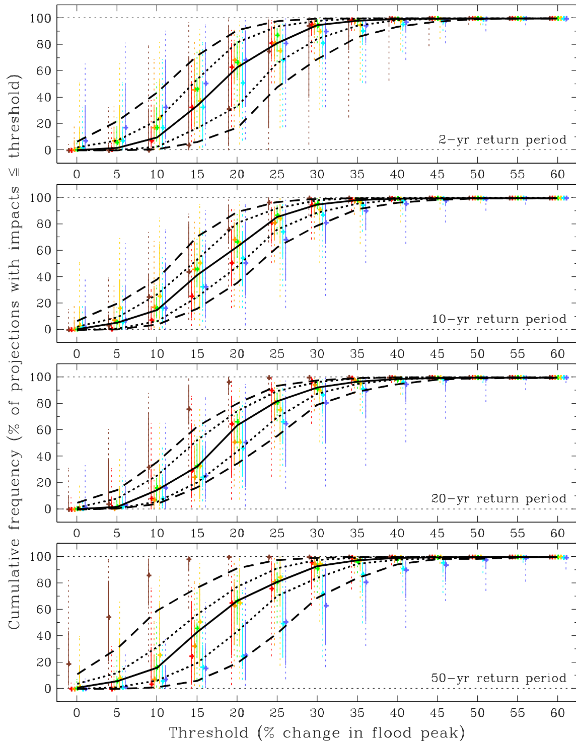
Figure B.11 Summary of the impacts obtained from each of the key response patterns using the UKCP09 Sampled Data (2050s Medium) for the North Highland river-basin region. Response-type risk (colours): Damped-High (red), Damped-Low (orange), Neutral (green), Mixed (gold), Enhanced-Low (cyan), Enhanced-Medium (blue), Enhanced-High (purple), Sensitive (magenta); central-estimate (plus sign), \pm 1 sd (solid vertical line), \pm 2 sd (dotted vertical line). Regional risk (black): central-estimate (solid curve), \pm 1 sd (dotted curves), \pm 2 sd (dashed curves).
