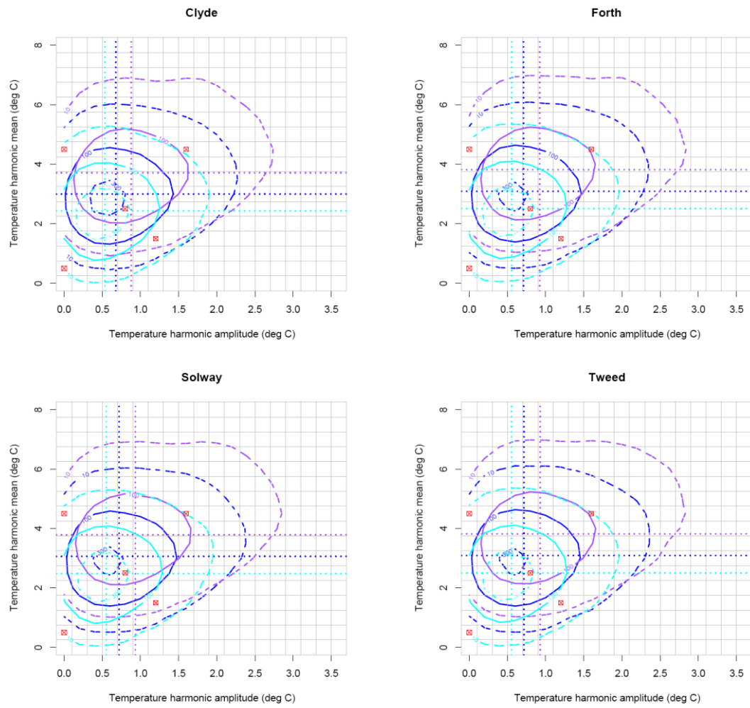
Figure A.16 continued.
