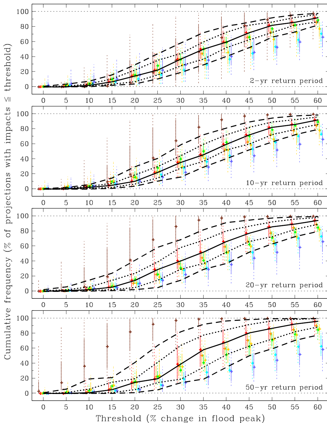
Figure B.40 As Figure B.31 but for the Orkney and Shetland river-basin region (2080s High).
