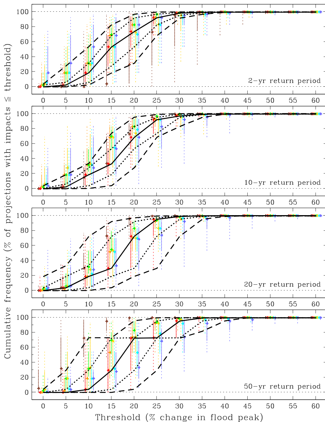
Figure B.10 As Figure B.1 but for the Orkney and Shetland river-basin region (2020s Medium).
