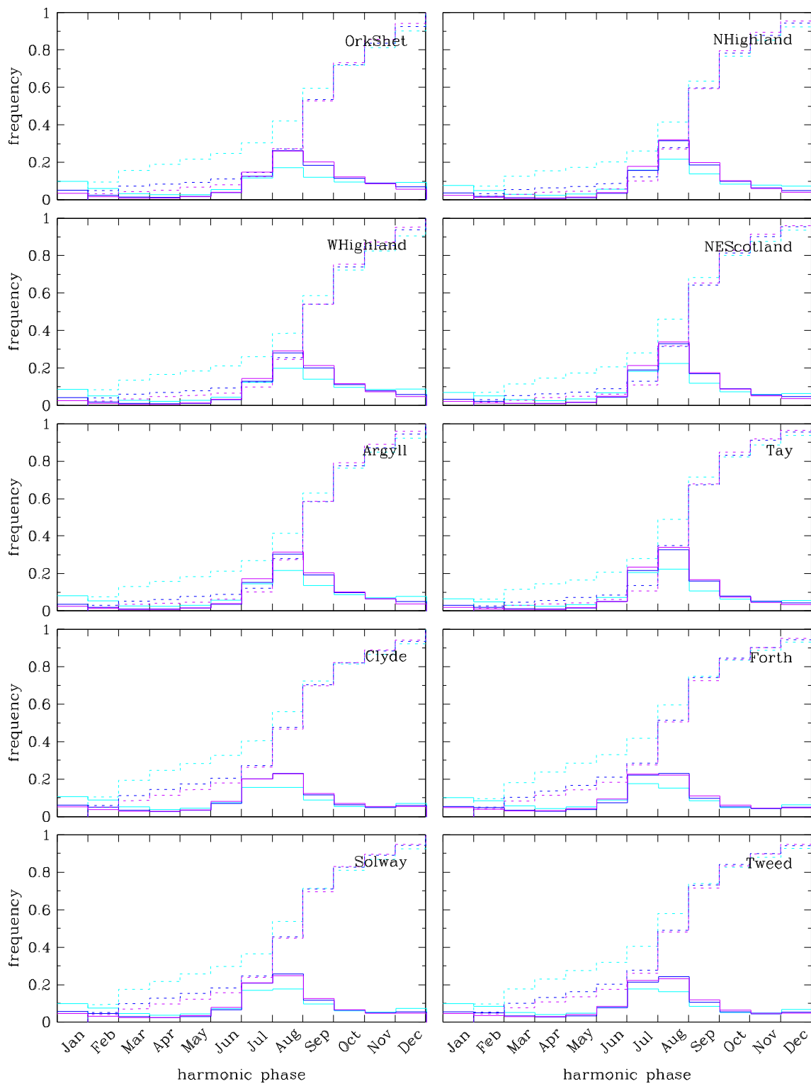
Figure A.15 Histograms and cdfs of the phases of the harmonic functions fitted to the UKCP09 temperature Sampled Data (2080s: Low emissions – cyan, Medium emissions – blue, High emissions – purple), for each of the 10 river-basin regions in Scotland.
