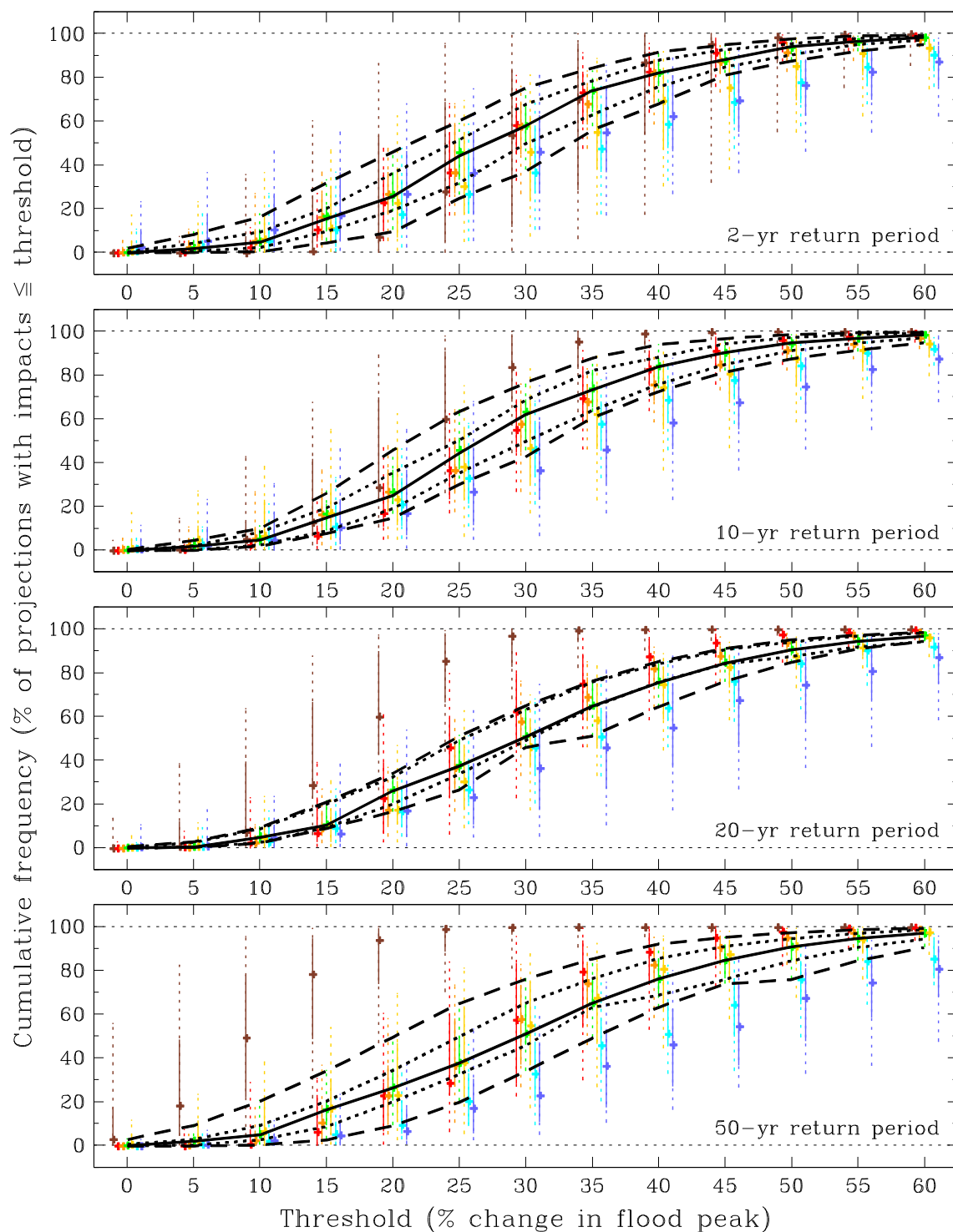
Figure B.29 As Figure B.21 but for the West Highland river-basin region (2080s Low).
