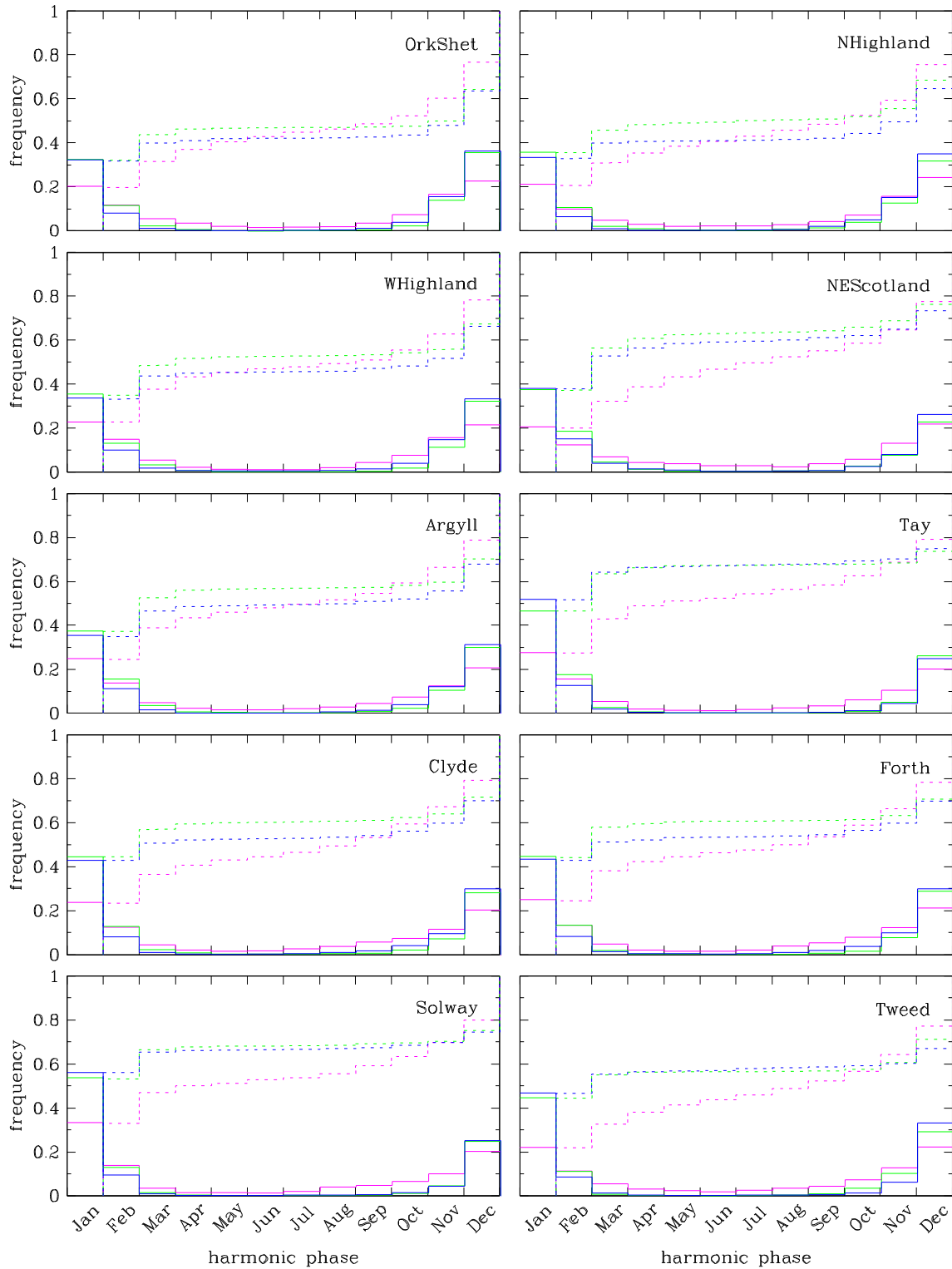
Figure A.3 Histograms and cdfs of the phases of the harmonic functions fitted to the UKCP09 precipitation Sampled Data (Medium emissions: 2020s – magenta, 2050s – green, 2080s – blue), for each of the 10 river-basin regions in Scotland.
