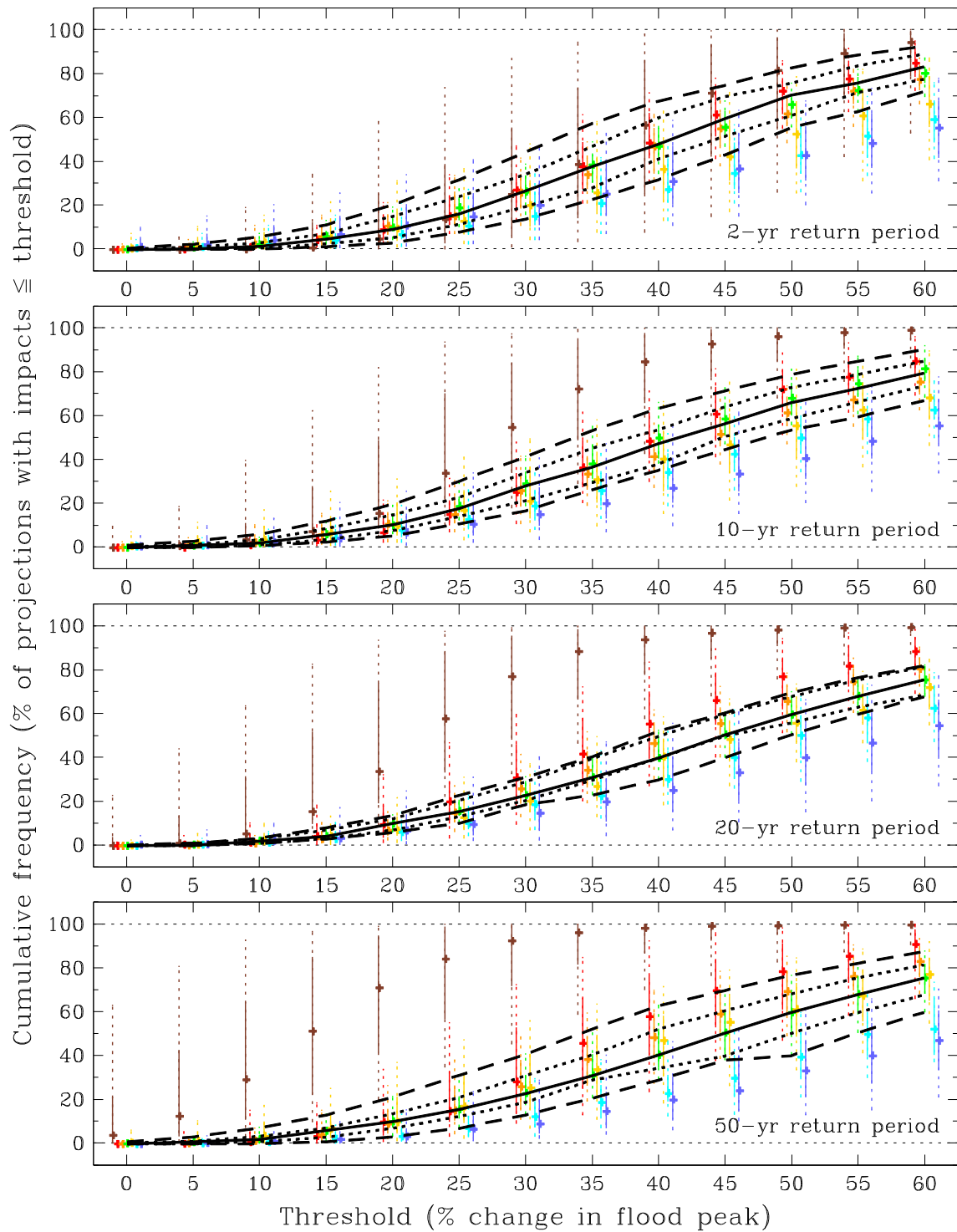
Figure B.38 As Figure B.31 but for the Argyll river-basin region (2080s High).
