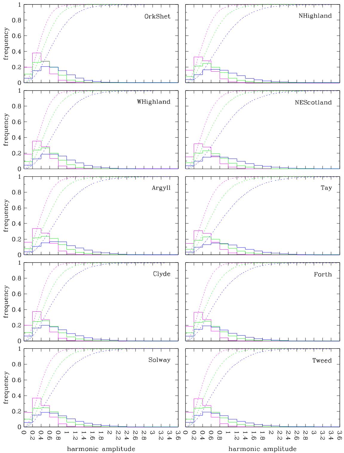
Figure A.10 Histograms and cdfs of the amplitudes of the harmonic functions fitted to the UKCP09 temperature Sampled Data (Medium emissions: 2020s – magenta, 2050s – green, 2080s – blue), for each of the 10 river-basin regions in Scotland.
