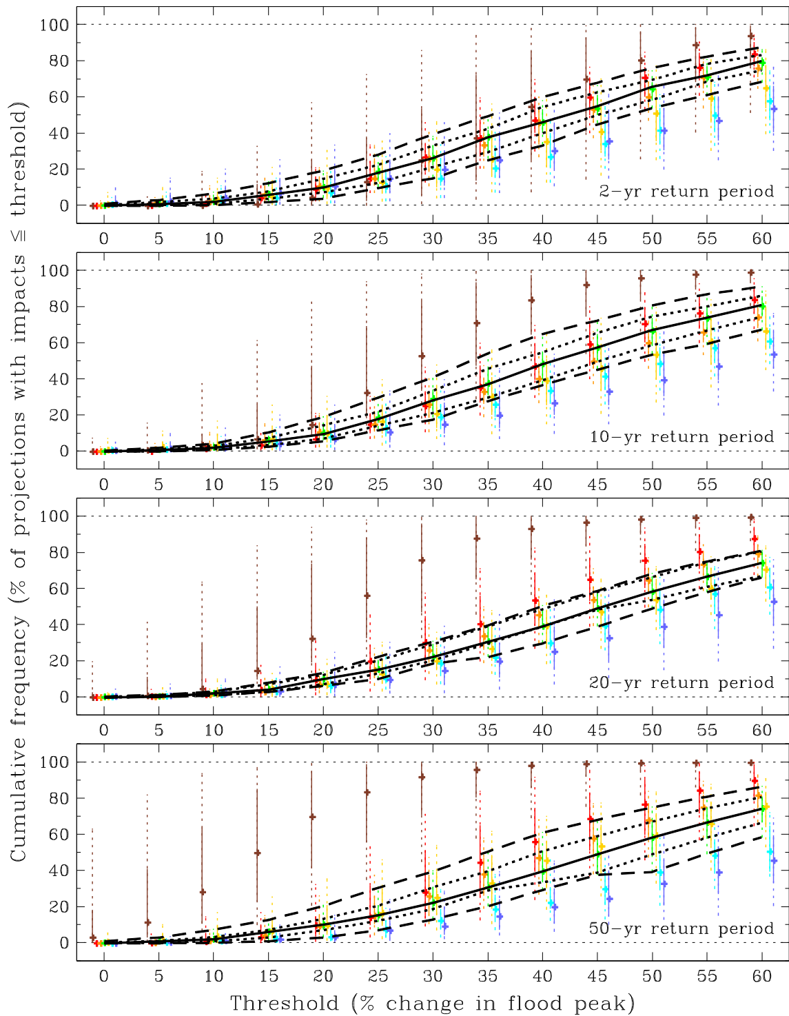
Figure B.39 As Figure B.31 but for the West Highland river-basin region (2080s High).
