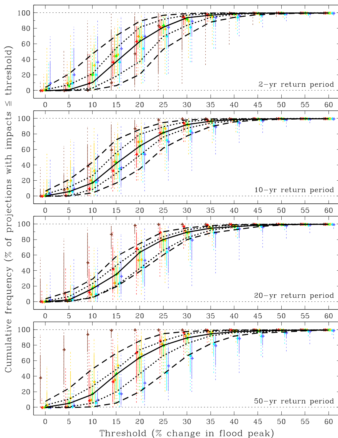
Figure B.16 As Figure B.11 but for the Solway river-basin region (2050s Medium) .
