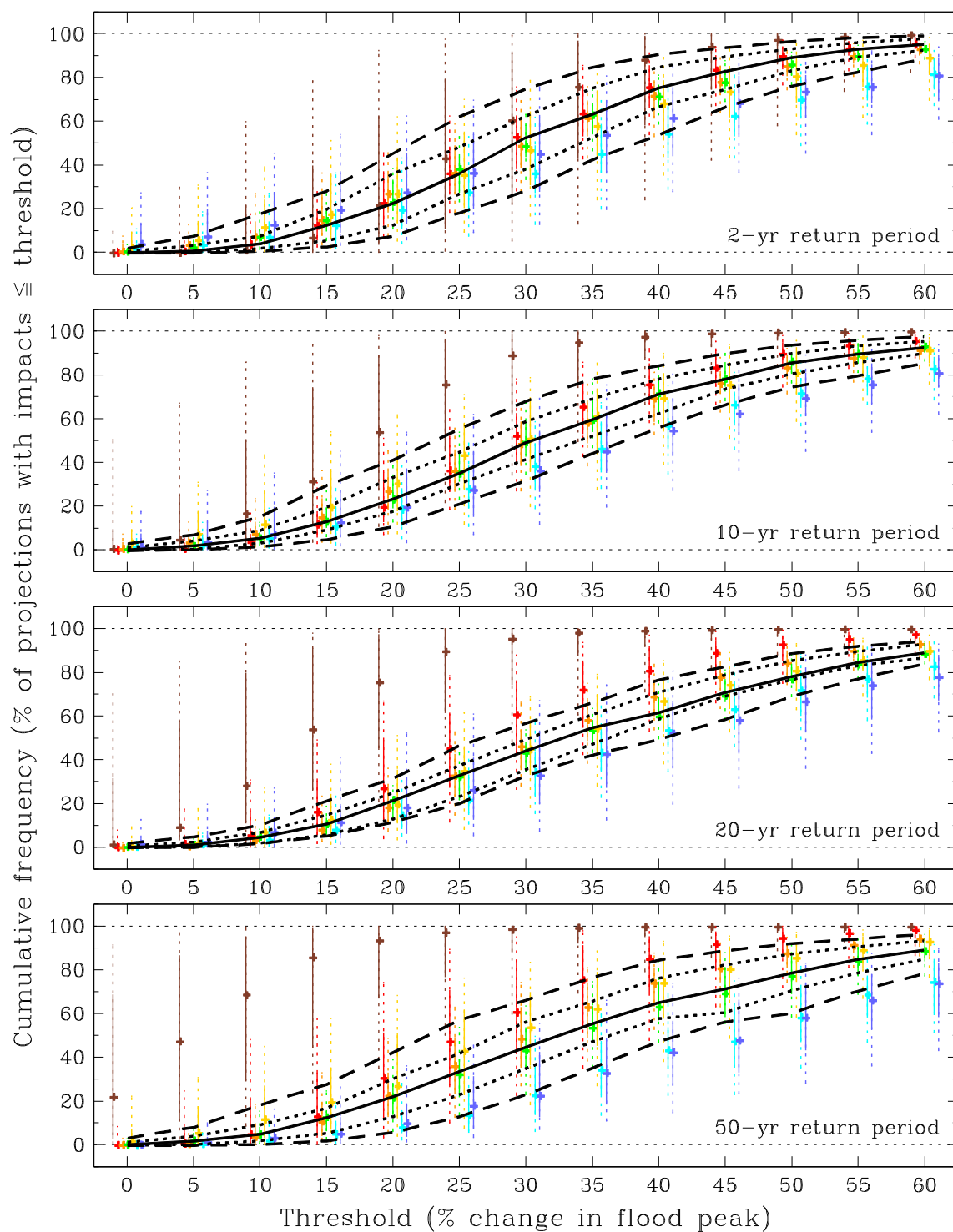
Figure B.36 As Figure B.31 but for the Solway river-basin region (2080s High).
