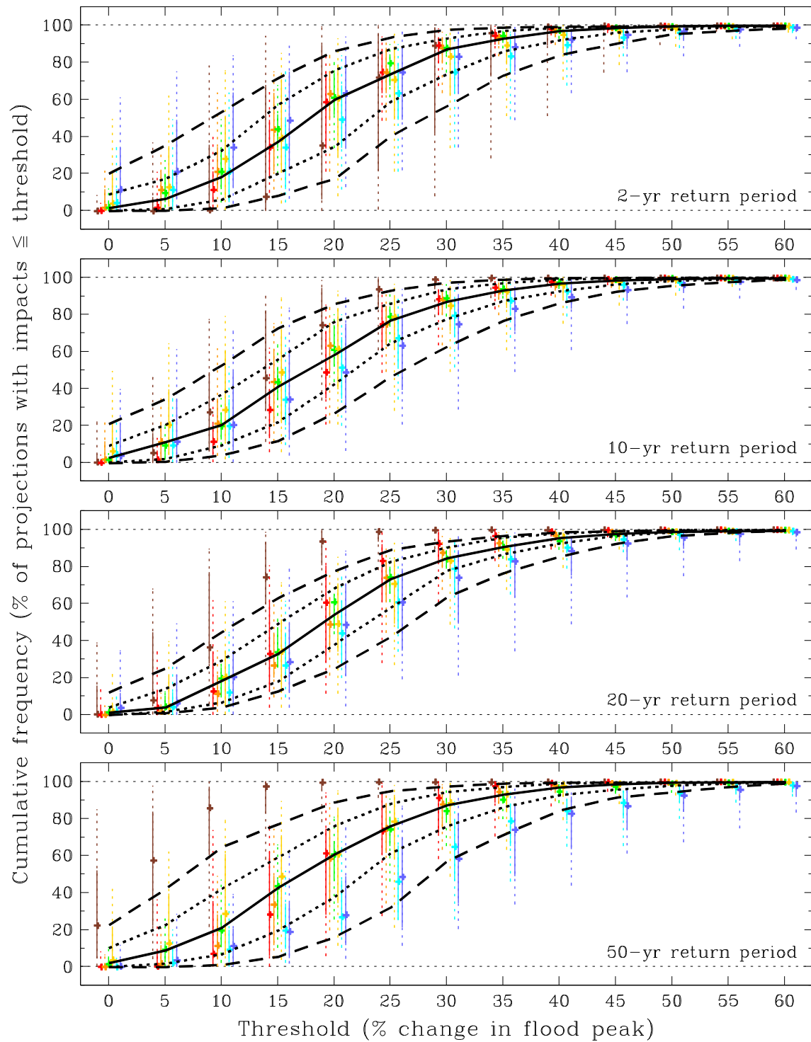
Figure B.24 As Figure B.21 but for the Forth river-basin region (2080s Low).
