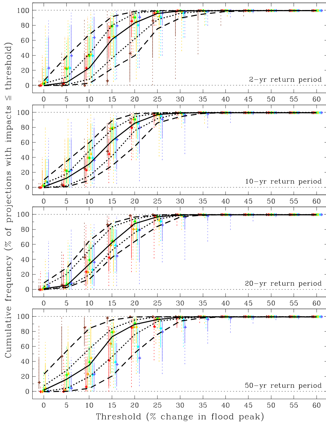
Figure B.7 As Figure B.1 but for the Clyde river-basin region (2020s Medium).
