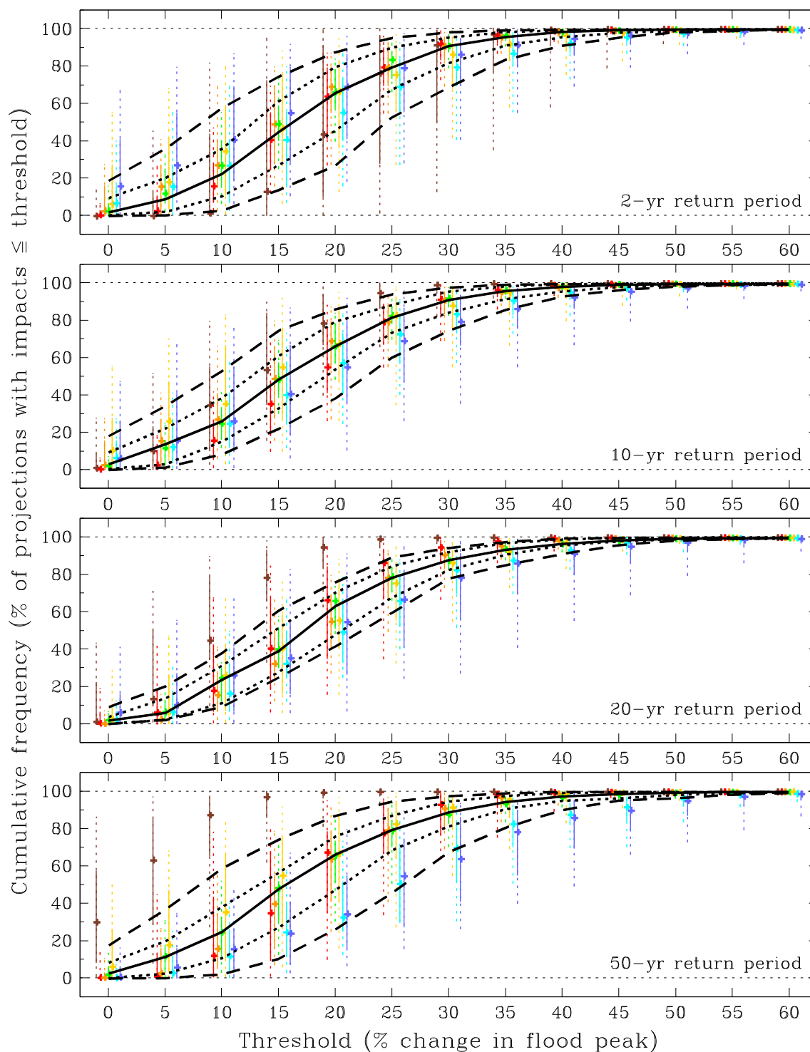
Figure B.23 As Figure B.21 but for the Tay river-basin region (2080s Low).
