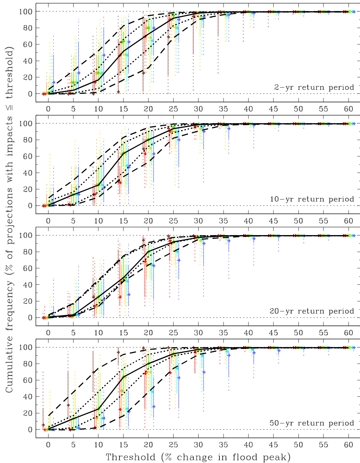
Figure B.8 As Figure B.1 but for the Argyll river-basin region (2020s Medium).
