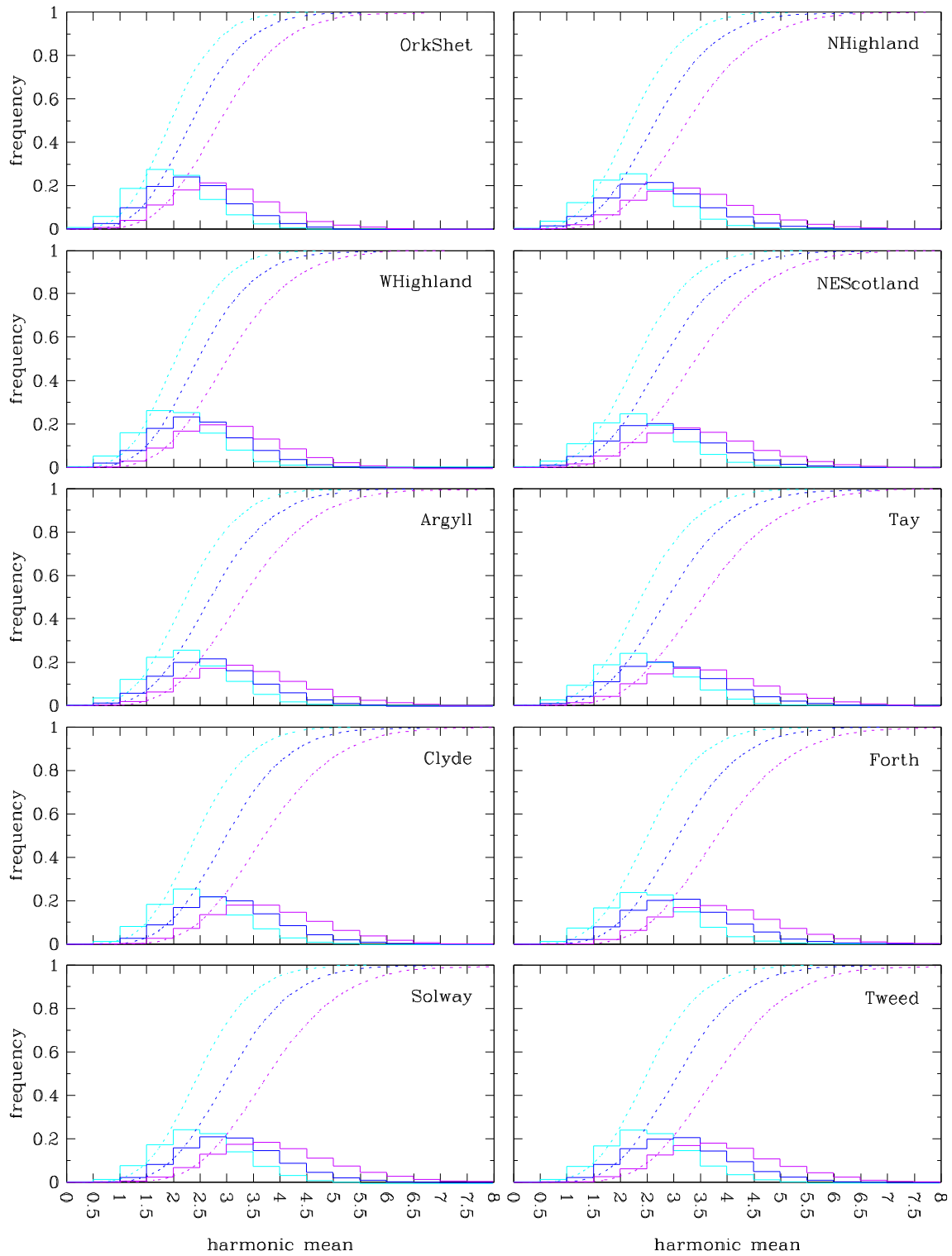
Figure A.13 Histograms and cdfs of the means of the harmonic functions fitted to the UKCP09 temperature Sampled Data (2080s: Low emissions – cyan, Medium emissions – blue, High emissions – purple), for each of the 10 river-basin regions in Scotland.
