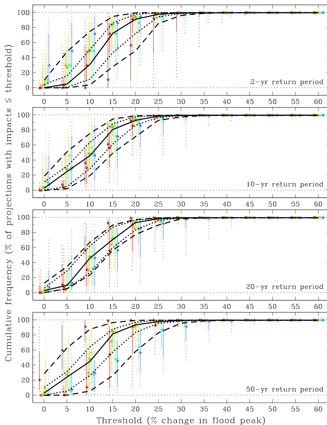
Figure B.6 As Figure B.1 but for the Solway river-basin region (2020s Medium).
