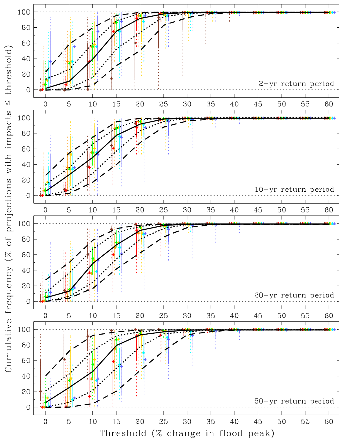
Figure B.5 As Figure B.1 but for the Tweed river-basin region (2020s Medium).
