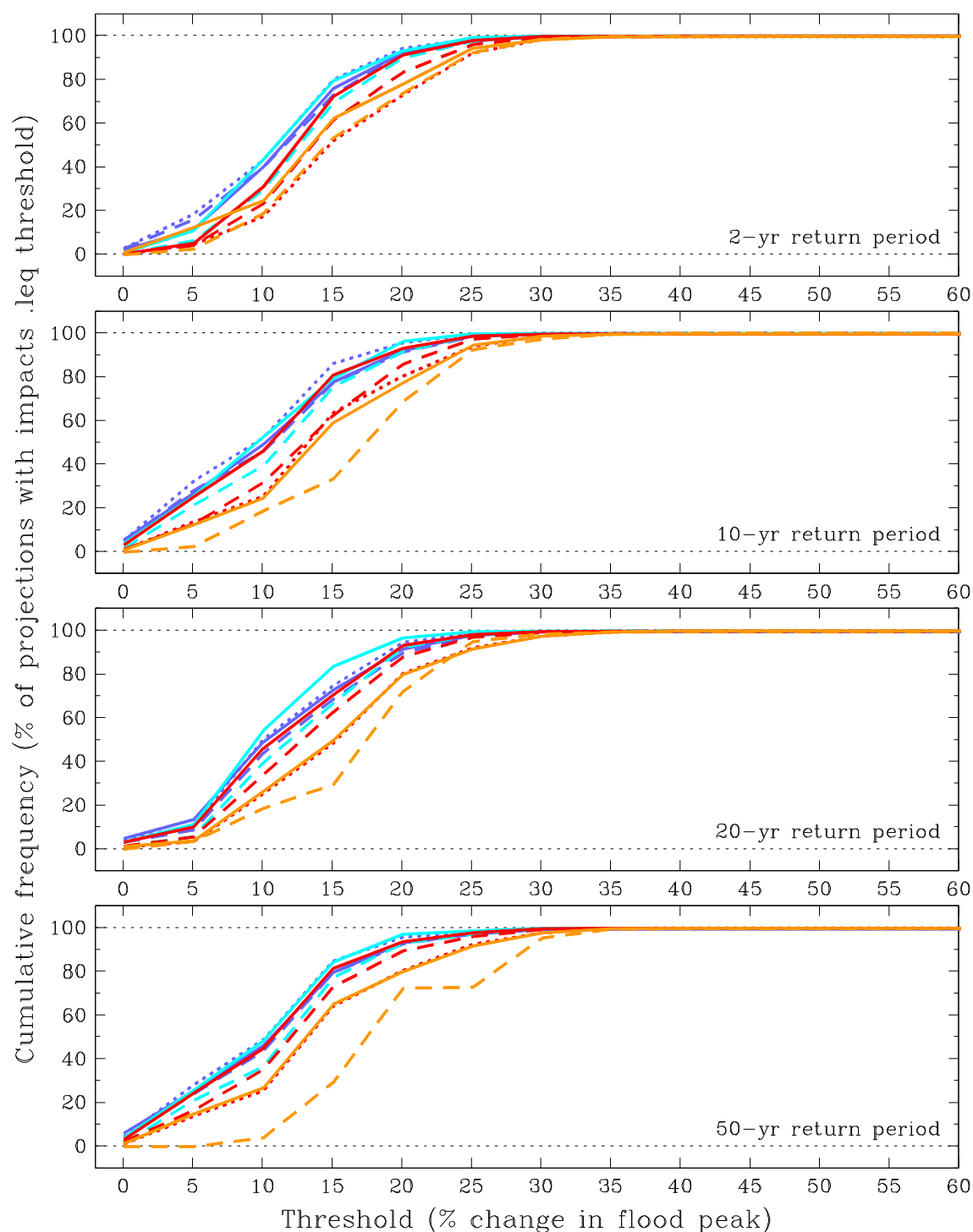
Figure B.41 Regional risk cdfs (central-estimates) for each of the 10 UKCP09 river-basin regions in Scotland, for the 2020s time-horizon under the Medium emissions scenario. Key: North Highland – cyan dashed; North-East Scotland – cyan solid; Tay – blue dotted; Forth – blue dashed; Tweed – blue solid; Orkney and Shetland – orange dashed; West Highland – orange solid; Argyll – red dotted; Clyde – red dashed; Solway – red solid.
