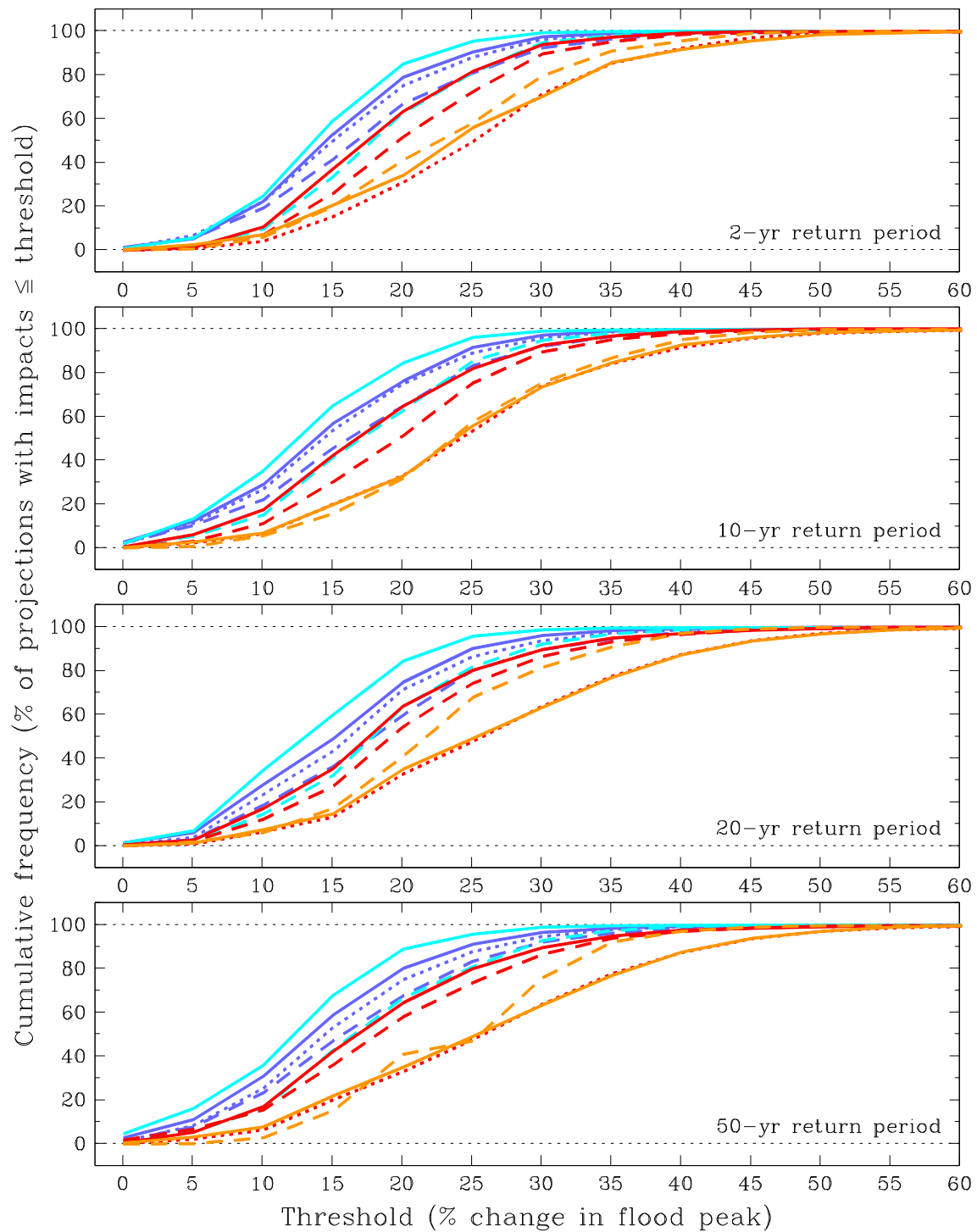
Figure B.42 As Figure B.41 but for the 2050s time-horizon under the Medium emissions scenario.
