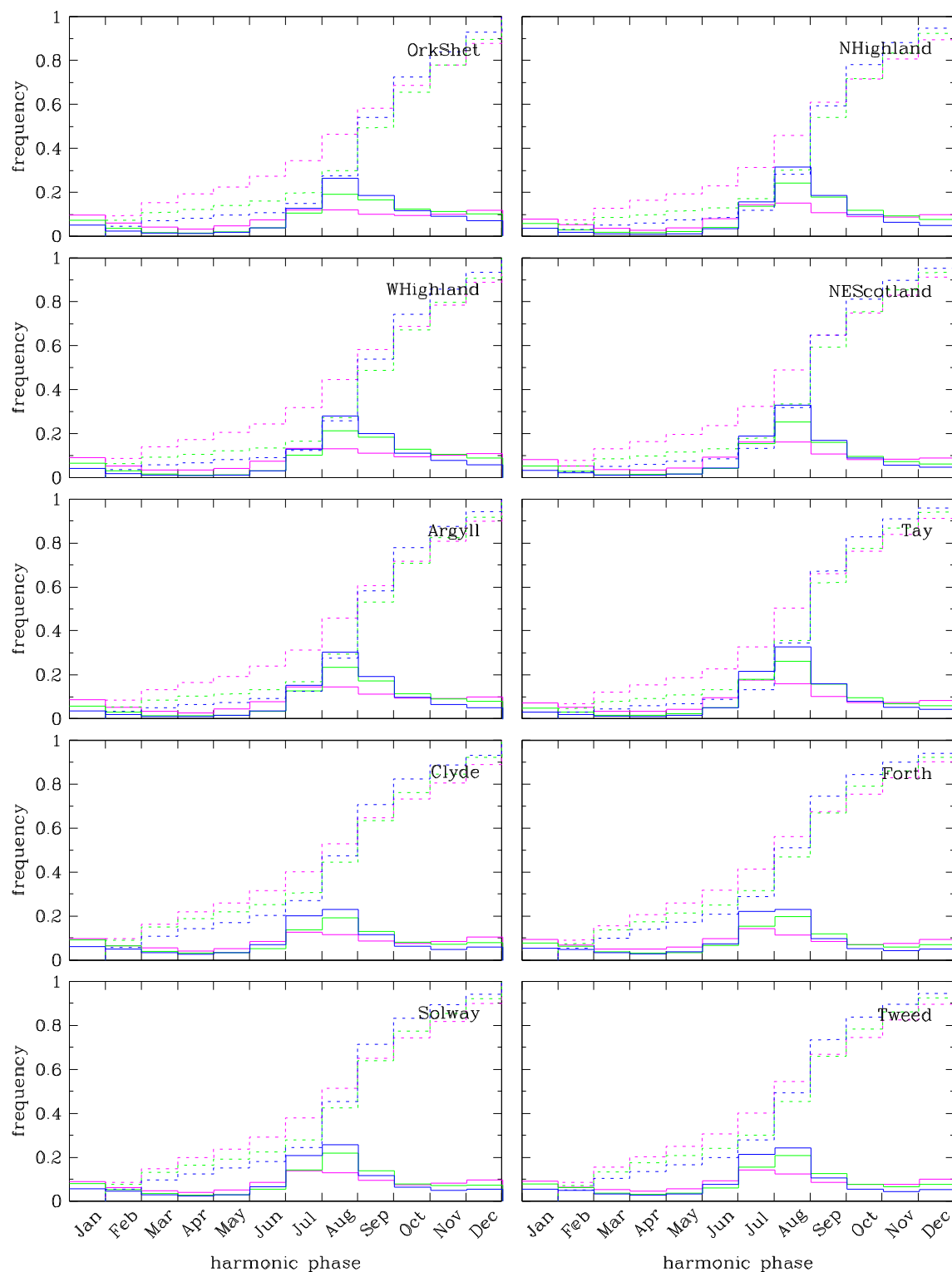
Figure A.11 Histograms and cdfs of the phases of the harmonic functions fitted to the UKCP09 temperature Sampled Data (Medium emissions: 2020s – magenta, 2050s – green, 2080s – blue), for each of the 10 river-basin regions in Scotland.
