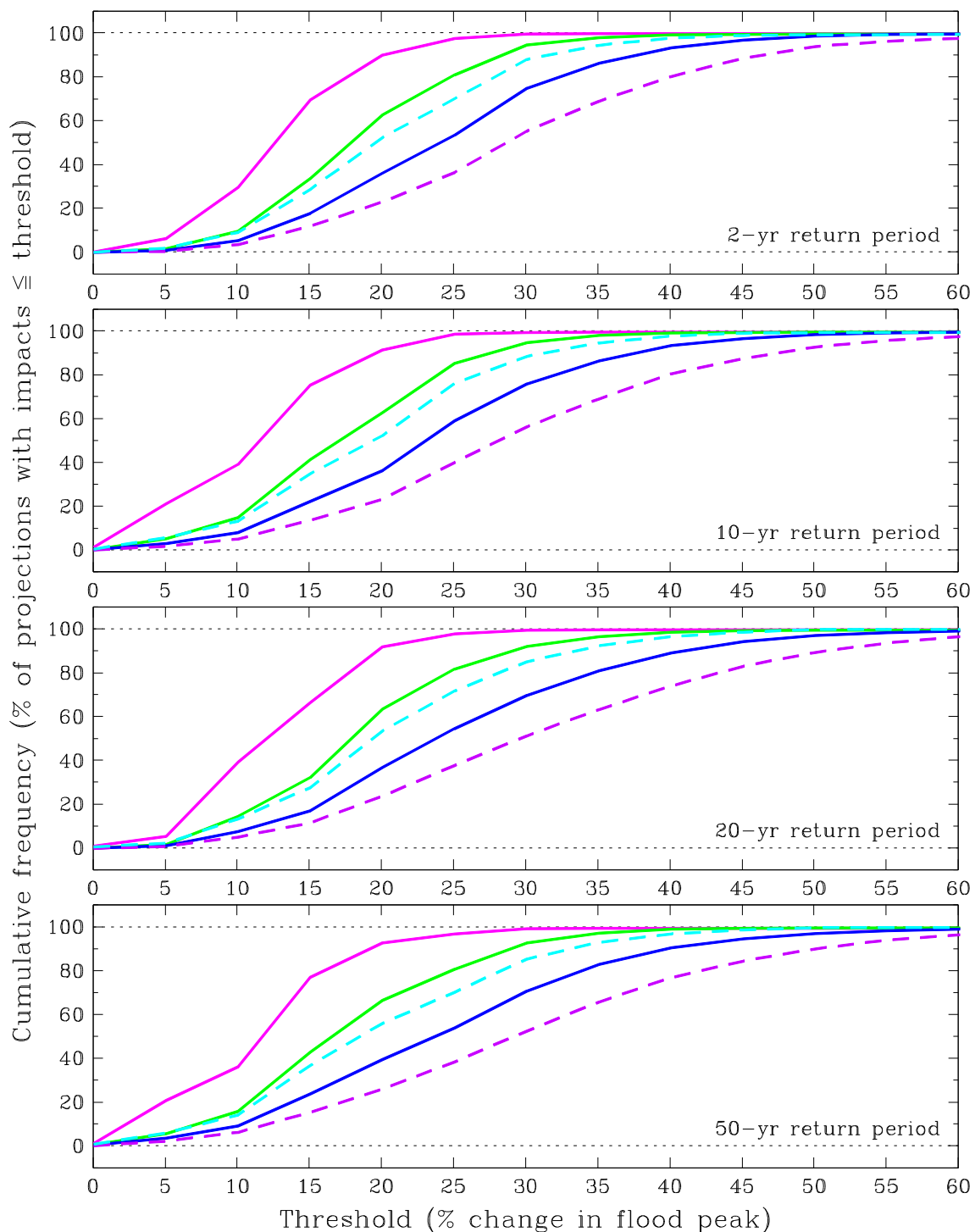
Figure B.45 Regional risk cdfs (central-estimates) for the North Highland river-basin region, for five different time-horizon / emissions scenario combinations: 2020s Medium (magenta solid), 2050s Medium (green solid), 2080s Medium (blue solid), 2080s Low (cyan dashed), 2080s High (purple dashed).
