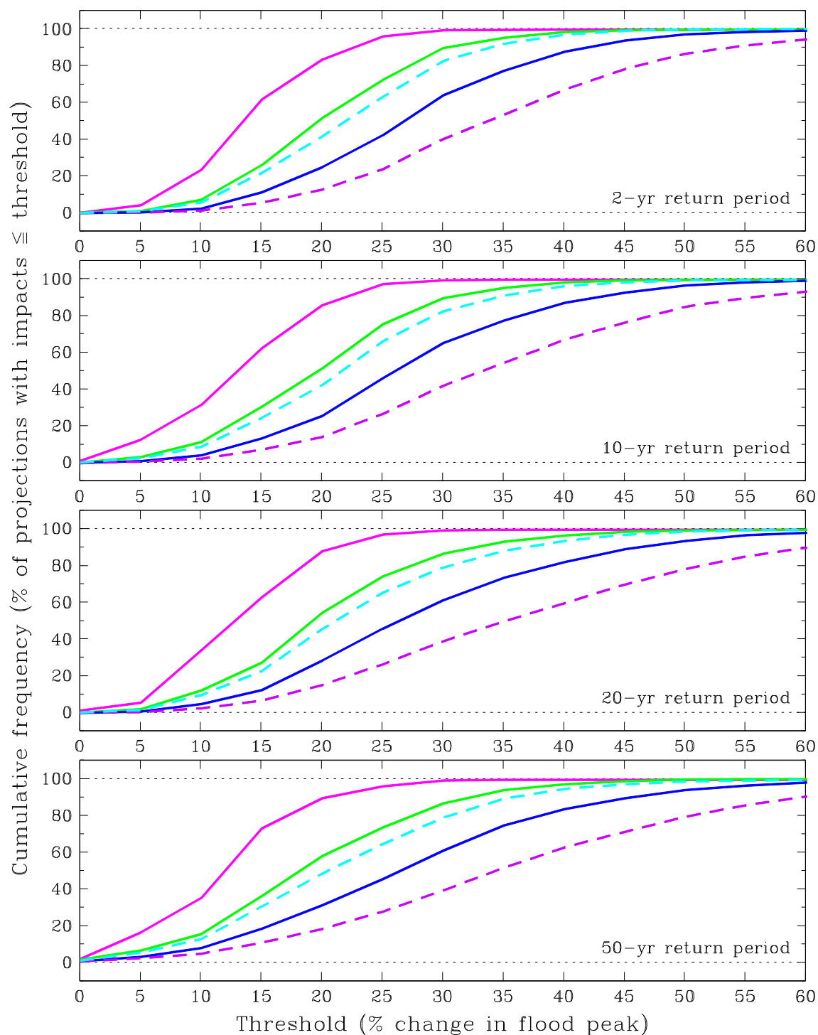
Figure B.51 As Figure B.45 but for the Clyde river-basin region.
