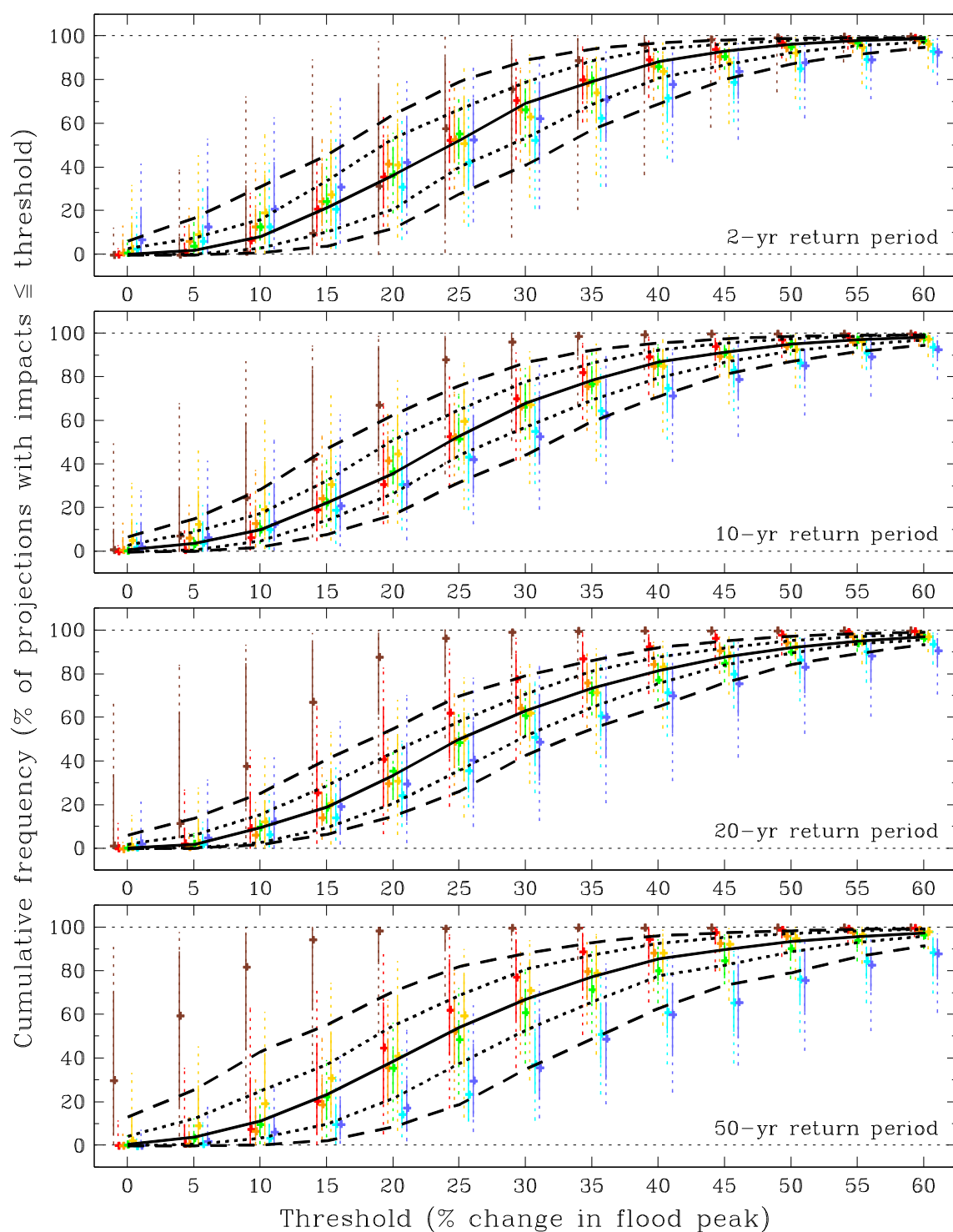
Figure B.35 As Figure B.31 but for the Tweed river-basin region (2080s High).
