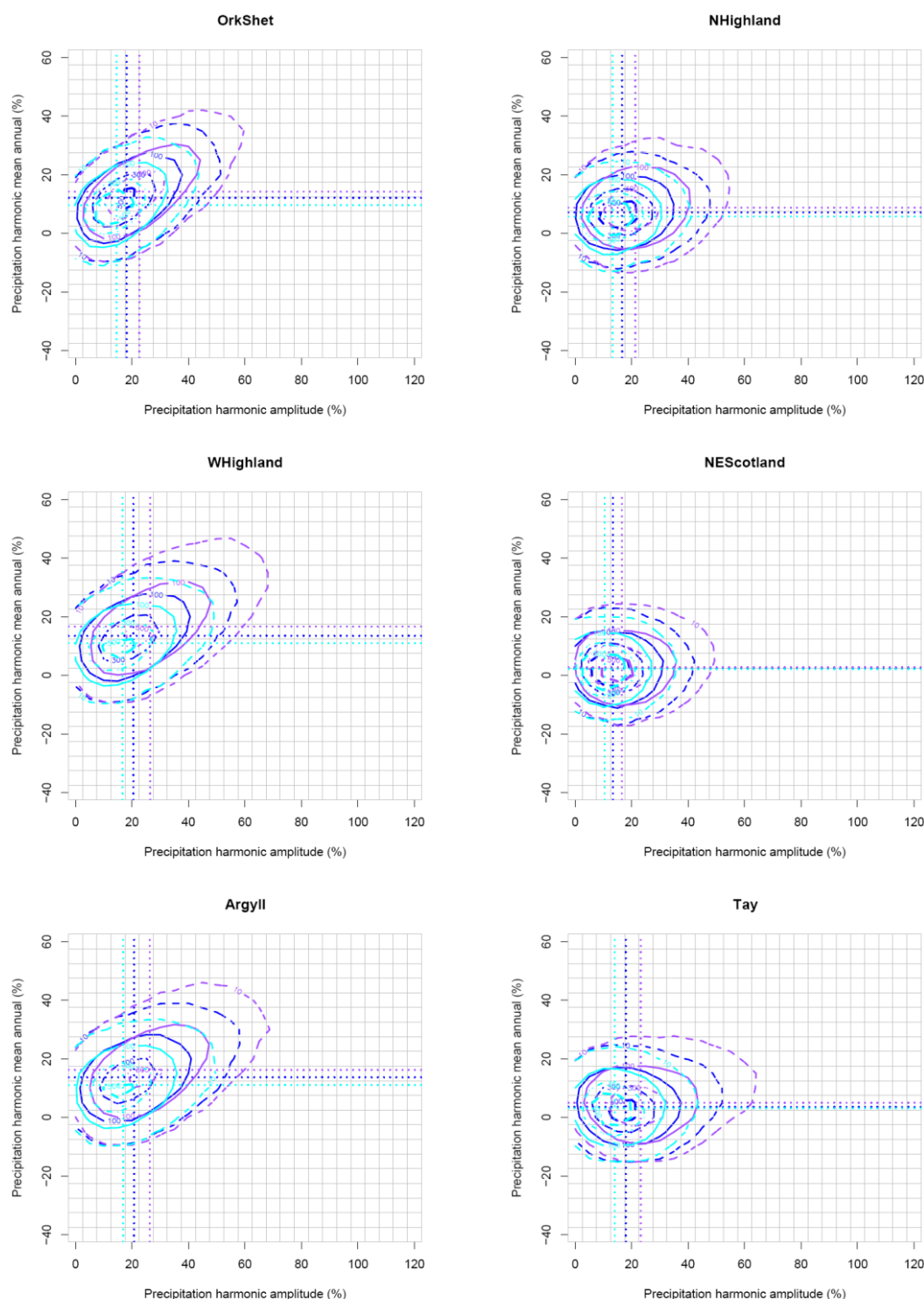
Figure A.8 Contours plots of the mean versus the amplitude of the harmonic functions fitted to the UKCP09 precipitation Sampled Data (2080s: Low emissions – cyan, Medium emissions – blue, High emissions – purple), for each of the 10 river-basin regions in Scotland. The median of each harmonic parameter is shown by the dotted horizontal/vertical lines. Note that the grid on these plots is the same as that of the FD2020 sensitivity framework (Table 1.1) and thus of the response patterns and standard deviation patterns (Figure 1.3 and Figure 1.4). The contours mark densities of 10, 100, 300 and 500 scenarios per grid square, where required. Figure continued on next page.
