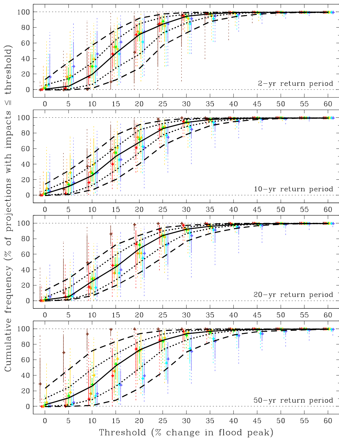
Figure B.25 As Figure B.21 but for the Tweed river-basin region (2080s Low).
