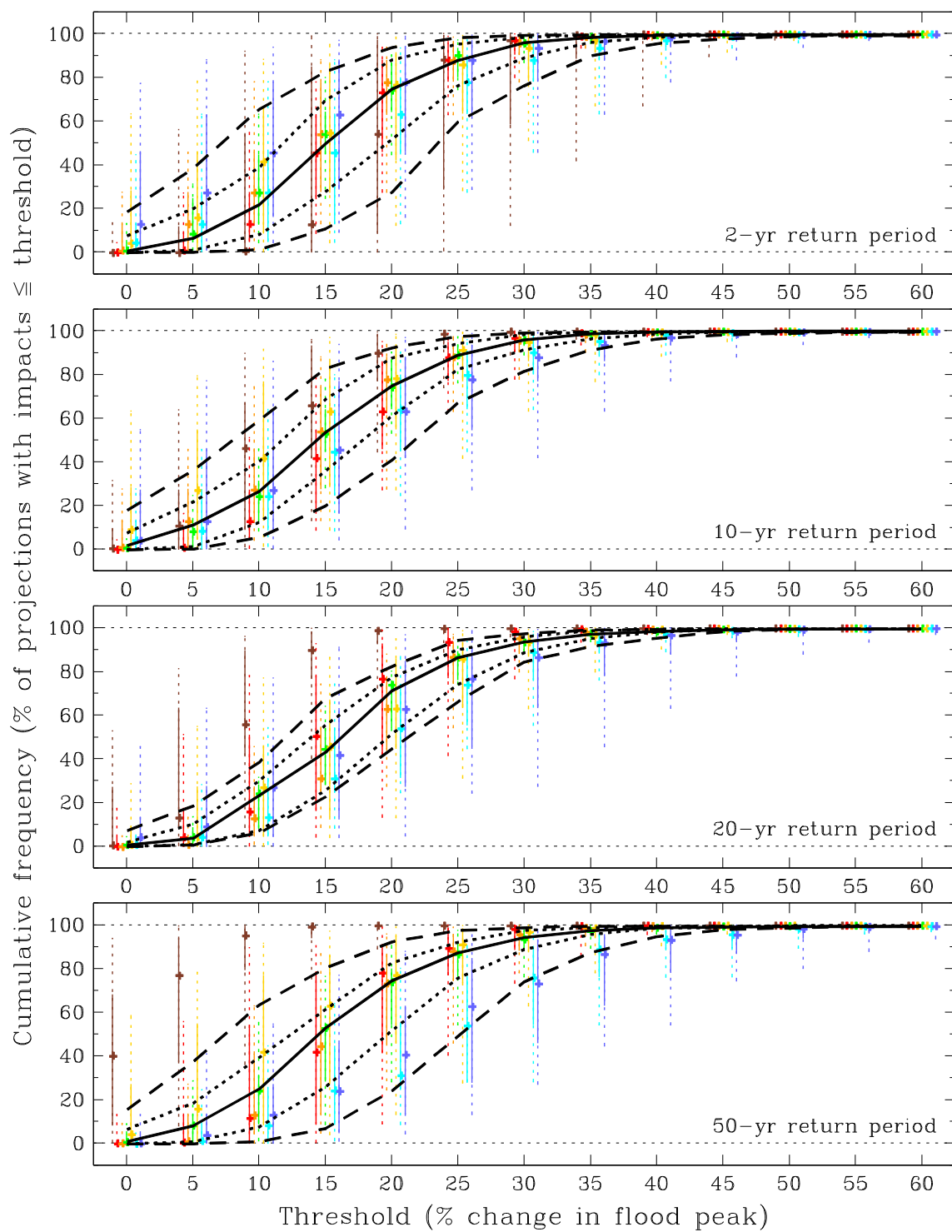
Figure B.13 As Figure B.11 but for the Tay river-basin region (2050s Medium).
