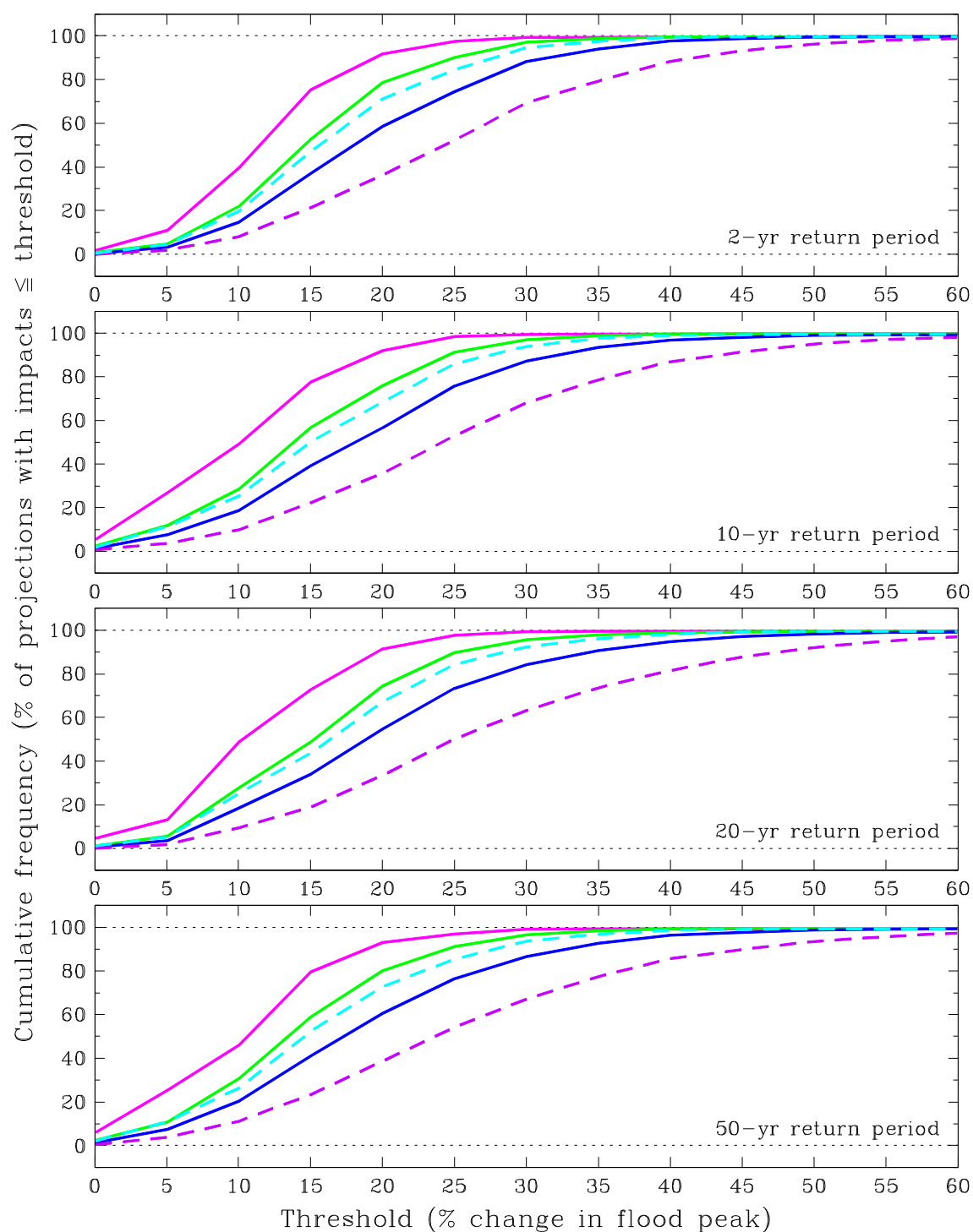
Figure B.49 As Figure B.45 but for the Tweed river-basin region.
