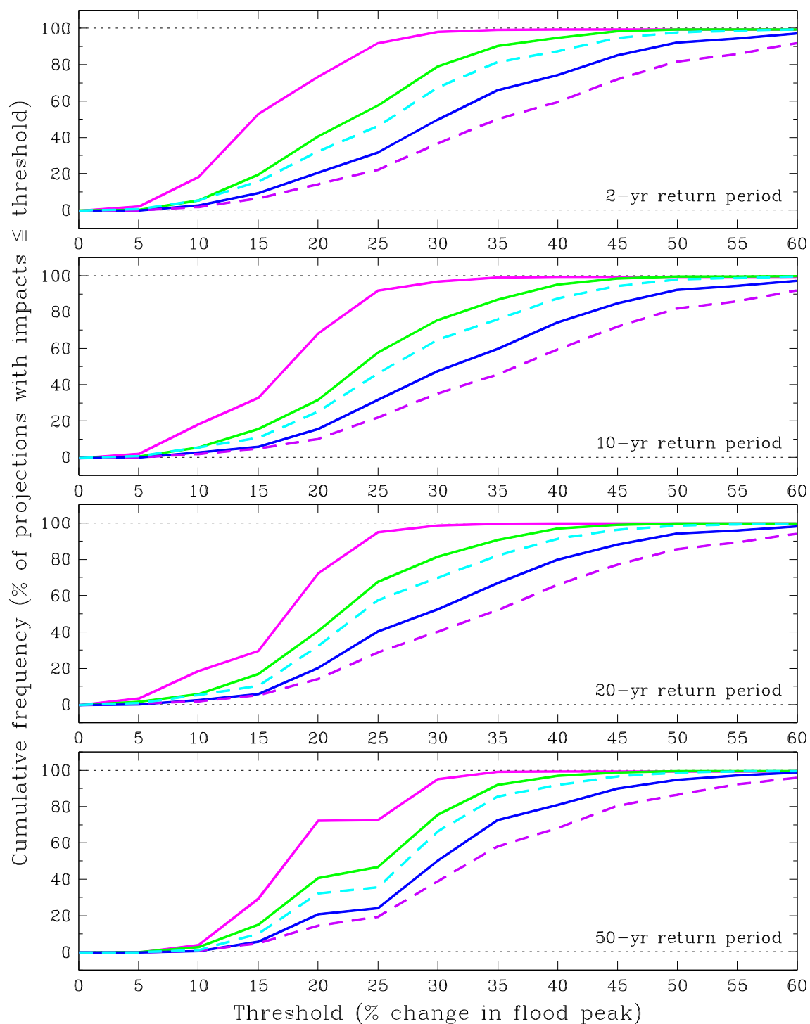
Figure B.54 As Figure B.45 but for the Orkney and Shetland river-basin region.
