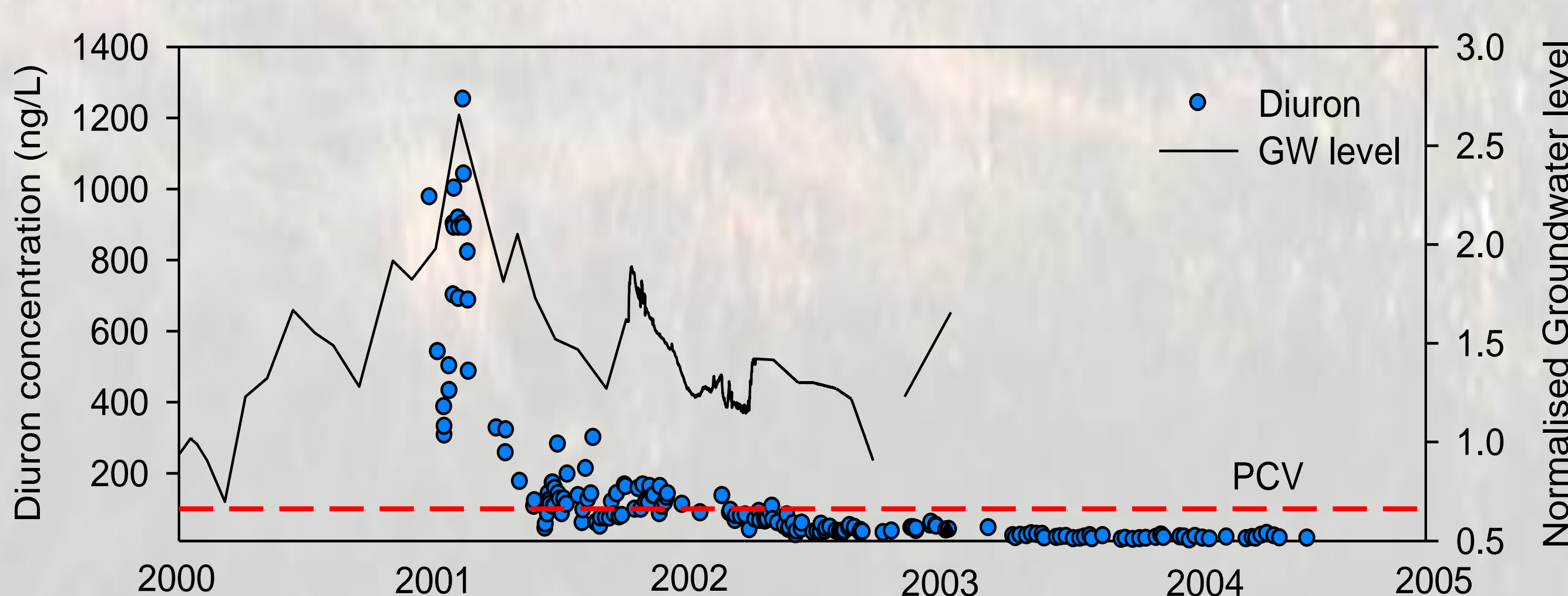
Changes in diuron concentration and normalised groundwater level in the Chalk aquifer of southeast England
