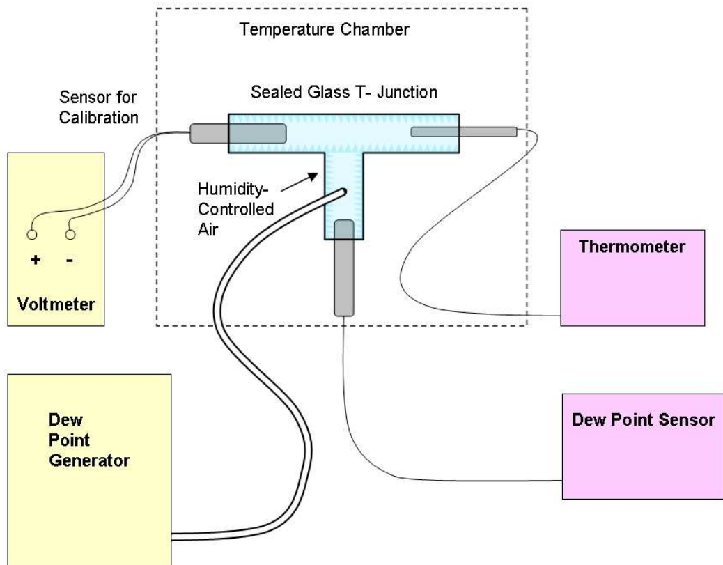
Figure 7: Equipment connection diagram
