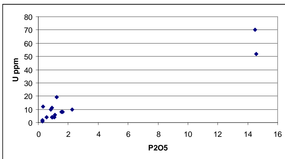
Figure 4. Correlation between U and P 2 O 5 .
