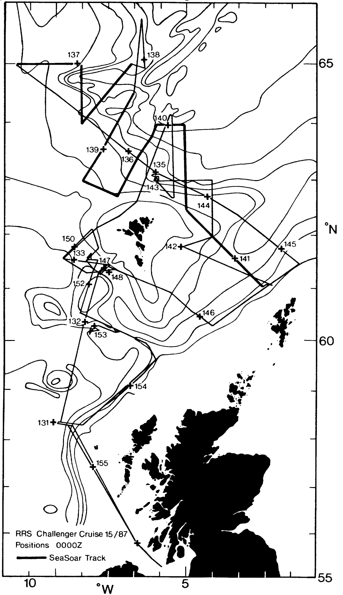
Fig.1 Track chart
