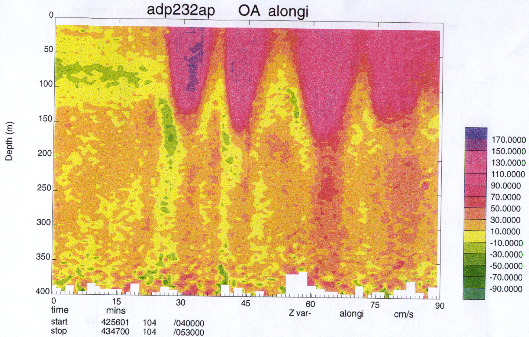
Figure 3. Alongstrait ( 77^{\circ}\text{T} ) Velocity (cm/sec) from underway ADCP sampling in the Strait of Gibraltar at L4E on 14 April between 0400 and 0530.
