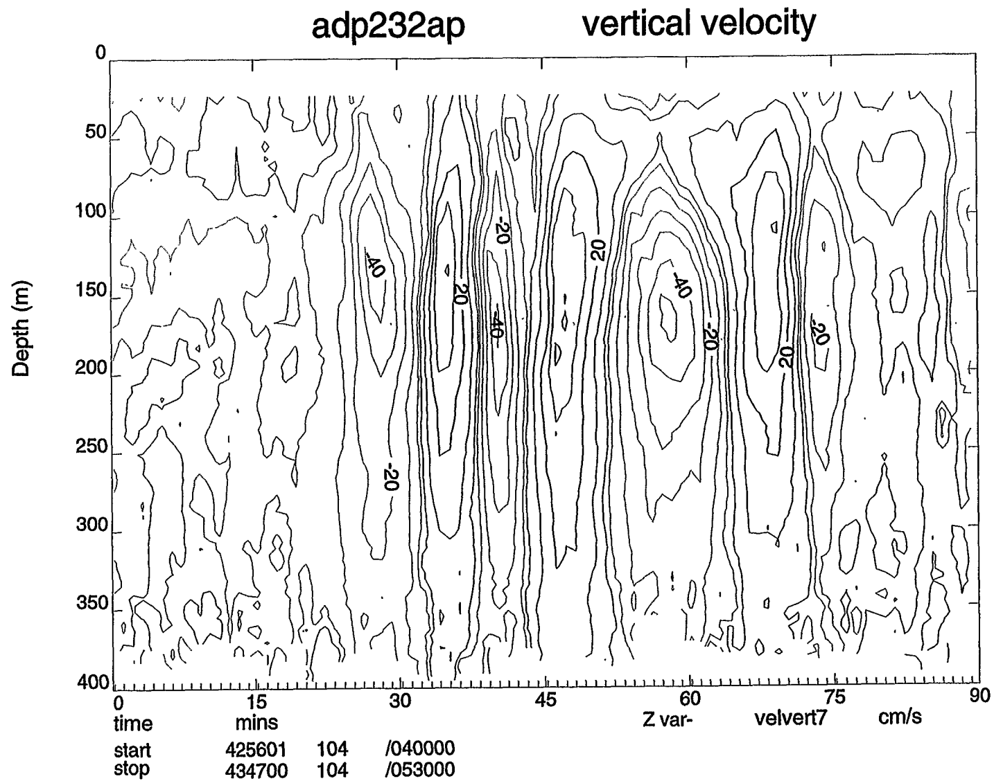
Figure 4. Vertical Velocity (cm/sec) from underway ADCP sampling in the Strait of Gibraltar at L4E on 14 April 1999 between 0400 and 0530
