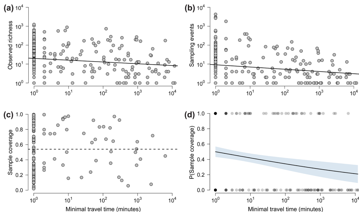
Figure 4. Effect of accessibility variation on tidal flat records. Plots show the effects of accessibility of tidal flats, as measured by the minimal travel time to reach a tidal flat from urban centres, on the observed species richness (a), sampling effort (b), and sample coverage (c). Solid and dashed lines indicate significant and non-significant relationships, respectively ( \alpha = 0.05 ). Plot (d) shows the logistic regression between accessibility to city centres and the probability of grid cells having enough data to calculate the sample coverage. Shadow indicates the 95% confidence interval.
