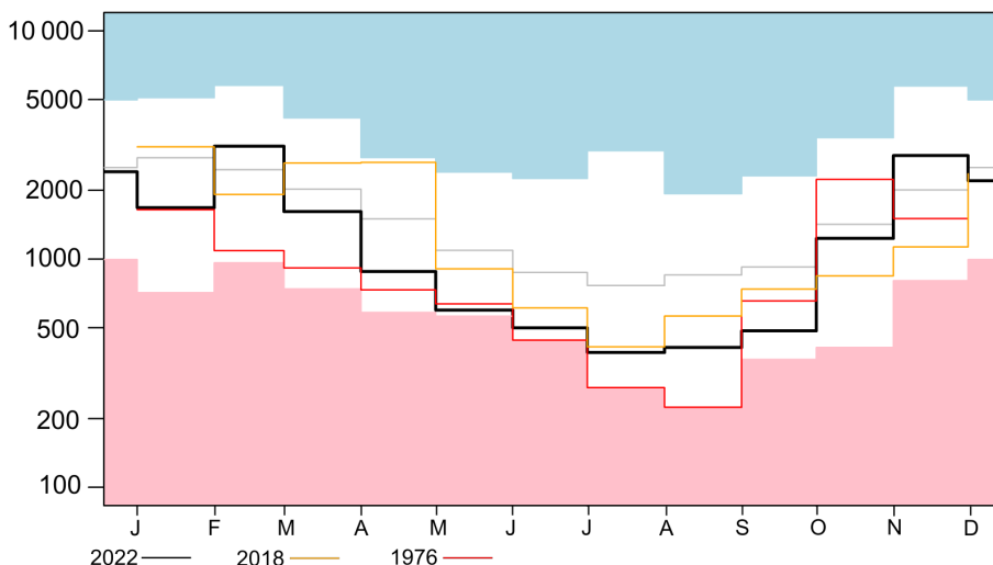
Figure 7. Monthly mean outflows ( \text{m}^3\text{s}^{-1} ) for England (thick black line) for 2022 showing the monthly maximum and minimum outflow (blue and red shading, respectively) and the long-term average (grey line), as well as the 1976 and 2018 droughts.
