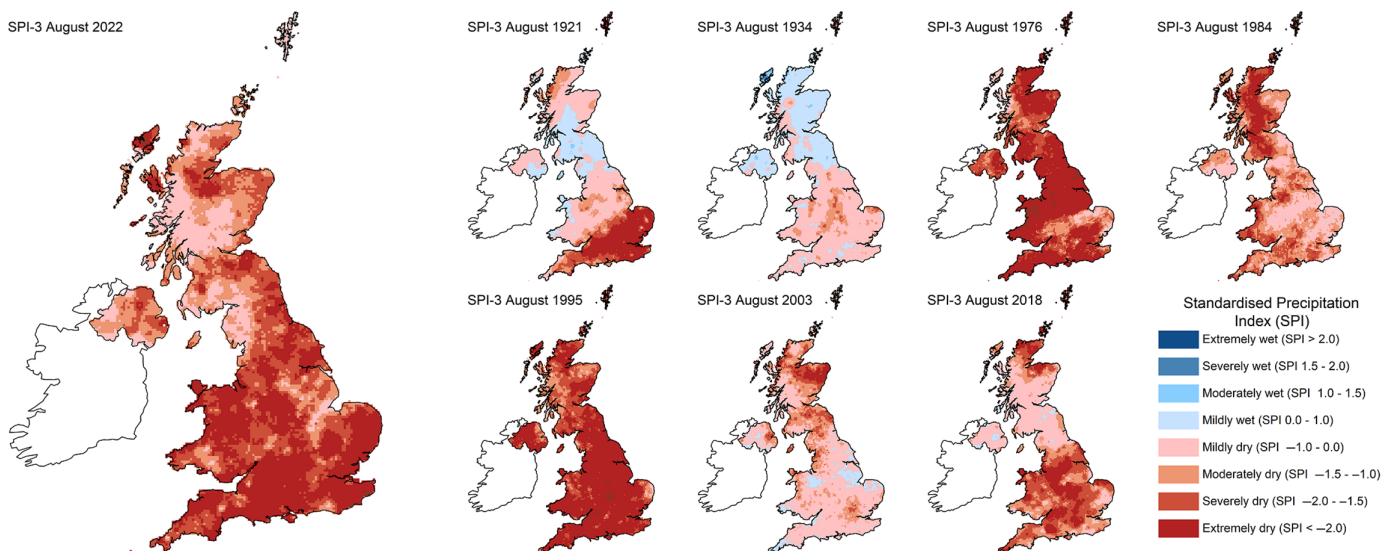
Figure 5. SPI for the 3-month period ending in August (i.e. June–August) for 2022, 1921, 1934, 1976, 1984, 1995, 2003 and 2018.
