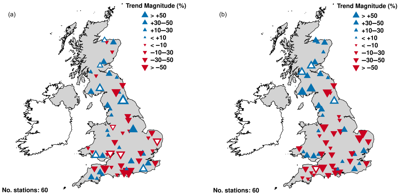
Figure 10. Trend analysis of river flow indicators (a) Q95 and (b) Seasonal Summer flows for the period 1965 to 2022, for all NHMP sites (N.B. naturalised data used for the River Thames). Trend magnitude (using the Thiel-Sen slope estimator) is shown according to the key as a percentage change. White colouration of triangles denotes a significant trend (using the Mann-Kendall trend test, at the 5% level).
