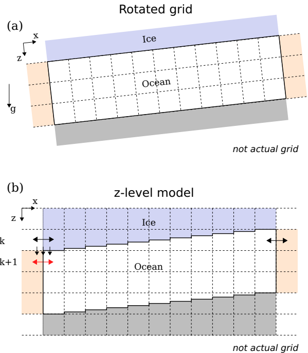
FIG. 1. Schematic representation of (a) the rotated domain for the 1D and LES models and (b) the shifted lateral boundary conditions undertaken for the z -level model. Shading represents the ice topography (blue), the solid lower boundary (gray), and the communication cells of the periodic boundary (orange). Dashed lines represent the grid layout. The ocean boundary is marked by the solid black line. In (b), black arrows show the alignment of existing boundary communication in the z -level model, and the red arrow shows an example of shifting this communication by one cell. The number of grid cells used in the model simulations far exceeds what is shown here.
