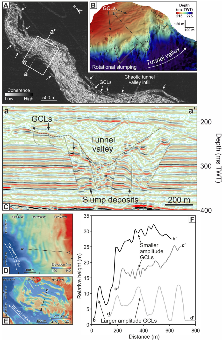
Fig. 5. Buried glacial curvilineations (GCLs) imaged within tunnel valleys. (A) Timeslice of seismic coherence at 290 ms TWT displaying curvilinear seismic anomalies (GCLs) along the sides of a tunnel valley in high-resolution 3D seismic data. (B) Oblique view of a picked seismic surface displaying GCLs and rotational slump scars along the tunnel valley sides. (C) Seismic section displaying the location of GCLs, slump deposits and faulting (semi-transparent lines) within the tunnel valley. (D, E) Examples of terrestrial GCLs in North America identified by Clark and Livingstone (2018) using the USA’s national elevation dataset (NED) ( http://nationalmap.gov/elevation.html ). (F) Profiles of relative height across the GCLs present within the tunnel valley compared to terrestrial examples in North America.
