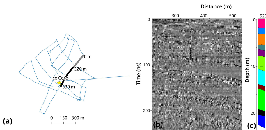
Figure 4. Mount Siple GPR. (a) Reference map depicts the full track of measurements (blue), the profile (grey), and the section shown in the radargram (black). (b) Radargram ending at the position of the ice core extraction (star) shown with layer interpretation and (c) estimated depth of layers.
