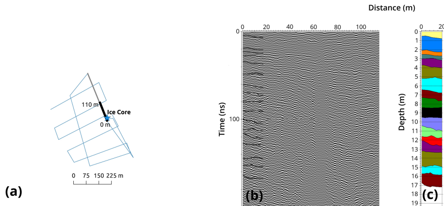
Figure 5. Young Island GPR. (a) Reference map depicts the full track of measurements (blue), the profile (grey), and the section shown in the radargram (black). (b) Section of a radargram obtained walking in NW direction from the ice core, shown with layer interpretation and (c) estimated depth of layers. A crevasse was detected at 70 m from the starting point (discontinuity in the reflections).
