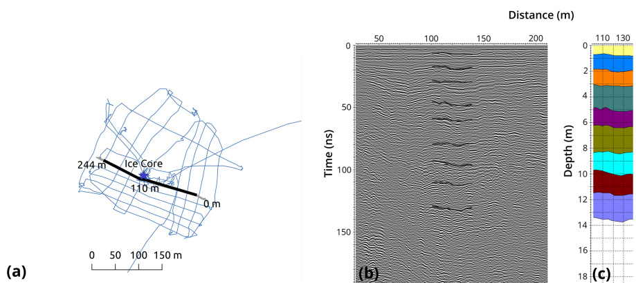
Figure 3. Peter I GPR. (a) Reference map depicts the full track of measurements (blue), the profile (grey), and the section shown in the radargram (black). (b) Section of a radargram taken in an east-westerly direction with layer interpretation and (c) estimated depth of layers.
