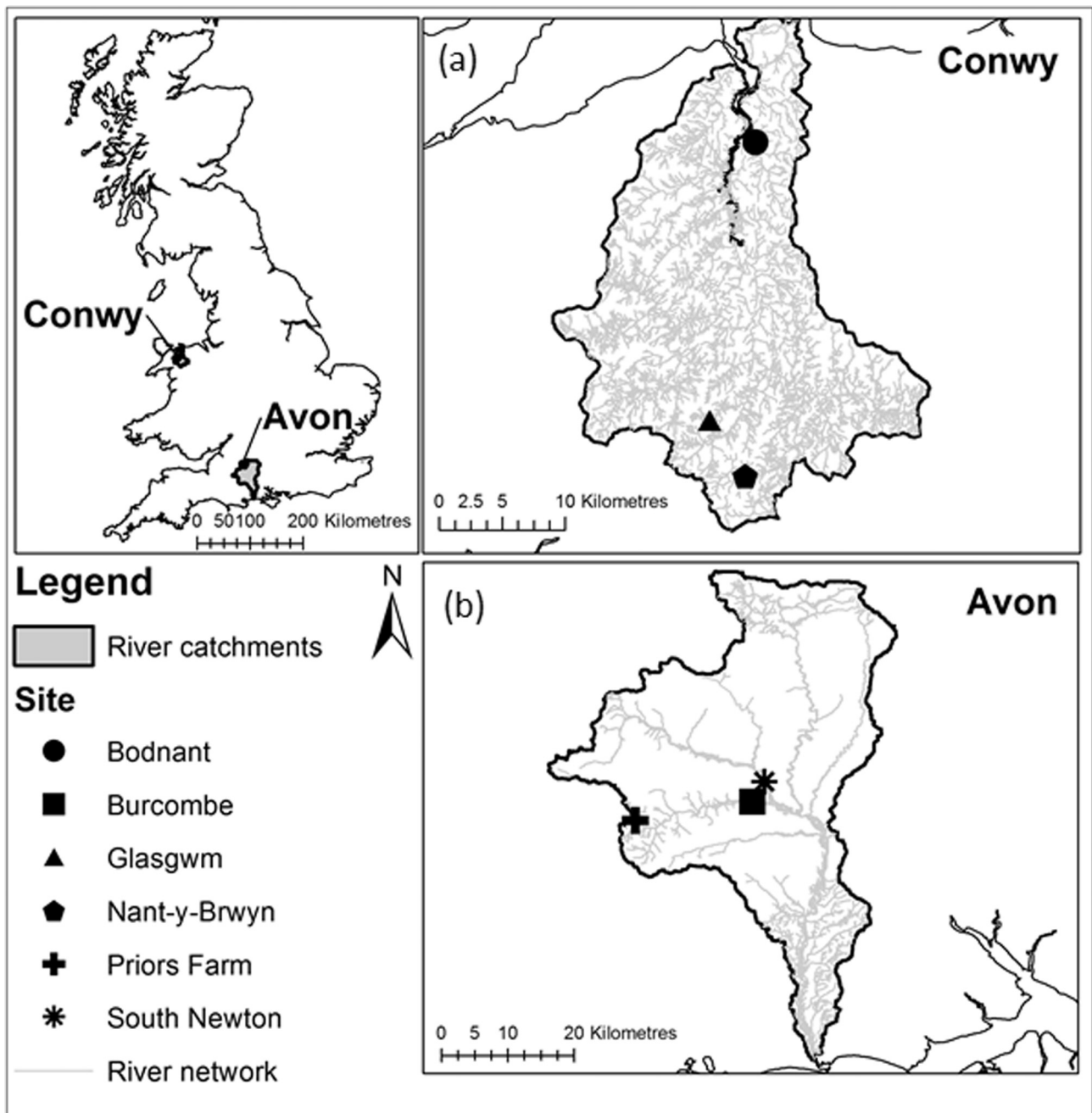
Fig. 1. Maps of studied catchments and sampling sites: Conwy, north Wales (a) and Hampshire Avon, southern England (b). Site latitude and longitude are given in Table 1.
