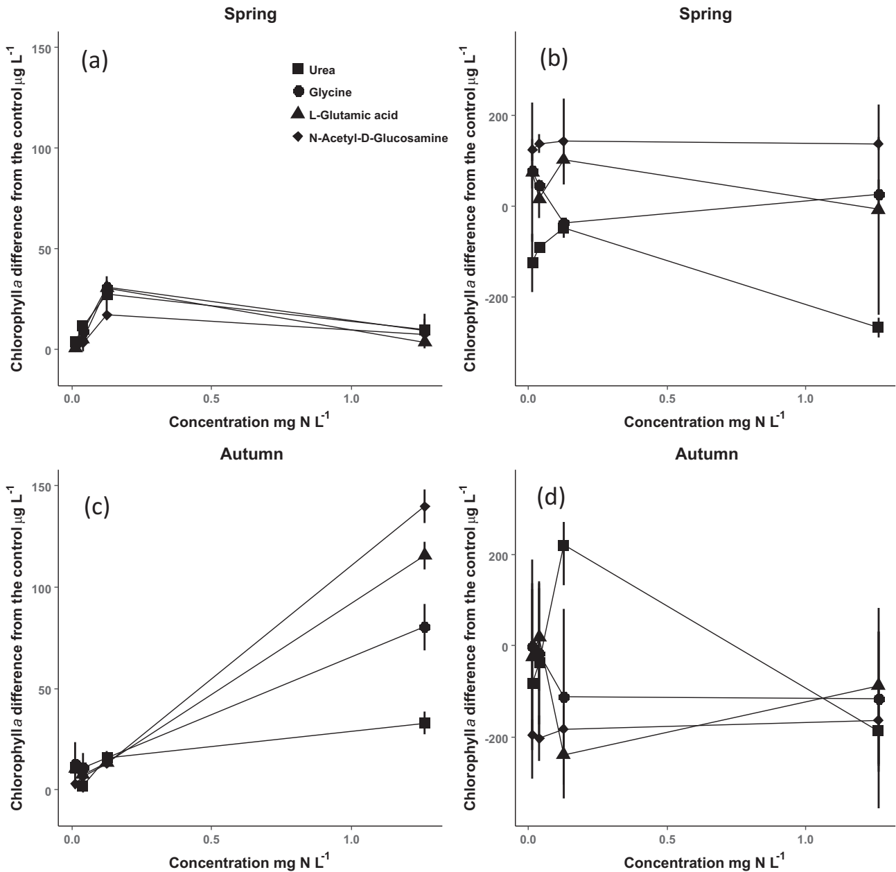
Fig. 6. The mean and standard deviation of the bioassay growth response of river phytoplankton to varying concentrations of DON compounds in spring and autumn 2017 at Nant-y-Brwyn (a and c) and South Newton (b and d).
