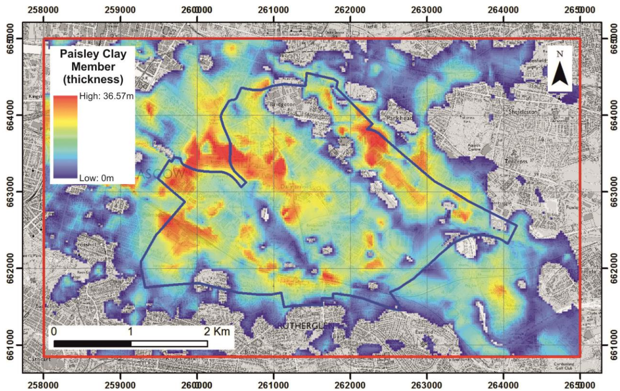
Figure 36 Modelled distribution and thickness of the Paisley Clay Member (PAIS) across the UKGEOS Glasgow superficial geology model area (red outline). These laminated marine clays and silts are extensive within the Clyde Valley and are over 30 m thick in places. 1 km grid squares shown. Includes mapping data licensed from Ordnance Survey. © Crown Copyright and/or database right 2019. Licence number 100021290 EUL.
