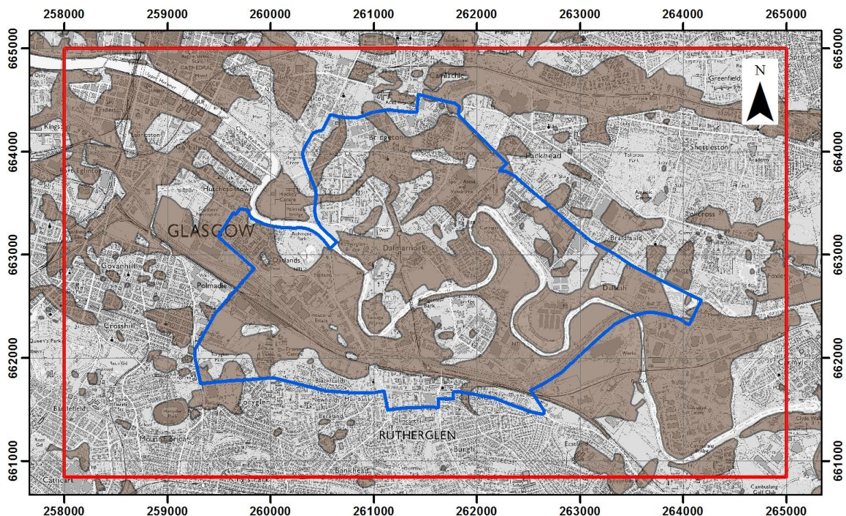
Figure 11: Modelled distribution of made ground (MGR), across the UKGEOS Glasgow superficial geology model area (red outline). 1 km grid squares shown. Includes mapping data licensed from Ordnance Survey. © Crown Copyright and/or database right 2019. Licence number 100021290 EUL).
