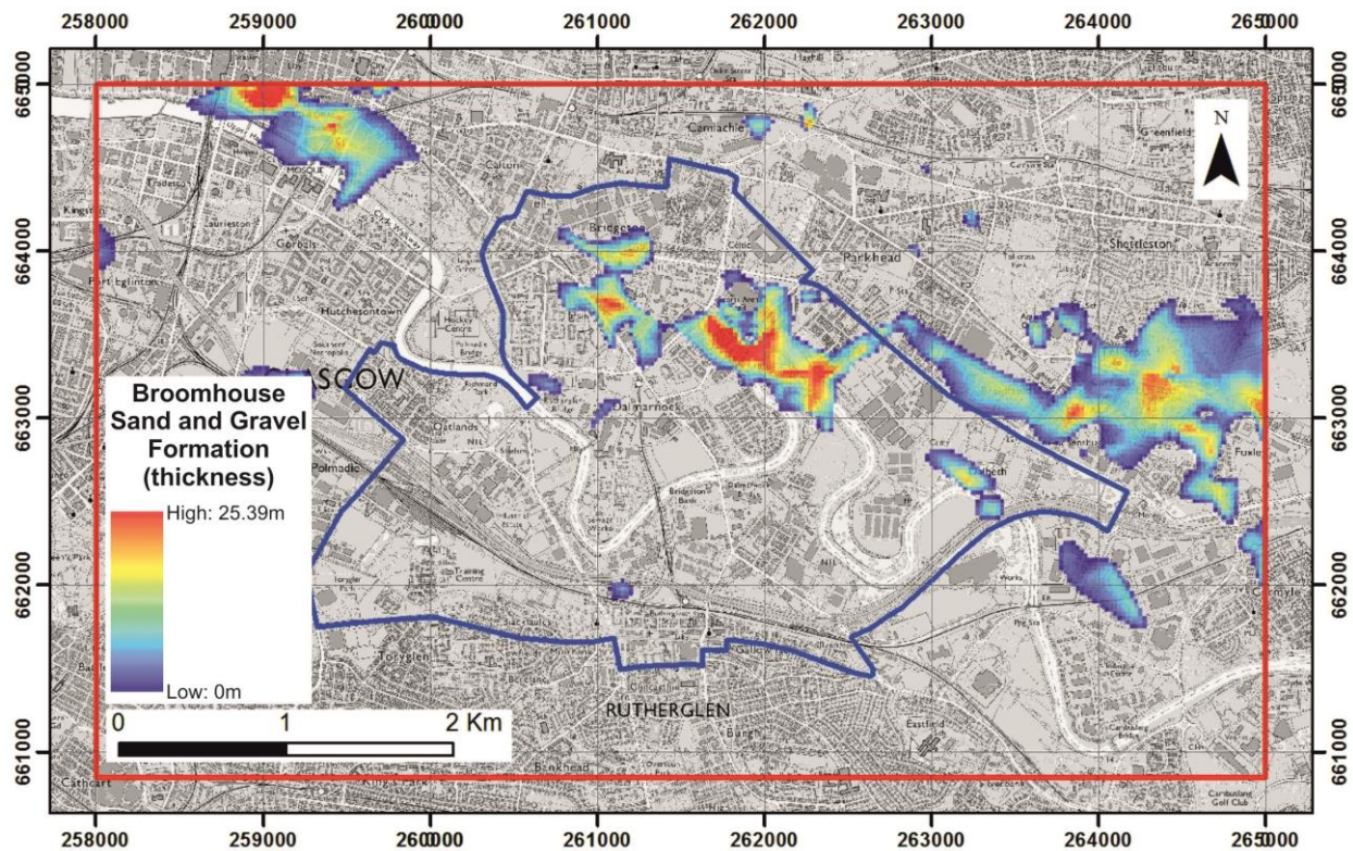
Figure 38 Modelled distribution and thickness of the Broomhouse Sand and Gravel Formation (BHSE) across the UKGEOS Glasgow superficial geology model area (red outline). This deposit of fluvioglacial sand and gravels generally occurs at a significant depth beneath the surface, as its known occurrence (shown above) is dependent on the presence of deep borehole records more extensive deposits may lie undetected in areas where there are a lack of data points. The unit is over 20 m thick in places. 1 km grid squares shown. Includes mapping data licensed from Ordnance Survey. © Crown Copyright and/or database right 2019. Licence number 100021290 EUL.
