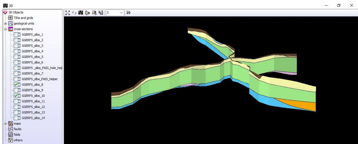
Figure 32 Cross-sections GGERFS_slba_8 and GGERFS_slba_10 as viewed in the 3D window of GSI3D. These two sections pass through the proposed site for borehole GGERFS10 at Dalmarnock (see Figure 16 for location and orientation of sections). The sections illustrate the calculated sequence and thickness of superficial deposits beneath this part of the UKGEOS Glasgow model area from available borehole and map data. Vertical exaggeration x 10. Ground surface derived from NEXTMap Britain elevation data from Intermap Technologies. Borehole constraint points along the sections and thickness of the geological units are indicated in Figures 24 and 25.
