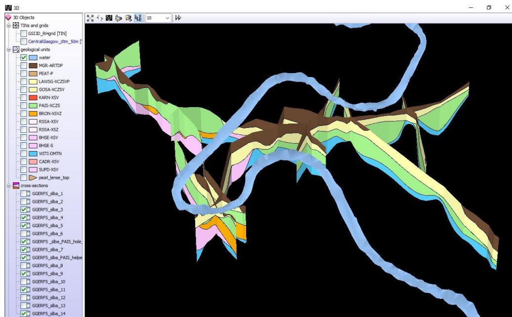
Figure 33 Nine cross-sections as viewed in the 3D window of GSI3D. This network of sections pass through the proposed sites for the Cuningar Loop boreholes (see Figure 16 for location and orientation of sections). The sections illustrate the calculated sequence and thickness of superficial deposits beneath this part of the UKGEOS Glasgow model area from available borehole and map data. Vertical exaggeration x 10. Ground surface derived from NEXTMap Britain elevation data from Intermap Technologies. Borehole constraint points along some of the sections and thickness of the geological units are indicated in Figures 24 and 25.
