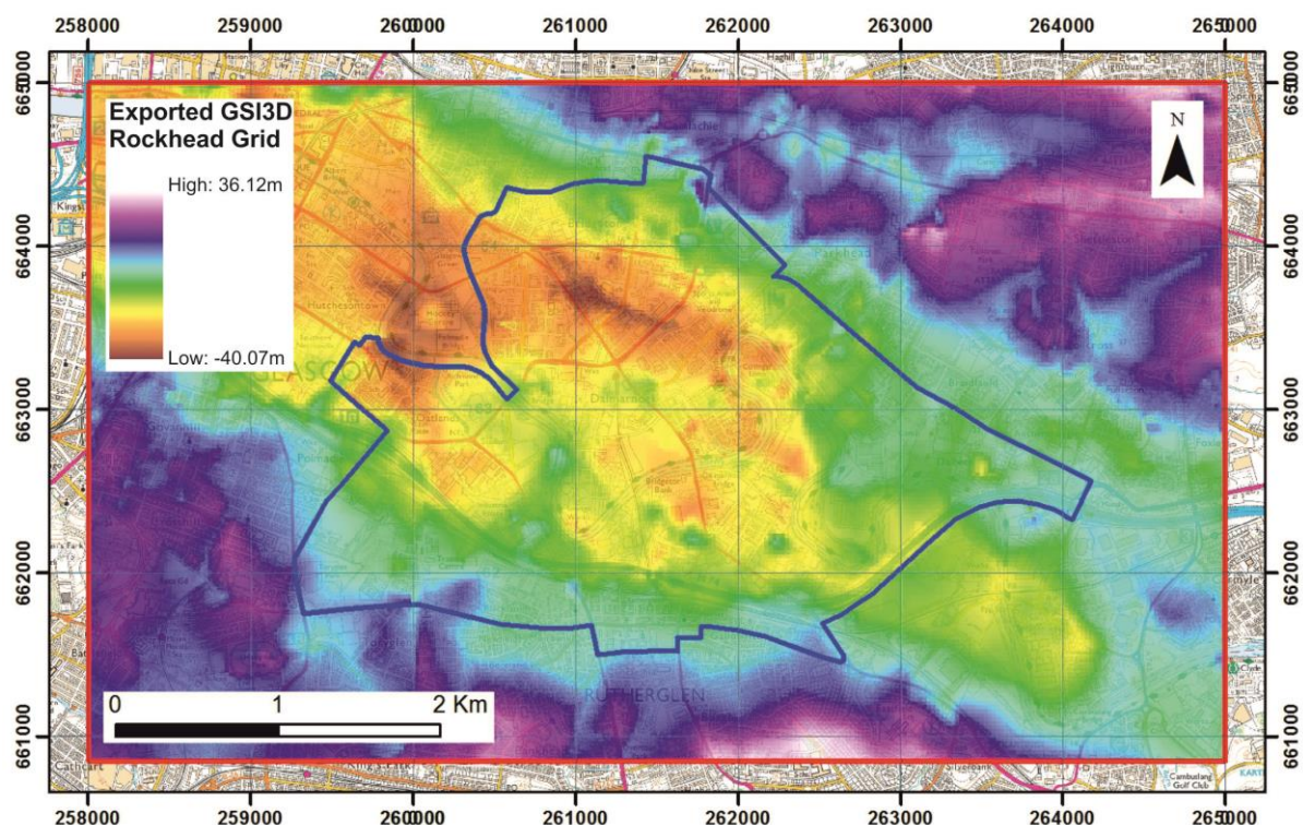
Figure 19 Rockhead surface for the study area, generated in GSI3D by combining the bases of all the modelled superficial units. Low values are in yellow and brown and high values are in purple and white. Includes mapping data licensed from Ordnance Survey. © Crown Copyright and/or database right 2019. Licence number 100021290 EUL).
