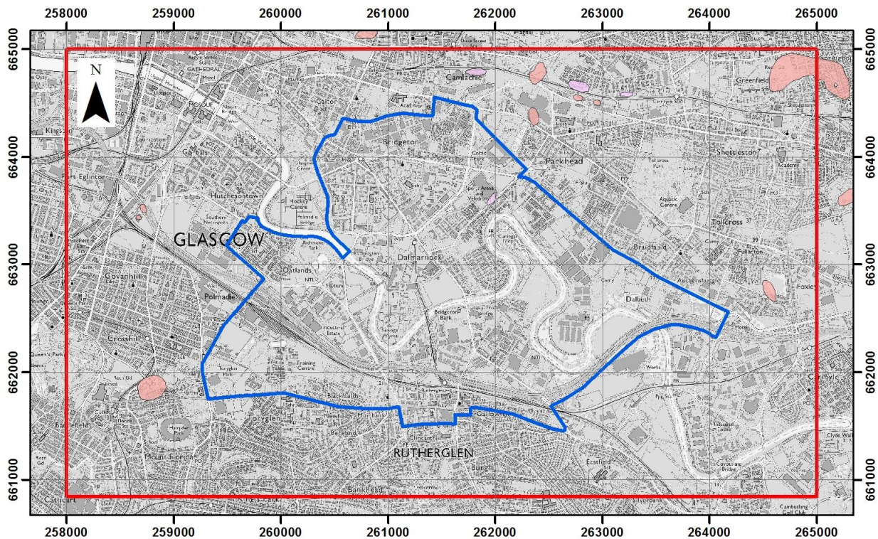
Figure 4: Modelled distribution of Cadder Sand and Gravel Formation (orangey pink) and the Sand and Gravel unit (pink) across the UKGEOS Glasgow model area (red outline). 1 km grid squares shown. Includes mapping data licensed from Ordnance Survey. © Crown Copyright and/or database right 2019. Licence number 100021290 EUL.
