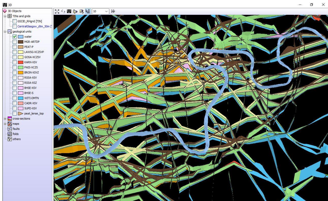
Figure 17 Network of sections constructed in the vicinity of the UKGEOS Glasgow model area viewed in 3D
