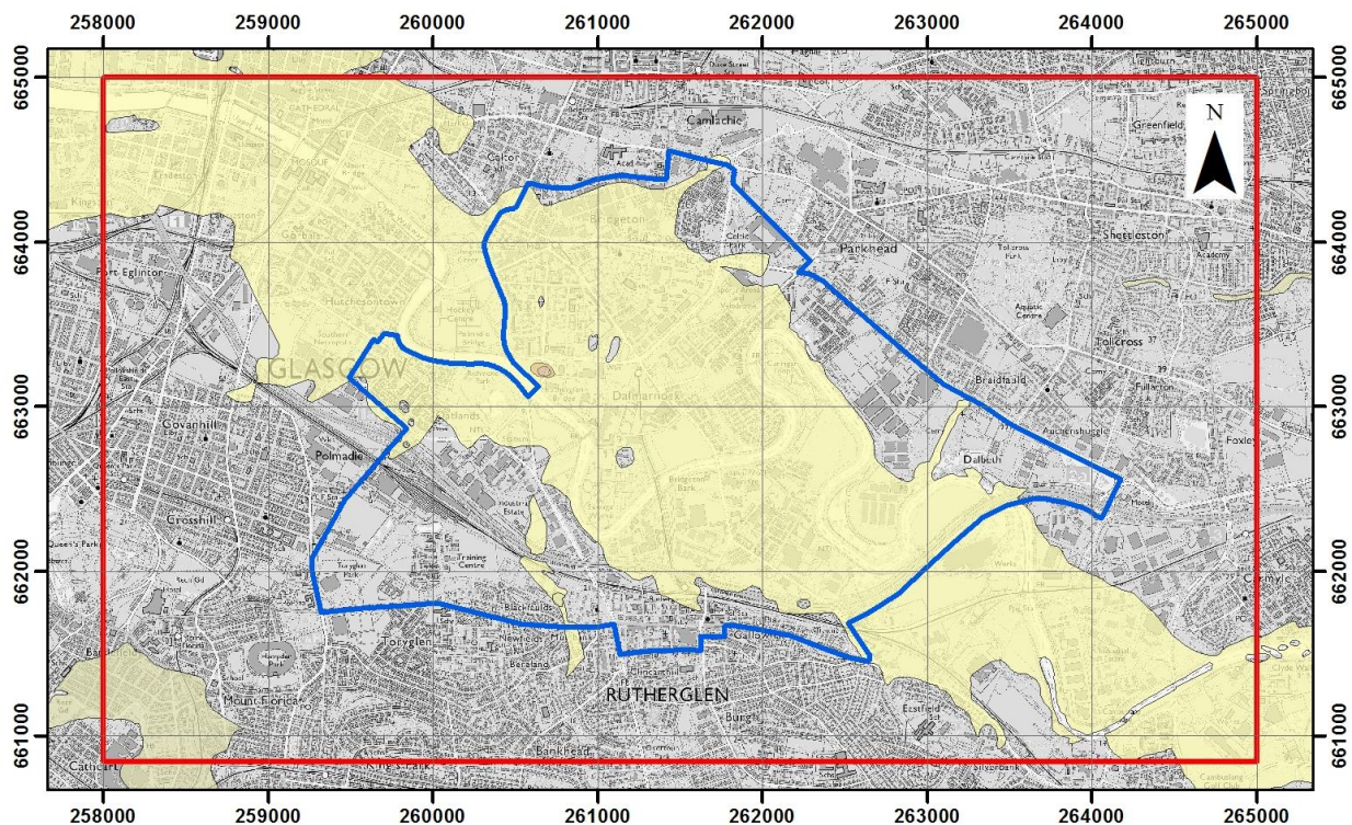
Figure 10: Modelled distribution of Gourrock Sand Member (pale yellow), Law Sand and Gravel Member (greenish yellow) and peat (brown), across the UKGEOS Glasgow superficial geology model area (red outline). 1 km grid squares shown. Includes mapping data licensed from Ordnance Survey. © Crown Copyright and/or database right 2019. Licence number 100021290 EUL).
