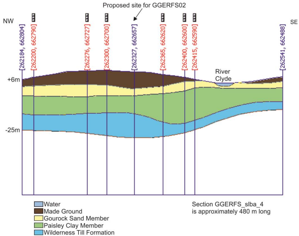
Figure 27 Cross-section GGERFS_slba_4 , orientated NW-SE through the superficial deposits of the UKGEOS Glasgow model area (see Figure 16 for location). Vertical exaggeration x 3. Borehole constraint points shown in red. Ground surface derived from NEXTMap Britain elevation data from Intermap Technologies. Height is in metres relative to Ordnance Datum.
