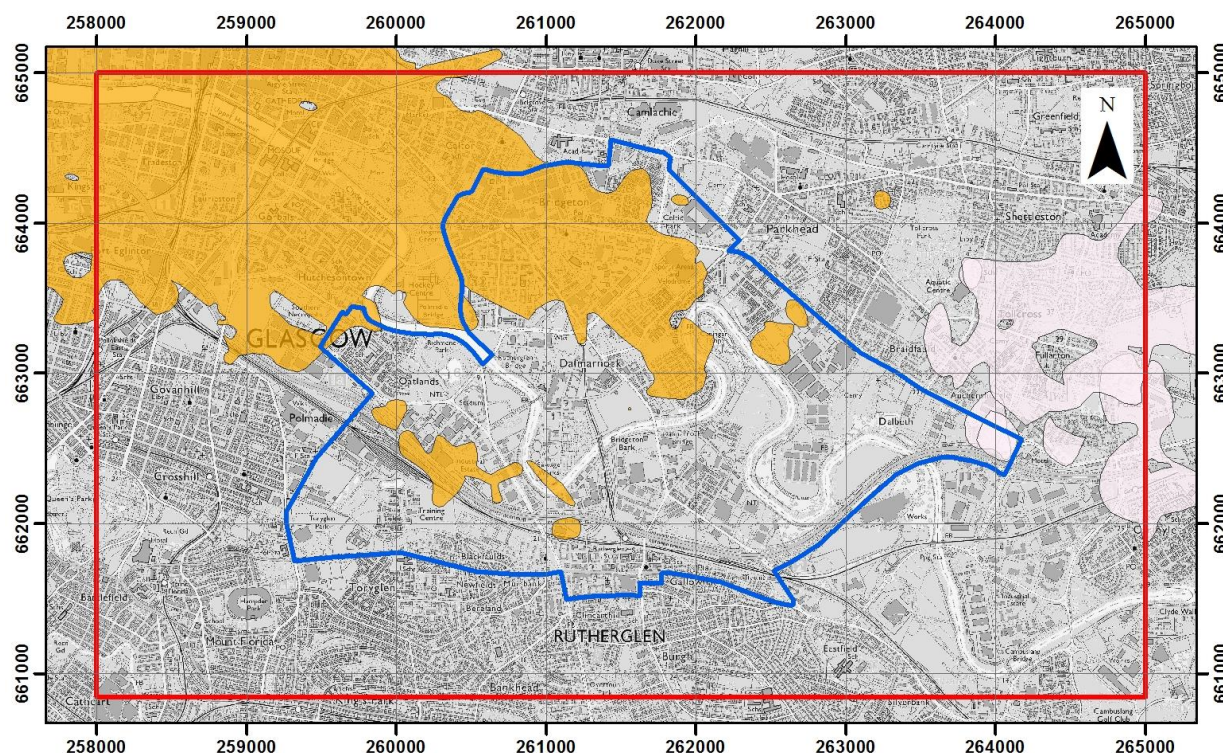
Figure 7: Modelled distribution of Broomhouse Sand and Gravel Formation (orange) and Ross Sand Member (pale pink), across the UKGEOS Glasgow superficial geology model area (red outline). 1 km grid squares shown. Includes mapping data licensed from Ordnance Survey. © Crown Copyright and/or database right 2019. Licence number 100021290 EUL).
