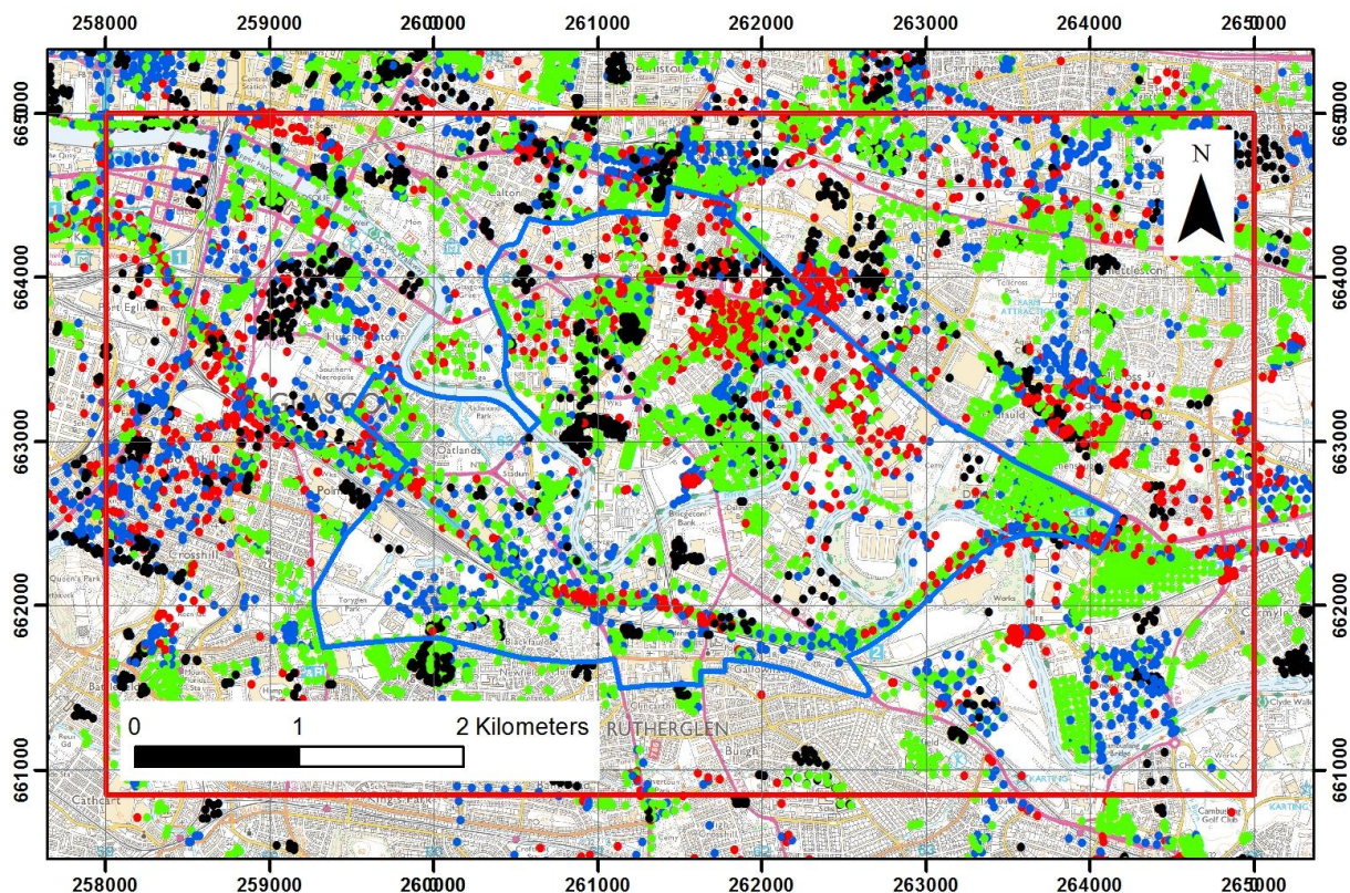
Figure 23 Location of borehole records held in the BGS Single Onshore Borehole Index database. Red dots (more than 30 m deep), blue dots (between 10 m and 30 m), green dots (less than 10 m) and black dots (depth unknown). Includes mapping data licensed from Ordnance Survey. © Crown Copyright and/or database right 2019. Licence number 100021290 EUL.
