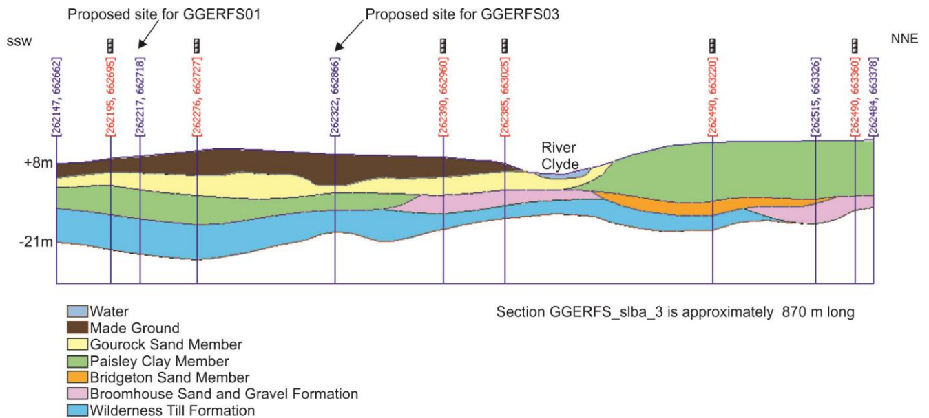
Figure 26 Cross-section GGERFS_slba_3 , orientated SSW-NNE through the superficial deposits of the UKGEOS Glasgow model area (see Figure 16 for location). Vertical exaggeration x 3. Borehole constraint points shown in red. Ground surface derived from NEXTMap Britain elevation data from Intermap Technologies. Height is in metres relative to Ordnance Datum.
