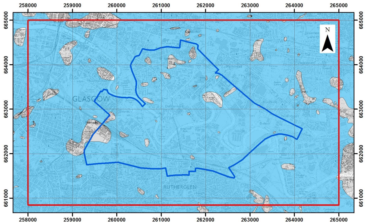
Figure 5: Modelled distribution of Wilderness Till Formation (pale blue) across the UKGEOS Glasgow superficial geology model area (red outline). 1 km grid squares shown. Includes mapping data licensed from Ordnance Survey. © Crown Copyright and/or database right 2019. Licence number 100021290 EUL).
