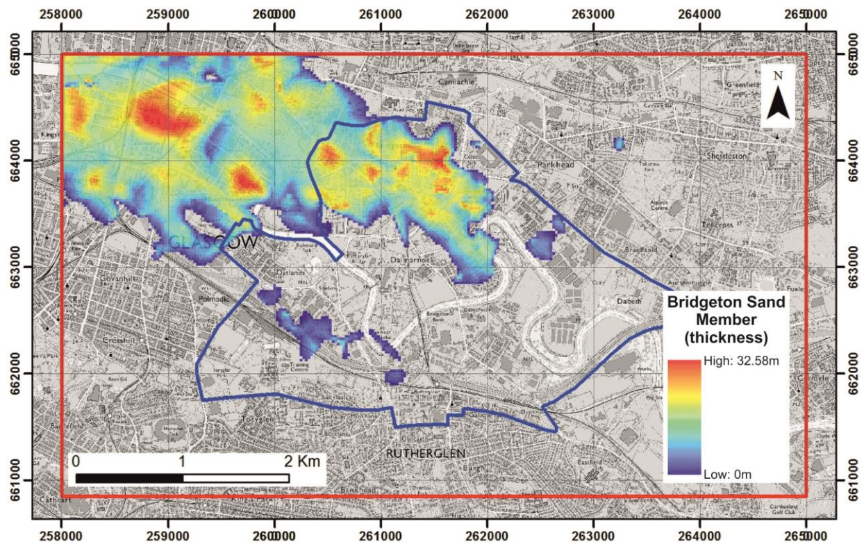
Figure 37 Modelled distribution and thickness of the Bridgeton Sand Member (BRON) across the UKGEOS Glasgow superficial geology model area (red outline). This deposit of marine sands is significant in the north-western corner of the modelled area where it is over 30 m thick in places. 1 km grid squares shown. Includes mapping data licensed from Ordnance Survey. © Crown Copyright and/or database right 2019. Licence number 100021290 EUL.
