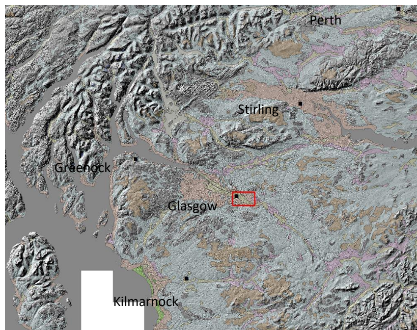
Figure 3 Location of the UKGEOS Glasgow study area (red rectangle) and the surrounding topography, depicted by the NEXTMap Surface model hillshade. Superficial deposits (DigMapGB-625k) are overlain as coloured tints: blue – glacial till, pink – glacial sand and gravel, orange – raised marine deposits, brown – peat, yellow – alluvium and green – blown sand.
