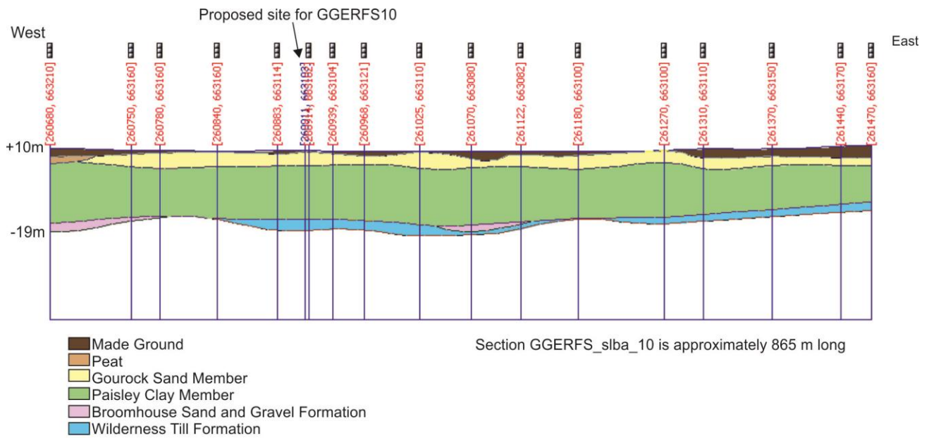
Figure 31 Cross-section GGERFS_slba_10 , orientated West-East through the superficial deposits of the UKGEOS Glasgow model area (see Figure 16 for location). Vertical exaggeration x 3. Borehole constraint points shown in red. Ground surface derived from NEXTMap Britain elevation data from Intermap Technologies. Height is in metres relative to Ordnance Datum.
