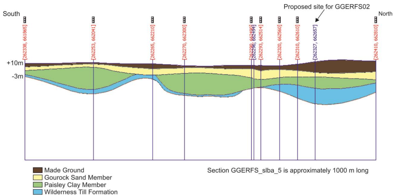
Figure 28 Cross-section GGERFS_slba_5 , orientated South-North through the superficial deposits of the UKGEOS Glasgow model area (see Figure 16 for location). Vertical exaggeration x 3. Borehole constraint points shown in red. Ground surface derived from NEXTMap Britain elevation data from Intermap Technologies. Height is in metres relative to Ordnance Datum.
