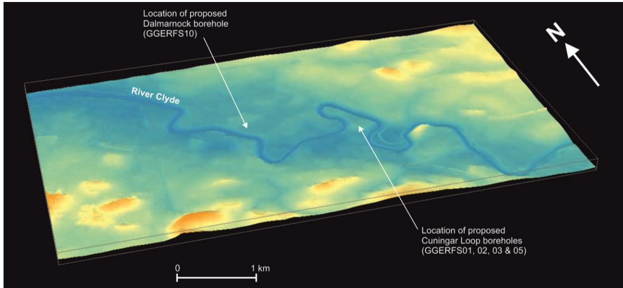
Figure 2 3D view of the Digital Terrain Model (5 m cell size) across the UKGEOS Glasgow area. The ground surface across the study area is between 2 m and 60 m above Ordnance Datum (OD). The course of the River Clyde can be clearly seen snaking its way north-westwards along the low ground of the Clyde valley (blue colours) with higher ground (orange colours) to the northeast and southwest. NEXTMap Britain elevation data from Intermap Technologies.
