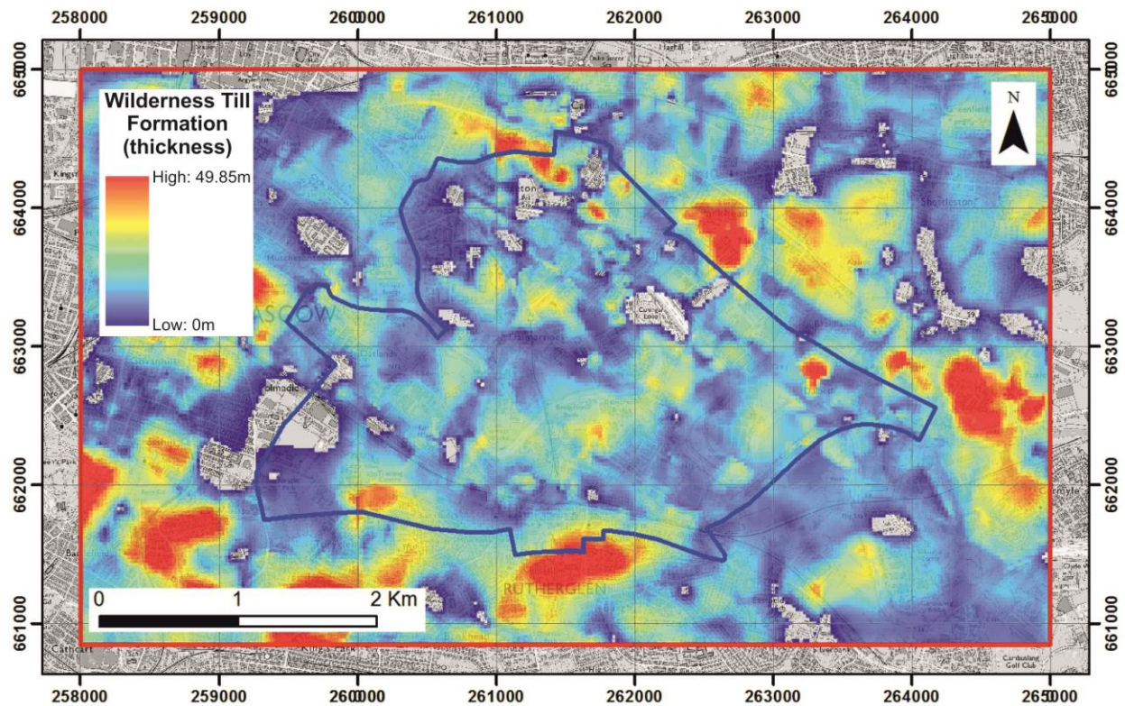
Figure 39 Modelled distribution and thickness of the Wilderness Till Formation (WITI) across the UKGEOS Glasgow superficial geology model area (red outline). This deposit of glacial till is widespread across the modelled area and beyond. It is thought to be almost 50 m thick in till-cored drumlins shaped by the over-riding Late Devensian glaciers. 1 km grid squares shown. Includes mapping data licensed from Ordnance Survey. © Crown Copyright and/or database right 2019. Licence number 100021290 EUL.
