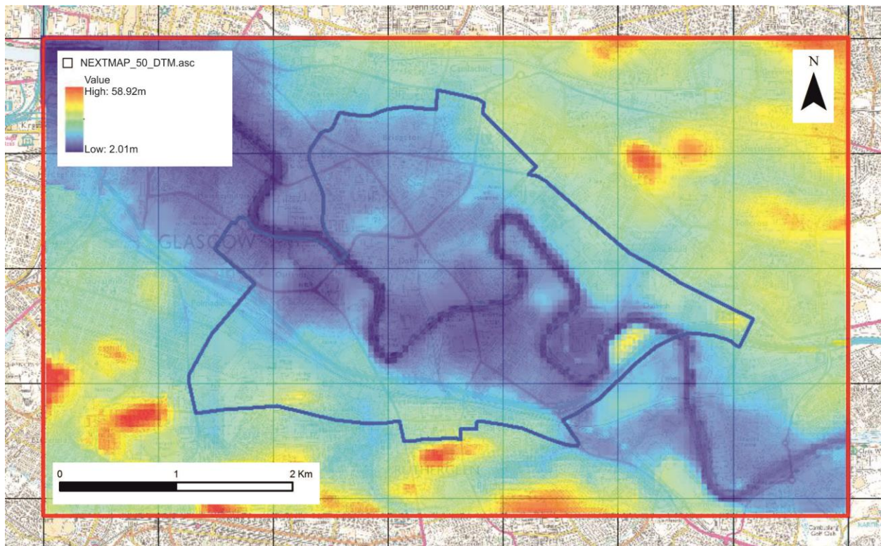
Figure 22 Digital Terrain Model (50 m cell size) across the UKGEOS Glasgow superficial deposits model area (red outline), as used in the model. NEXTMap Britain elevation data from Intermap Technologies. Includes mapping data licensed from Ordnance Survey. © Crown Copyright and/or database right 2019. Licence number 100021290 EUL.
