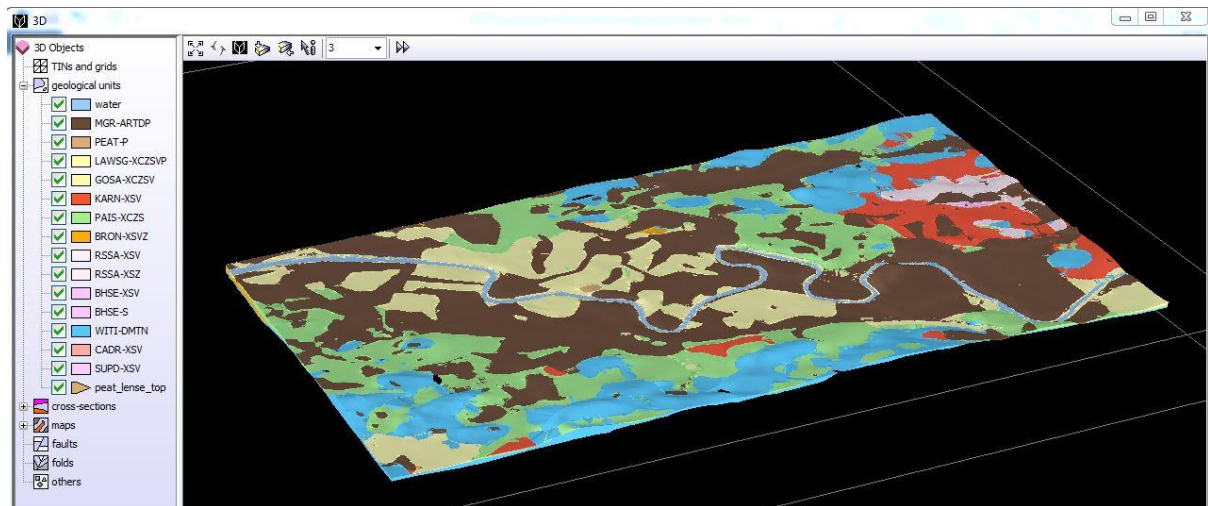
Figure 18 Overview of the calculated superficial deposits model across the UKGEOS Glasgow model area, looking north-east, 3x vertical exaggeration. NEXTMap Britain elevation data from Intermap Technologies.
