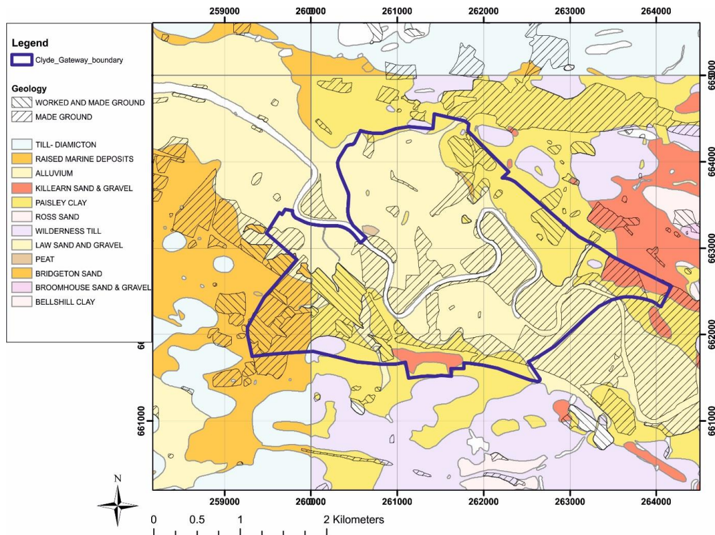
Figure 21 UKGEOS Glasgow model area summary of superficial geology from BGS©UKRI 2016 DigMap 1:10 000 scale data, the Clyde Gateway urban regeneration area is shown in blue.
