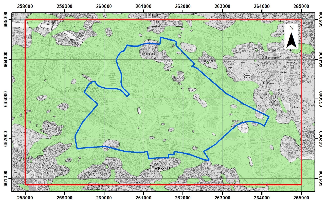
Figure 8: Modelled distribution of Paisley Clay Member (green) across the UKGEOS Glasgow superficial geology model area (red outline). 1 km grid squares shown. Includes mapping data licensed from Ordnance Survey. © Crown Copyright and/or database right 2019. Licence number 100021290 EUL).
