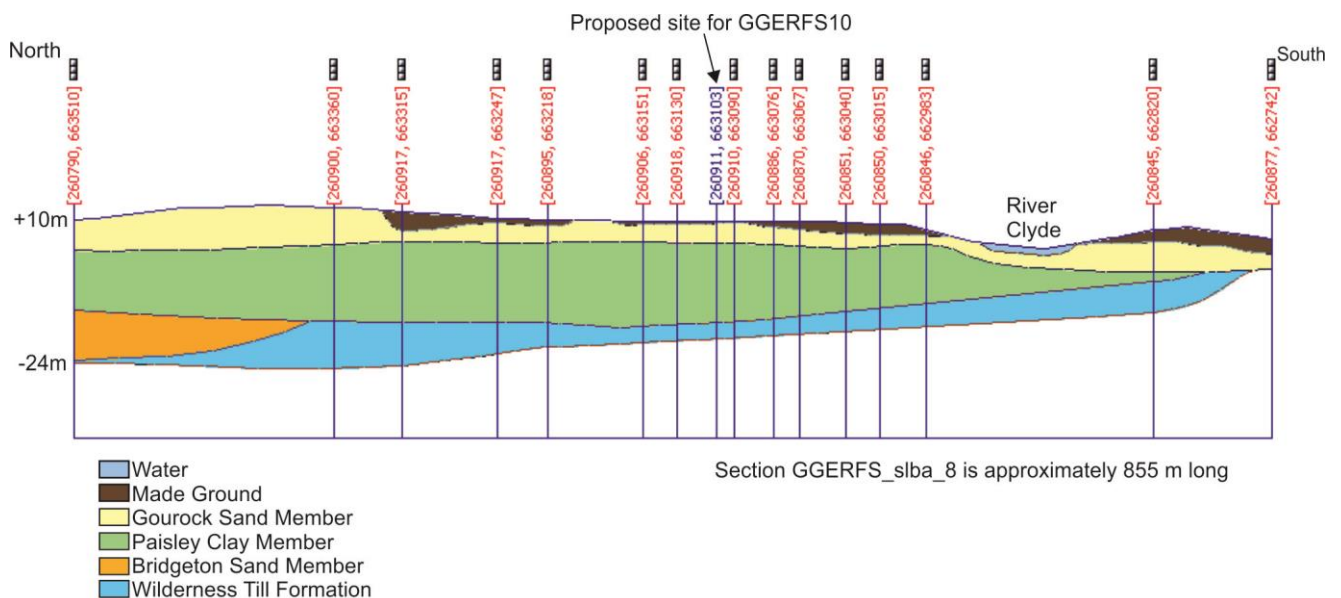
Figure 30 Cross-section GGERFS_slba_8 , orientated North-South through the superficial deposits of the UKGEOS Glasgow model area (see Figure 16 for location). Vertical exaggeration x 3. Borehole constraint points shown in red. Ground surface derived from NEXTMap Britain elevation data from Intermap Technologies. Height is in metres relative to Ordnance Datum.
