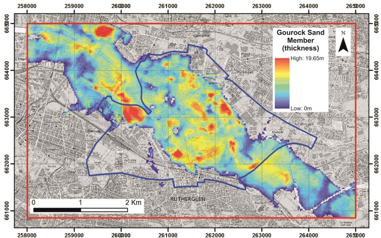
Figure 35 Modelled distribution and thickness of the Gourrock Sand Member (GOSA) across the UKGEOS Glasgow superficial geology model area (red outline). These marine sands are extensive within the Clyde Valley and are over 15 m thick in places. 1 km grid squares shown. Includes mapping data licensed from Ordnance Survey. © Crown Copyright and/or database right 2019. Licence number 100021290 EUL.
