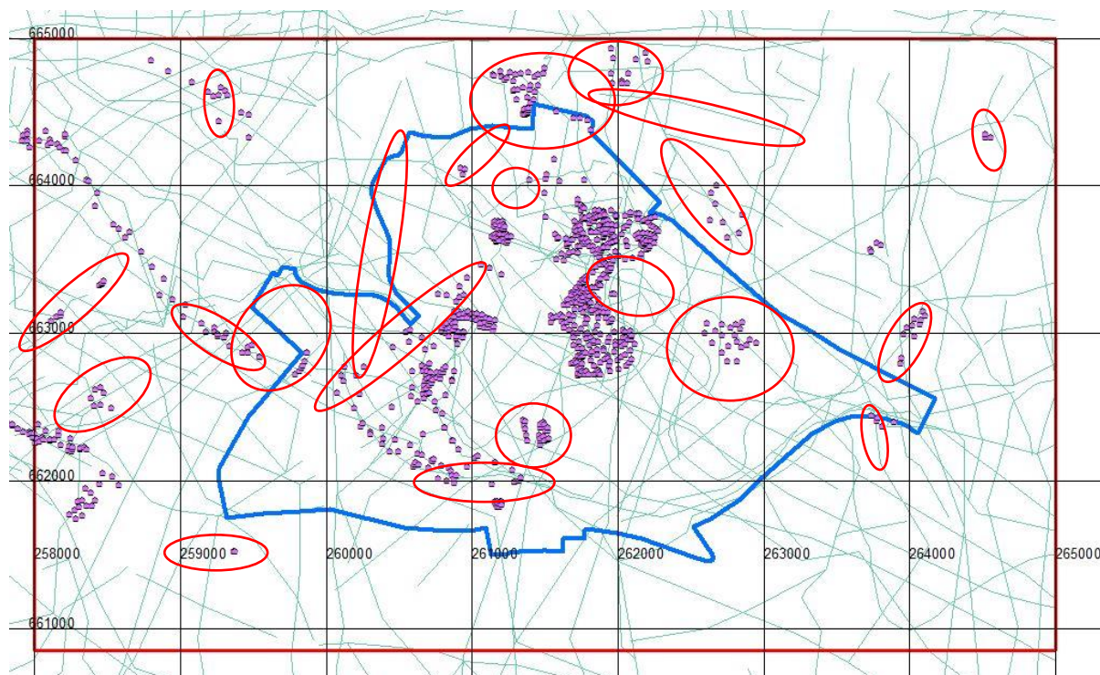
Figure 13 Areas circled in red show where the UKGEOS model was updated/improved during phase 1, green lines indicate existing GSI3D section lines from the published Central Glasgow model, purple dots represent the location of boreholes entered into the BGS borehole database post-2005.
