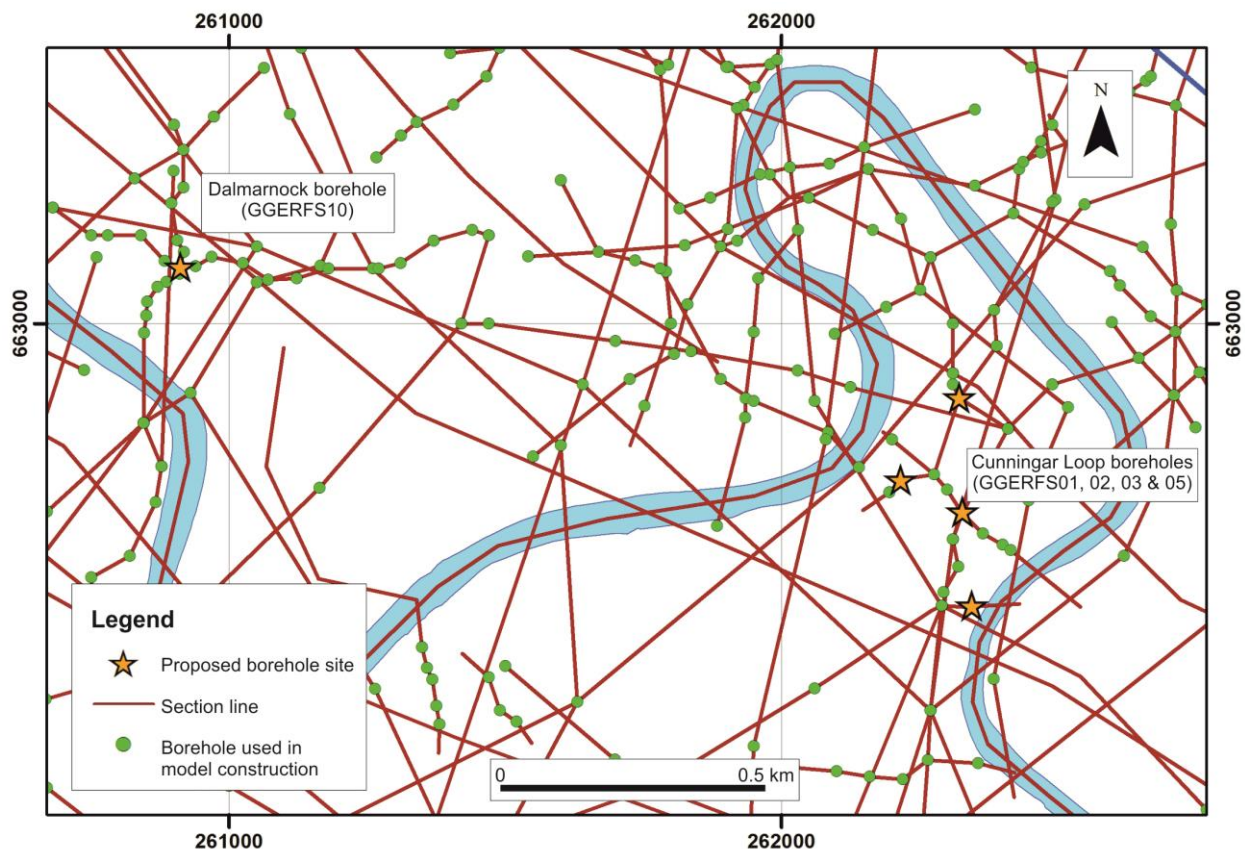
Figure 25 Distribution of boreholes used to construct the correlated cross-sections which constrain the superficial deposits model around the proposed borehole sites for the UKGEOS Glasgow project. The River Clyde is shown in pale blue.
