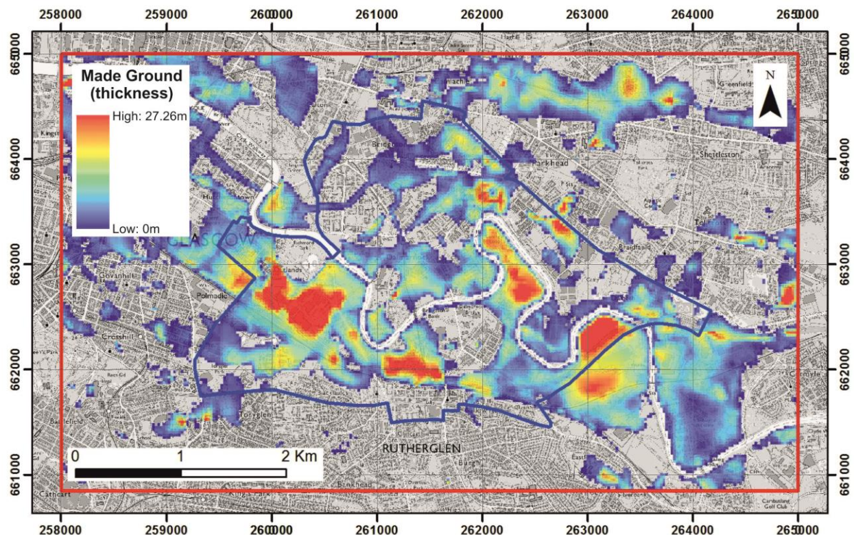
Figure 34 Modelled distribution and thickness of Made Ground deposits (MGR) across the UKGEOS Glasgow superficial geology model area (red outline). 1 km grid squares shown. Includes mapping data licensed from Ordnance Survey. © Crown Copyright and/or database right 2019. Licence number 100021290 EUL.
