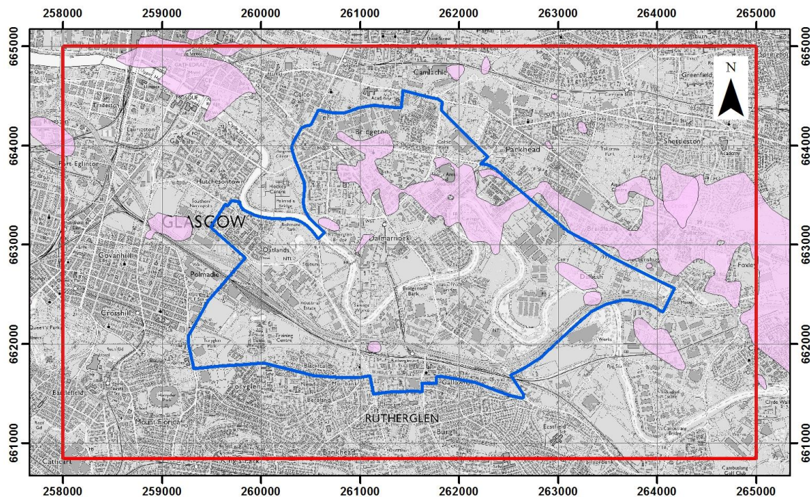
Figure 6: Modelled distribution of Broomhouse Sand and Gravel Formation (pink) across the UKGEOS Glasgow superficial geology model area (red outline). 1 km grid squares shown. Includes mapping data licensed from Ordnance Survey. © Crown Copyright and/or database right 2019. Licence number 100021290 EUL).
