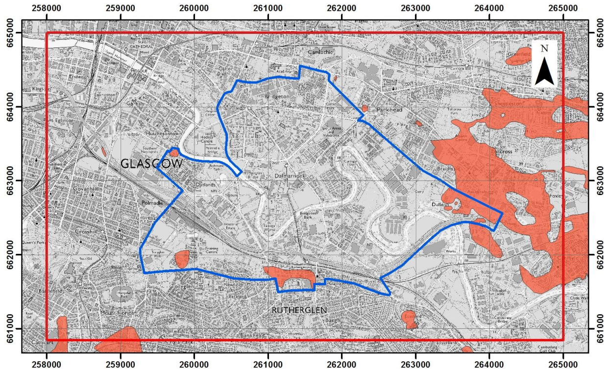
Figure 9: Modelled distribution of Killearn Sand and Gravel Member (red) across the UKGEOS Glasgow superficial geology model area (red outline). 1 km grid squares shown. Includes mapping data licensed from Ordnance Survey. © Crown Copyright and/or database right 2019. Licence number 100021290 EUL).
