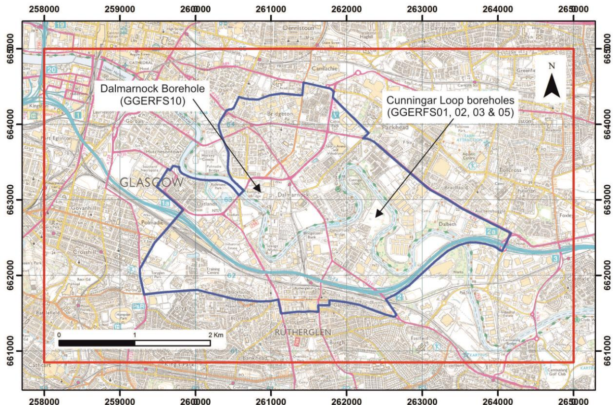
Figure 1 Location map of the Clyde Gateway regeneration area (blue outline) and GGERFS superficial model area (red outline) indicating the approximate location of the UKGEOS Glasgow boreholes. Includes mapping data licensed from Ordnance Survey. © Crown Copyright and/or database right 2019. Licence number 100021290 EUL.
