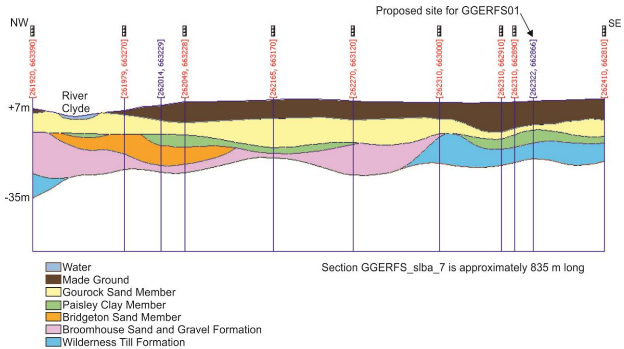
Figure 29 Cross-section GGERFS_slba_7 , orientated NW-SE through the superficial deposits of the UKGEOS Glasgow model area (see Figure 16 for location). Vertical exaggeration x 3. Borehole constraint points shown in red. Ground surface derived from NEXTMap Britain elevation data from Intermap Technologies. Height is in metres relative to Ordnance Datum.
