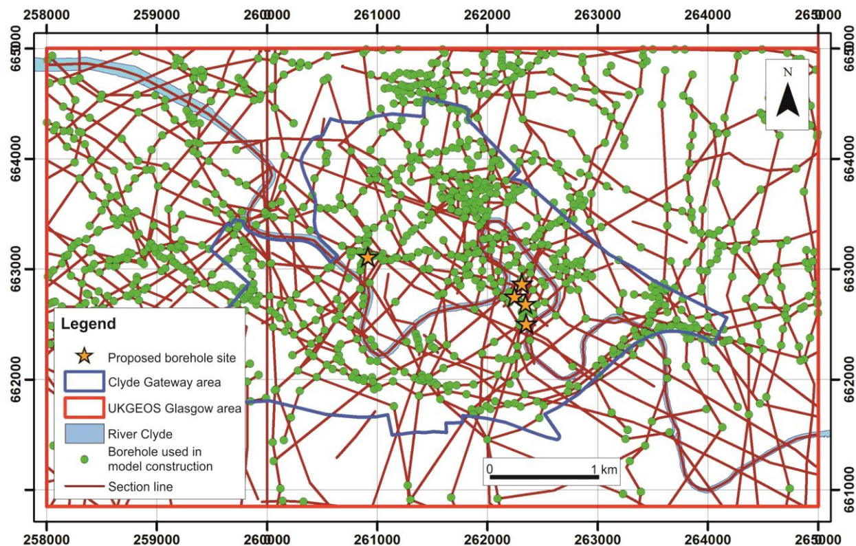
Figure 24 Distribution of boreholes used to construct the correlated cross-sections which constrain the superficial deposits model of the UKGEOS Glasgow area.
