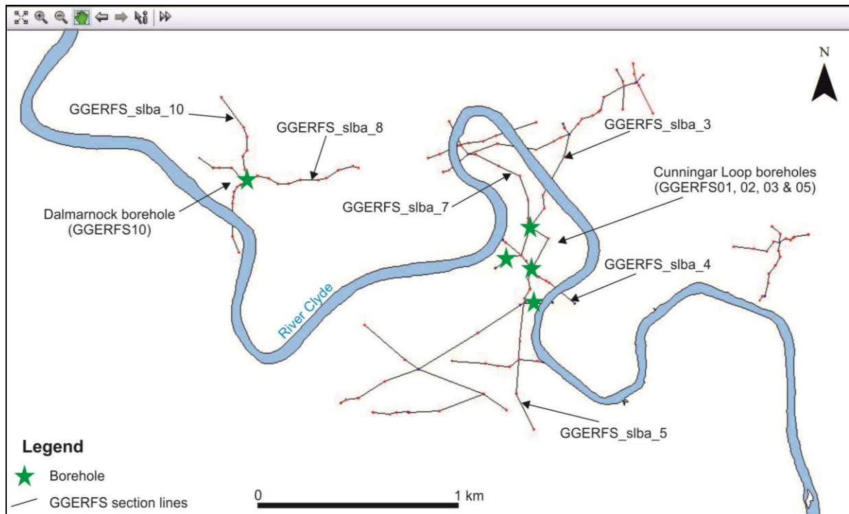
Figure 16 Summary map of proposed UKGEOS Glasgow borehole locations and sections constructed in GSI3D through the sites to indicate the nature and thickness of the superficial deposits beneath the surface.
