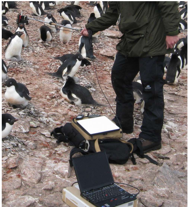
Fig. 3. Data collection. The sensor head is supported on a pole and alternately views the target and the Spectralon calibrator. The optical signal is carried by an optical fibre to the spectrometer (underneath Spectralon panel), which is controlled by the laptop computer.
