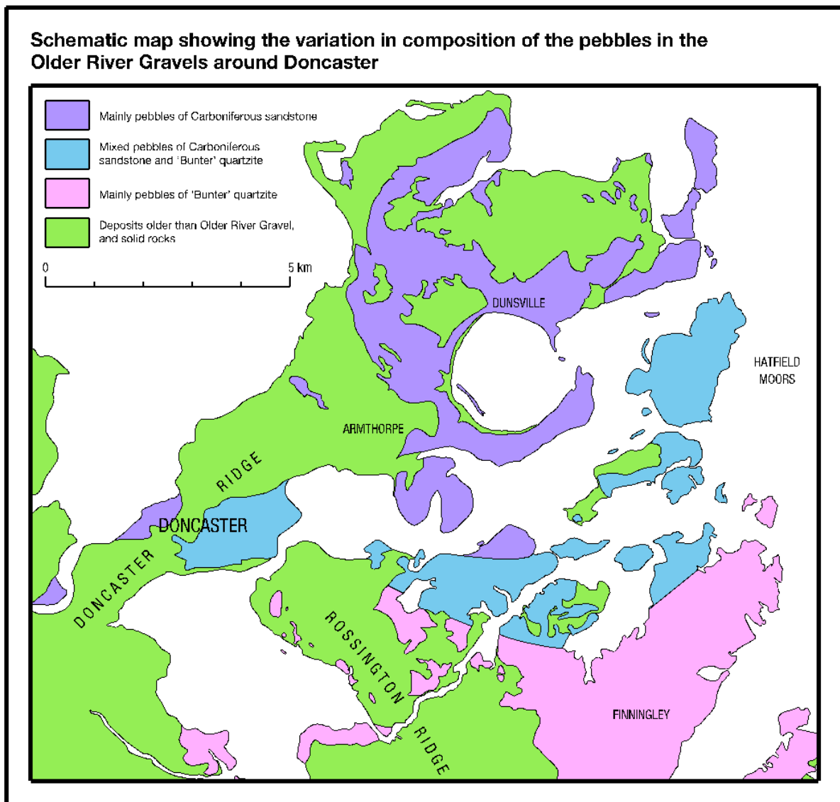
Schematic map showing the distribution of Older River Gravels deposits and their dominant pebble composition, fluvoglacial deposits and bedrock deposits. Uncoloured areas are non-mineral deposits
