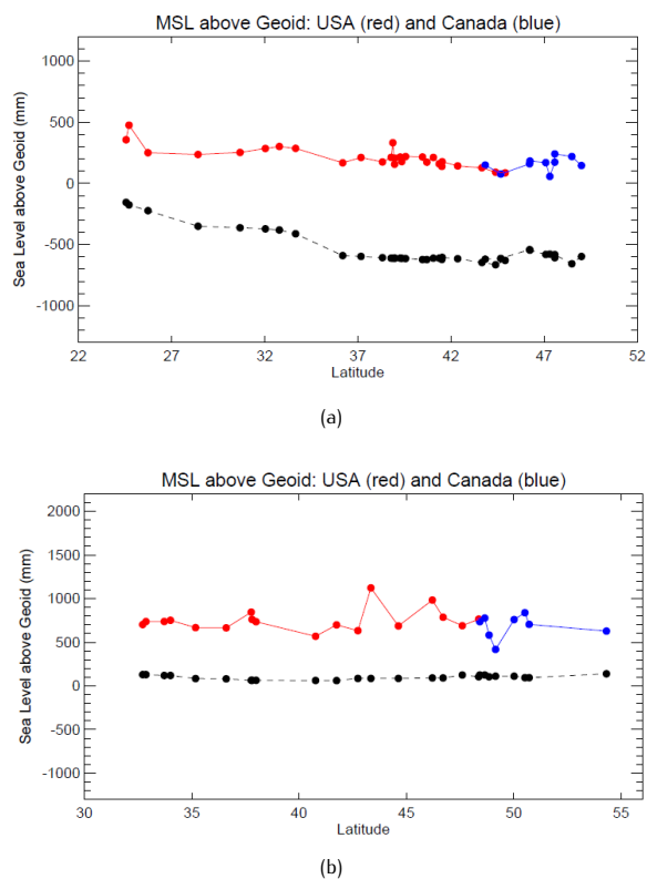
Figure 4. Equivalent information to Figure 3(a,b) but using the Extended GOCO03S geoid model.
