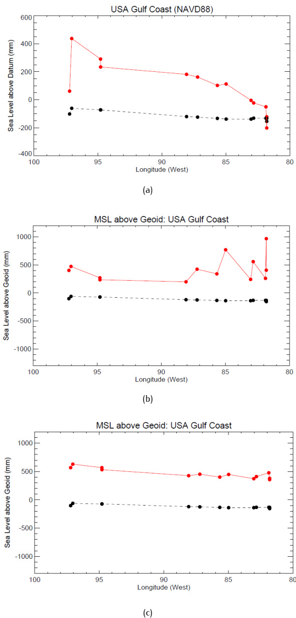
Figure 5. Corresponding information for the Gulf coastline. (a) MSL with respect to NAVD88, (b) geocentric MSL with respect to GOCO03S, and (c) geocentric MSL with respect to the Extended GOCO03S geoid model. Note that Key West has been included in Figures 2(a), 3(a), 4(a) and the present figure so as to provide a link between the Atlantic and Gulf coastlines.
