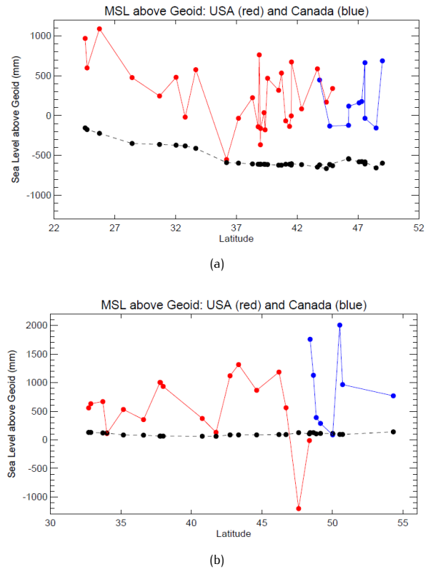
Figure 3. (a) As Figure 2(a) but with values of MSL determined as geocentric heights above the reference ellipsoid and are shown relative to values of the geoid from the GOCO03S model. (b) A similar set of points for the Pacific coast of North America.
