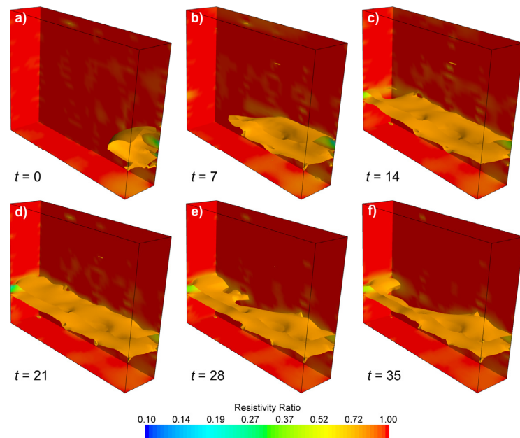
Figure 4. Evolution of the conductive tracer visualised in 3D at discrete times t (days). The isosurface ratio = 0.79.
