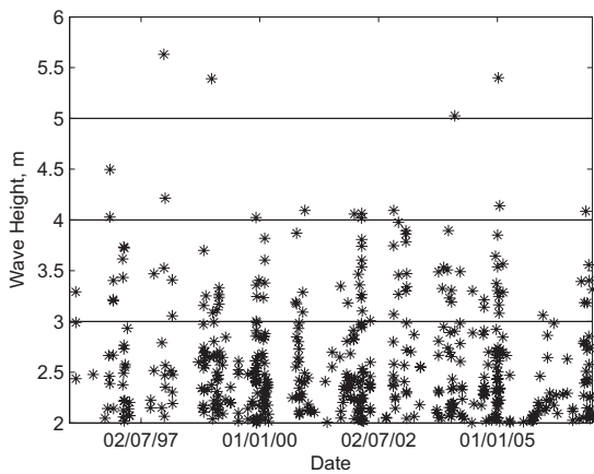
Fig. 7. Wave height greater than 2m over the past 11-years, obtained from model hindcast data due to limited observations (02/10/02 onwards).
