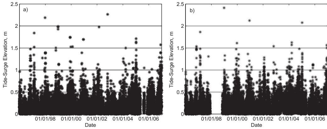
Fig. 5. The (positive) peak surge residuals, due to tide-surge interaction, over the past 11-years, obtained from tide gauge data at a) Liverpool and b) Heysham.
