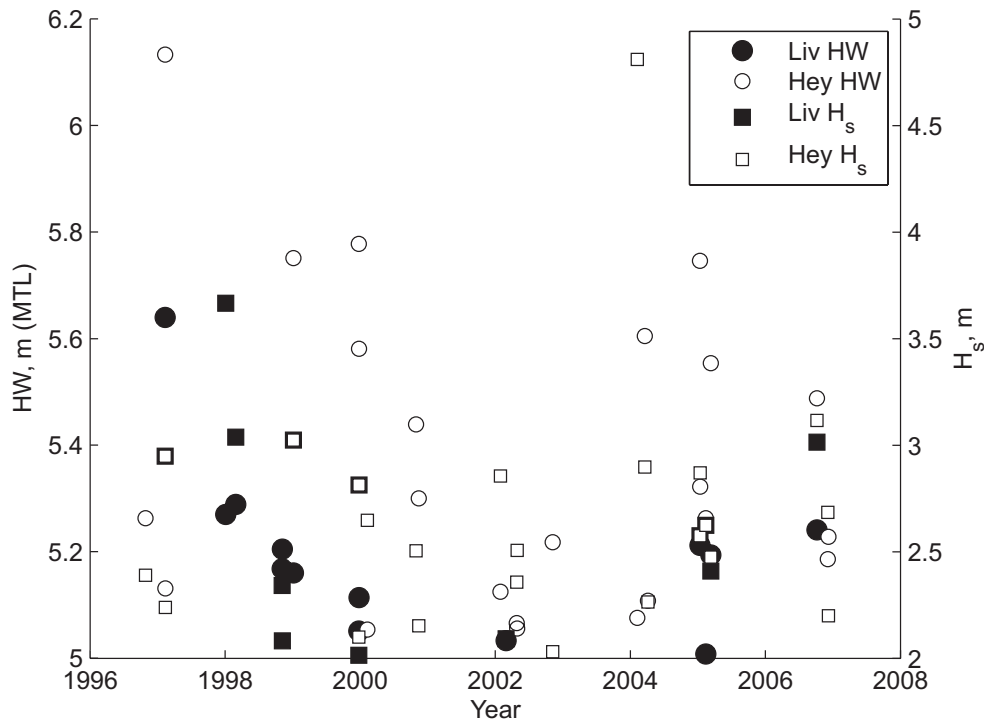
Fig. 8. Periods of coincidental extreme water levels and wave events. Observed high water (HW) levels exceeding 5m at Liverpool and Heysham, with modelled offshore wave heights ( H_s ) exceeding 2m at the wave buoy location, coincidental with HW at one of the ports.
