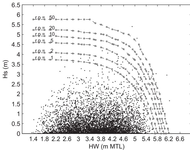
Fig. 10. Wave heights ( H_s ) during high water (HW) at Heysham during 1996 – 2006. The contours show the equal joint exceedance probability for a range return periods (r. p.), predicted by the JOIN-SEA software.
