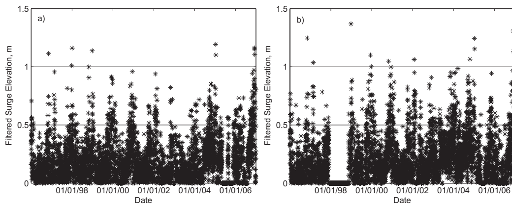
Fig. 4. The (positive) peak filtered surge residuals, due to the meteorological forcing alone, over the past 11-years, obtained from tide gauge data at a) Liverpool and b) Heysham.
