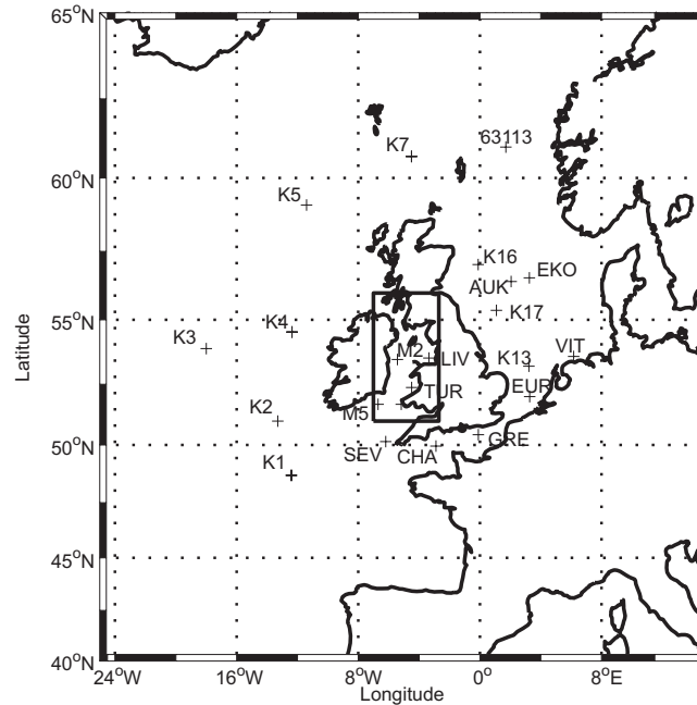
Fig. 2. The nested WAM model domains and the locations of the wave buoys and offshore platforms used for validation. The outer boundary of the figure represents the northeast Atlantic model and the inner rectangular box represents the Irish Sea model boundary.
