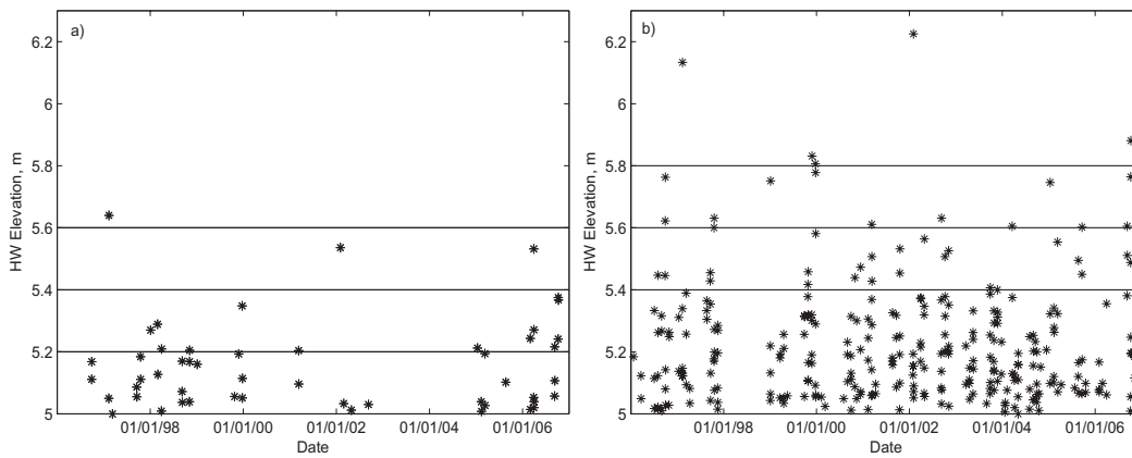
Fig. 6. High water elevations (above MTL) greater than 5m over the past 11-years, obtained from tide gauge data at a) Liverpool and b) Heysham.
