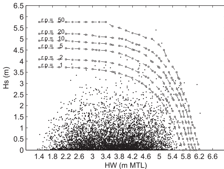
Fig. 9. Wave heights ( H_s ) during high water (HW) at Liverpool during 1996 – 2006. The contours show the equal joint exceedance probability for a range return periods (r. p.), predicted by the JOIN-SEA software.
