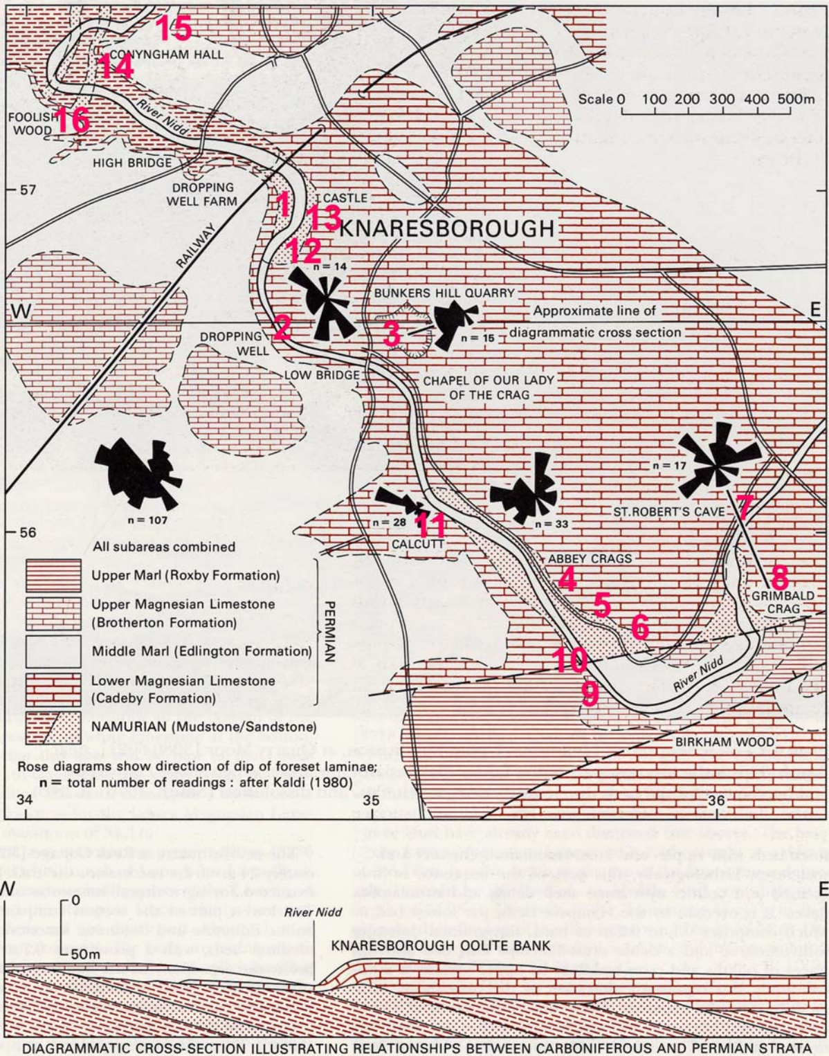
Geological map and cross-section of the Knaresborough area (with palaeocurrent information from Dr J.G.Kaldi) after Cooper and Burgess, 1993
