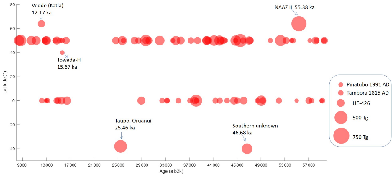
Figure 6. Schematic of the latitudinal location for the identified bipolar volcanic eruptions (Table S5). Volcanoes for which the eruption site is predicted above 40^\circ \text{ N} are marked at 50^\circ \text{ N} , and those predicted below 40^\circ \text{ N} are marked at the Equator. Volcanic locations that are known from ice-core tephra deposits are indicated by name and age of the eruption (Table S5). Due to its high relative sulfate deposition in Antarctica, the eruption at 46.68 ka, marked at 40^\circ \text{ S} in the figure, is very likely from the Southern Hemisphere, but the eruption site is unknown. The size of the circles represents the strength of volcanic stratospheric aerosol loading.
