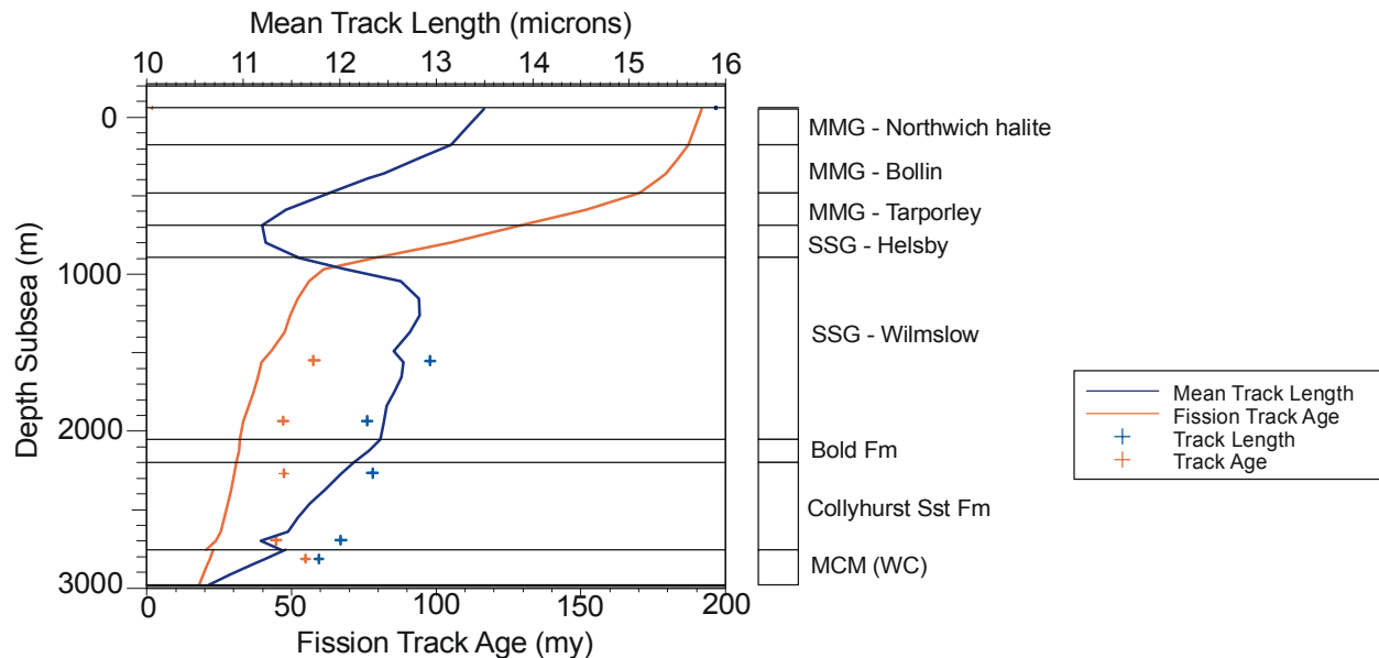
Figure 5d; Apatite Fission Track data and model from Knutsford Borehole.
