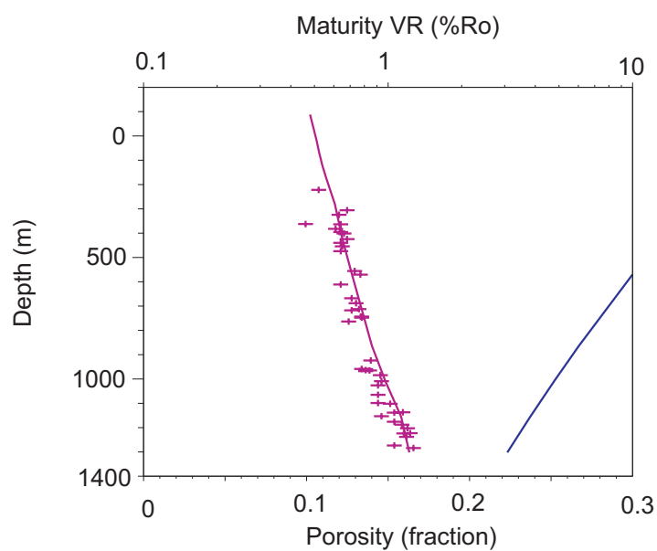
Figure 6d; Present day maturity in Pie Rough Borehole
