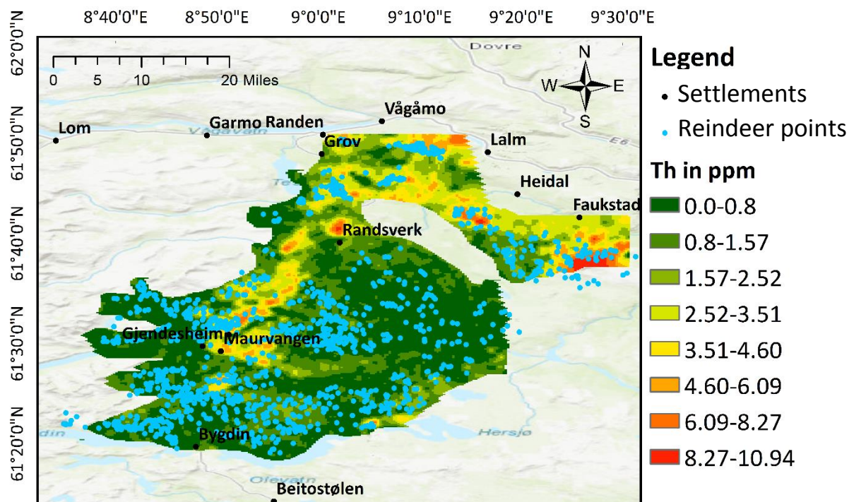
Figure 3 (c). GPS tracking locations over 11 months for an example (and typical) reindeer (Frigg) overlaid on soil Th concentrations
