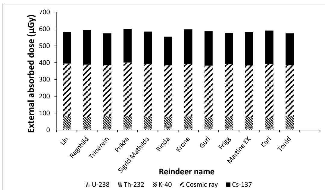
Figure 2. External doses of twelve Norwegian reindeers over 11 months calculated using the radionuclide activity concentrations in soil, cosmic exposures (estimated from altitude) and GPS tracking data.
