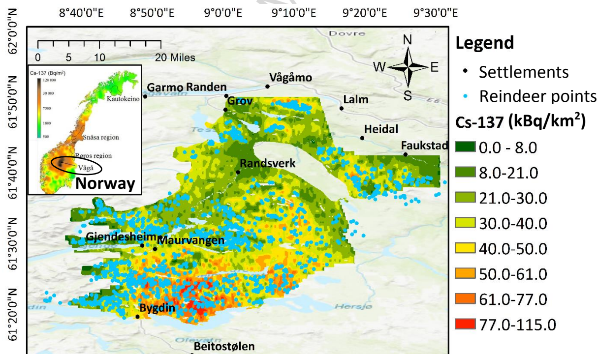
Figure 3 (a). GPS tracking locations over 11 months for an example (and typical) reindeer (Frigg) overlaid on ^{137}\text{Cs} activity deposition in Vågå (sources for the GIS base map: Esri, HERE, Delorme, Intermap, increment P Corp., GEBCO, USGS, FAO, NPS, NRCAN, GeoBase, IGN,
