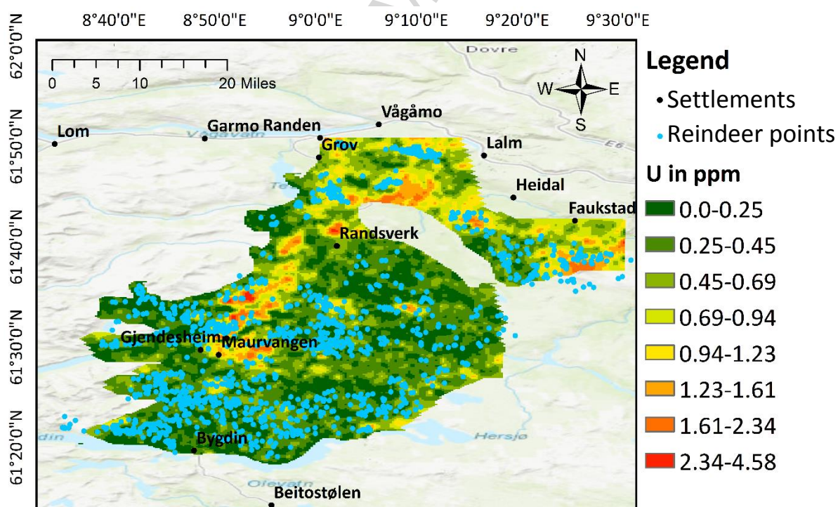
Figure 3 (d). GPS tracking locations over 11 months for an example (and typical) reindeer (Frigg) overlaid on soil U concentrations
