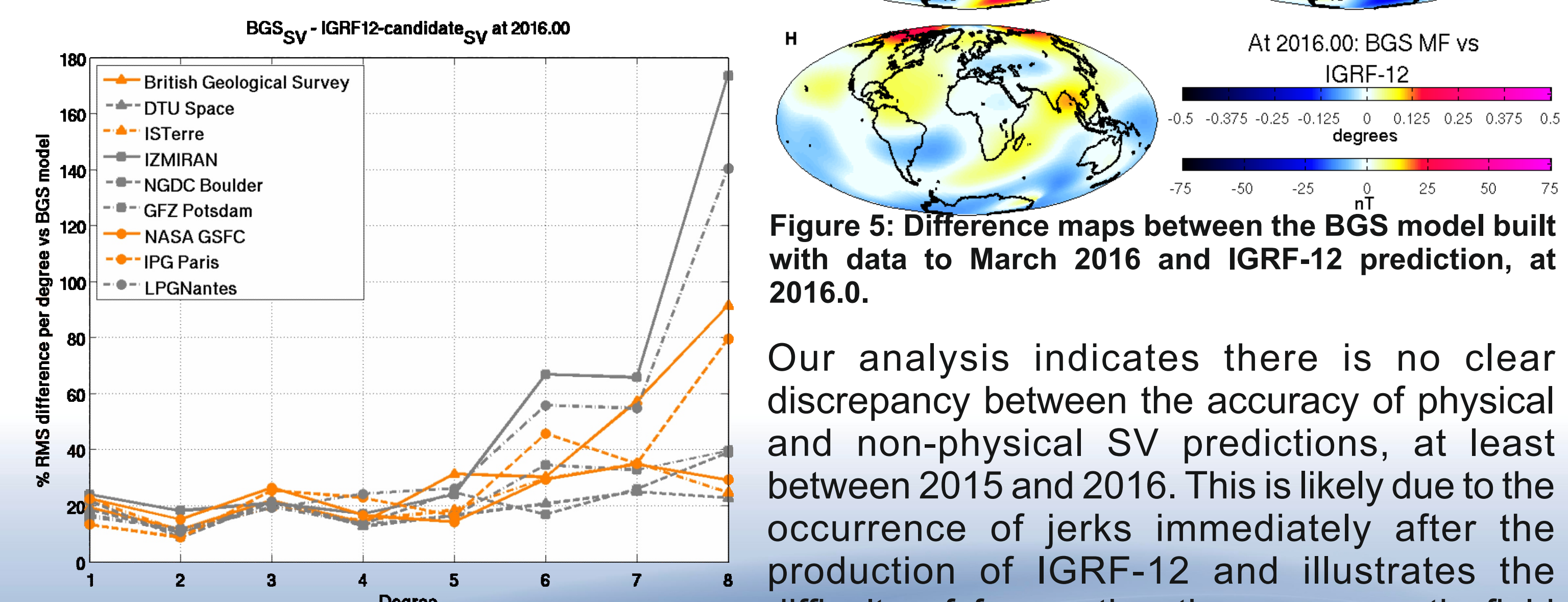
Figure 6: Percentage difference per degree for the 9 IGRF-12 SV candidates and the new BGS model, at 2016.0. Candidates with physically derived SV predictions in orange, mathematically extrapolated SV models in grey.
