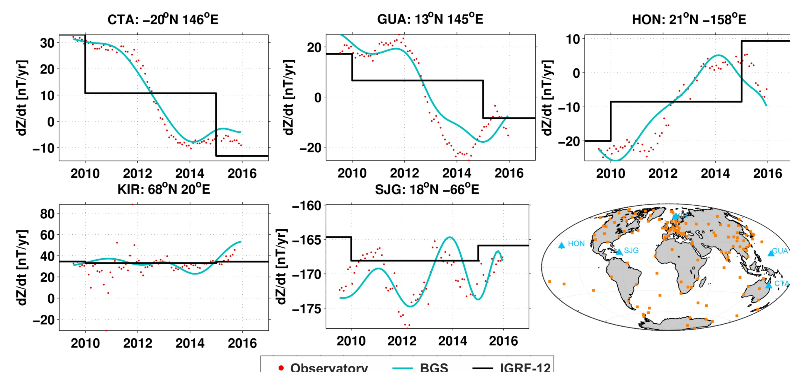
Figure 4: Z-component of SV data and models at Charters Towers (CTA), Guam (GUA), Honolulu (HON), Kiruna (KIR) and San Juan (SJG). GUA and SJG indicate that a newer jerk occurred in 2015, further illustrating the unpredictable and rapid nature of such SV. Map shows observatories currently operating.
