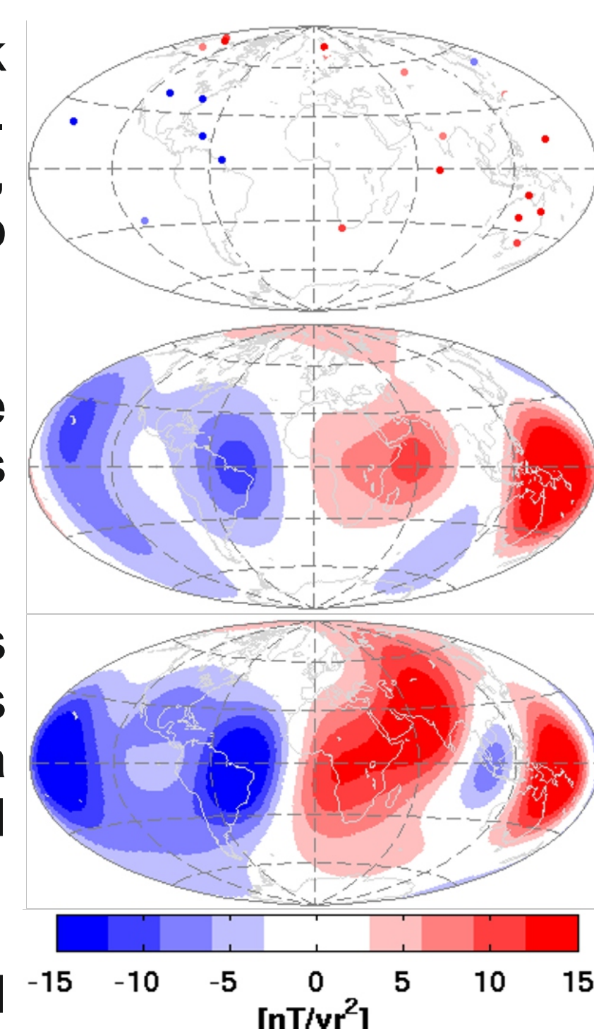
Figure 3: Detected (top) and modelled (middle) 2014 jerk amplitudes with estimated \Delta SA from CHAOS-6 model (bottom).
