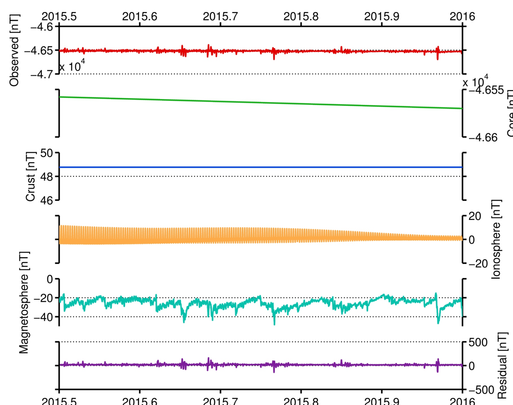
Figure 2: Separated field sources from an example observatory timeseries (radial component, Eskdalemuir, Scotland) using a BGS field model created from Swarm and AUX_OBS_2 data, CM4 and CHAOS-6.
