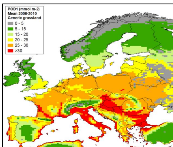
Figure 4.1. Phytotoxic ozone dose (POD 1 ) for grass per 0.5° x 0.25° grid, accumulated over a six months period (April – September) and averaged for 2006 – 2010.
