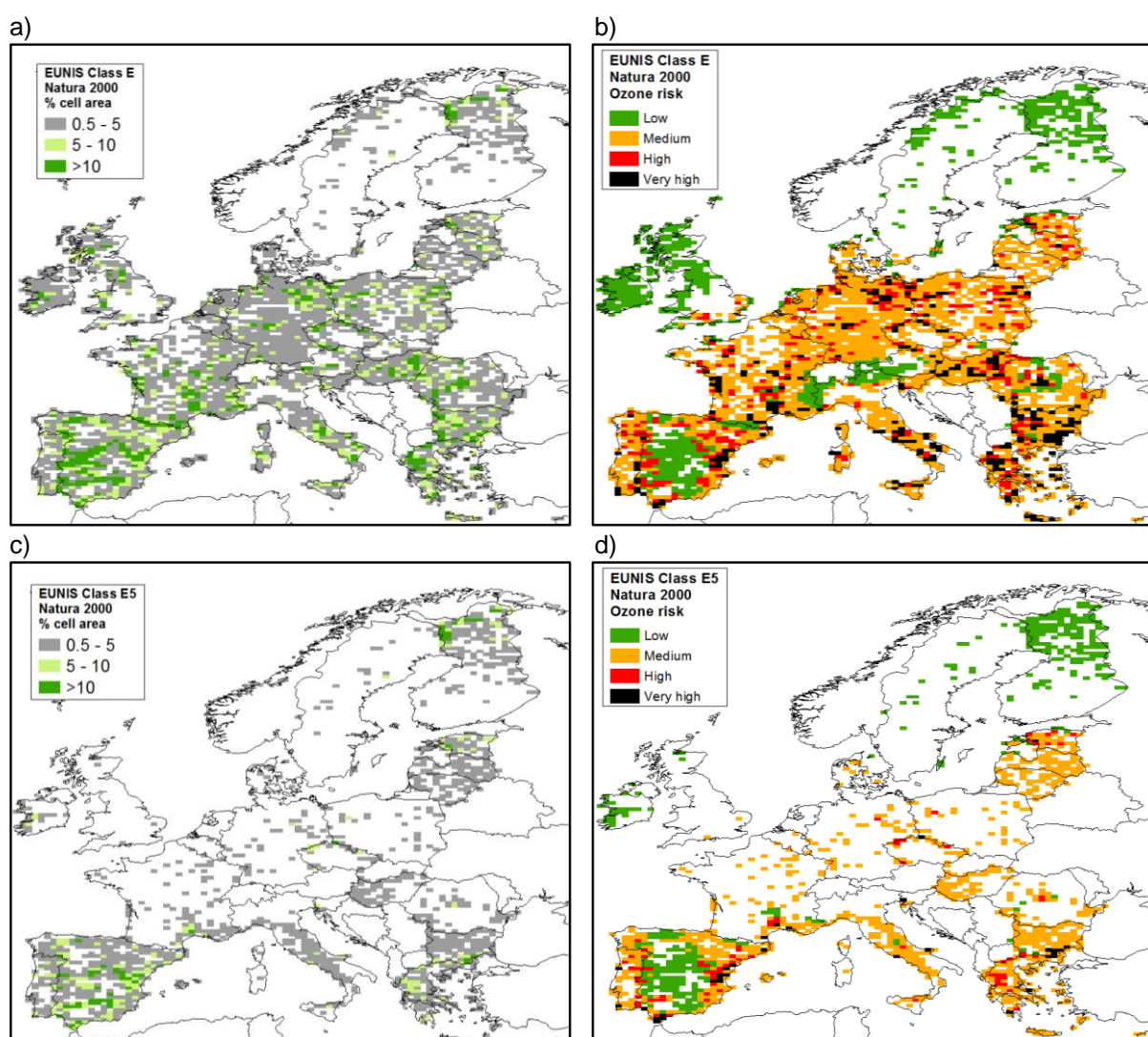
Figure 4.2. Percentage area (a, c) of grasslands (a) and woodland fringes (c) per 0.5° x 0.25° grid and the risk of ozone impact (b, d) on grasslands (b) and woodland fringes (d) in Natura 2000 areas.
