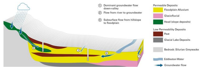
Conceptual model of groundwater flow in the floodplain aquifer, showing hillslope/river inflows
