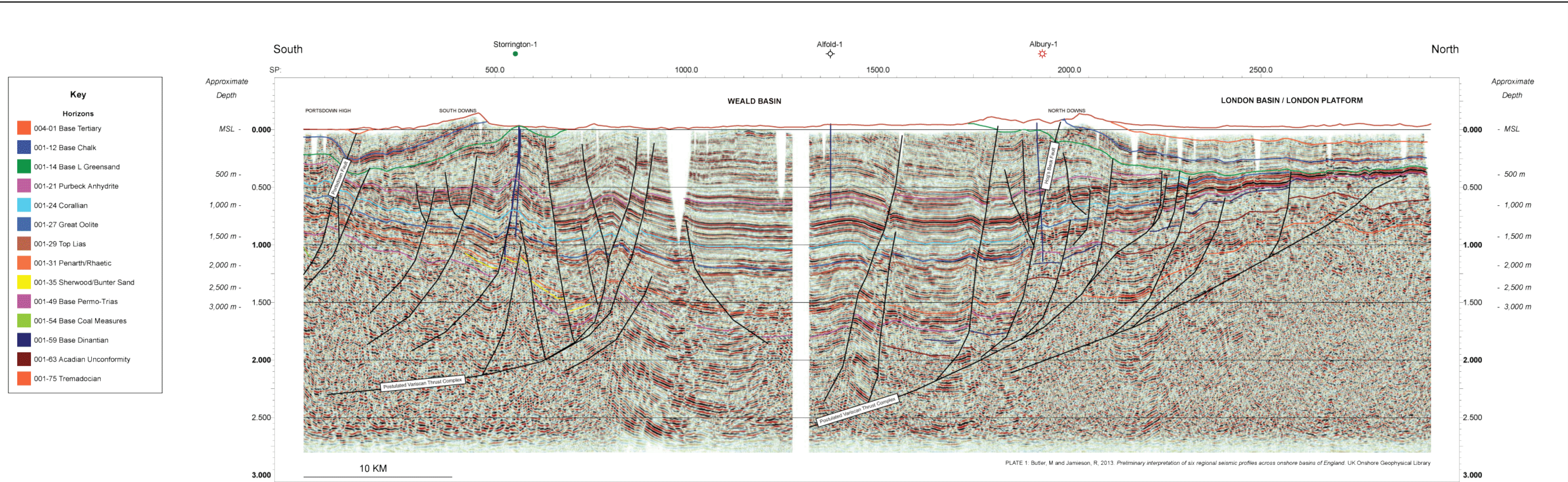
Figure 19. Regional 2D seismic line UKOGL-RG-001 across the central Weald Basin (from Butler & Jamieson 2013). See Figure 12 for location.
