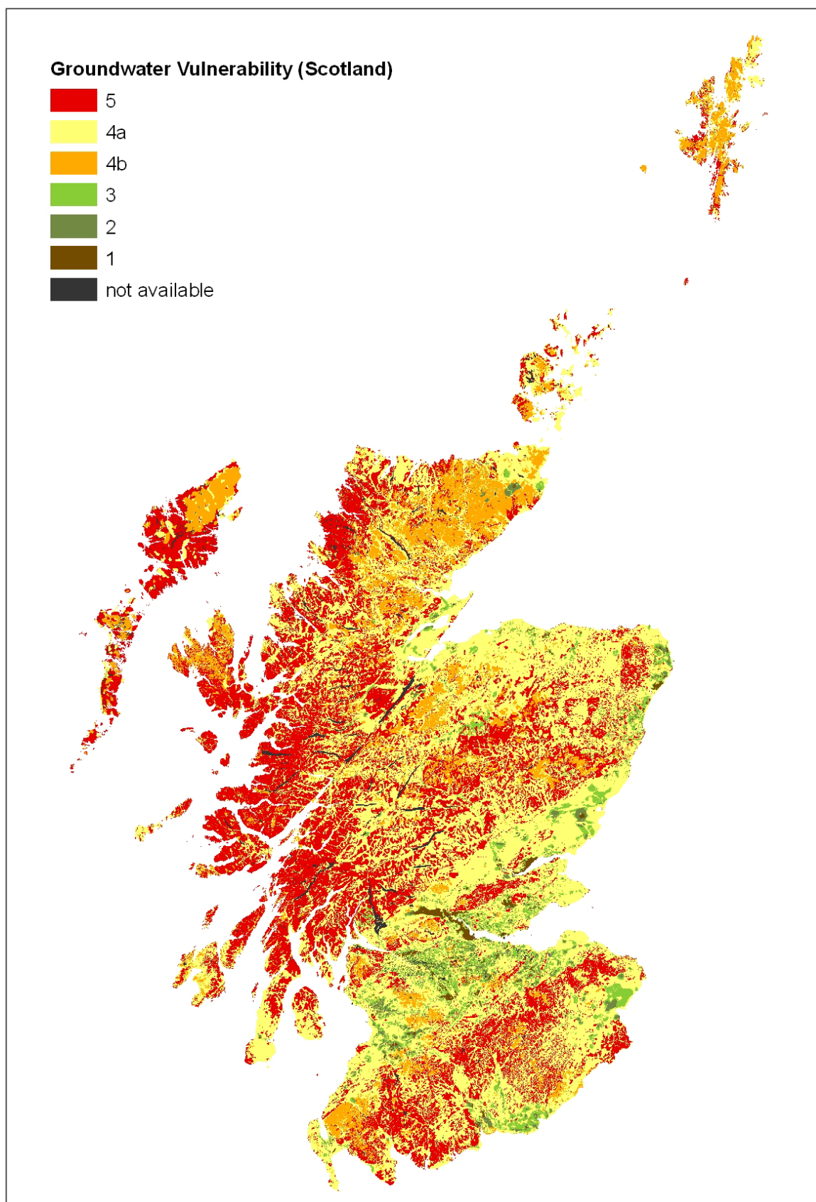
Figure 1 The groundwater vulnerability (Scotland) map, Version 2
