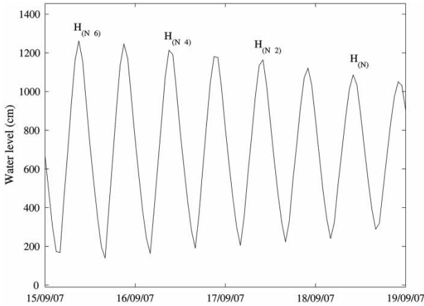
Figure 2. Example of the indexing of HW employed by the Empirical Correction Method, using hourly sampled data from the Avonmouth tide gauge.
