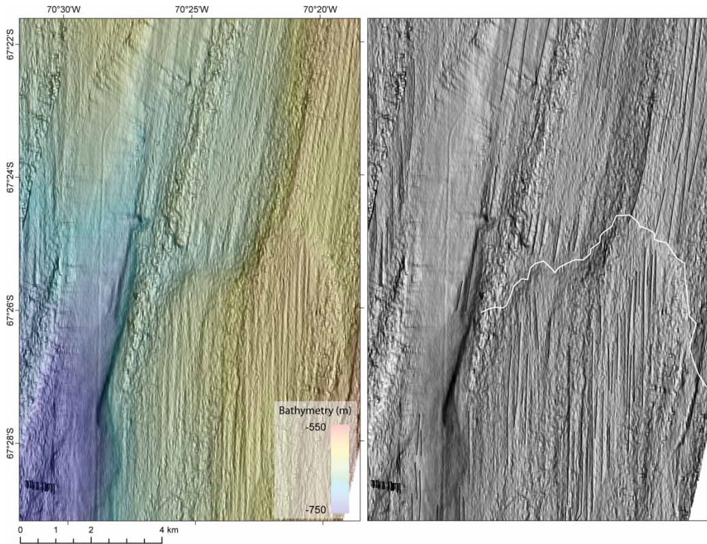
Figure 7. Example of grounding zone wedge on the outer shelf. Note the subtle difference in orientation of the MSGs either side of the wedge crest (white line). The left-hand panel is the relief-shaded image and the right-hand panel shows the mapped landforms (colours are the same as in the main map). The relief-shaded image is x20 exaggeration and is shaded from the NE.
