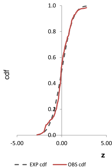
Fig. 2. Cumulative distribution function for the natural logarithms of the shrub Cs CR_{wo-media} dataset ( N = 354 ). OBS cdf = observed cdf; EXP cdf = expected cdf for a lognormal distribution.
