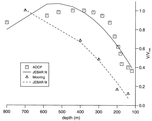
Figure 10. The JEBAR functional fit, as specified in equation (11) to depth-averaged velocity data, where the velocity has been normalised by the sectional maxima. Original ADCP data for section HA are indicated by squares and solid line represents the fit; while the mean normalised velocities from the mooring deployments are indicated by triangles and their fit by the dashed line.
