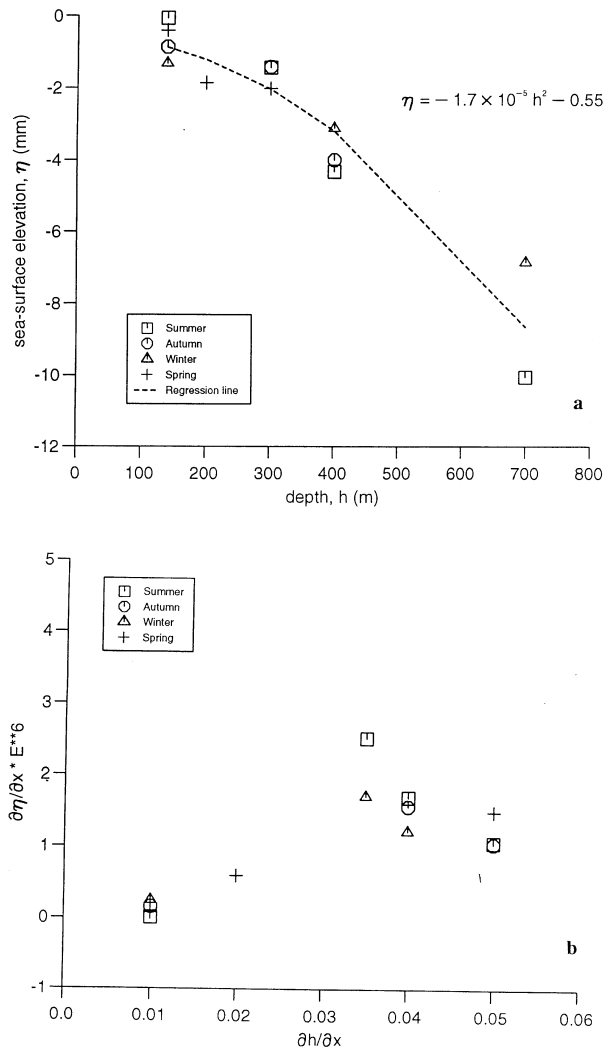
Figure 9. Sea surface topography on S line derived from barotropic geostrophic approximation. a) Elevation versus depth; b) surface gradient (barotropic geostrophic velocity) versus bottom slope.
