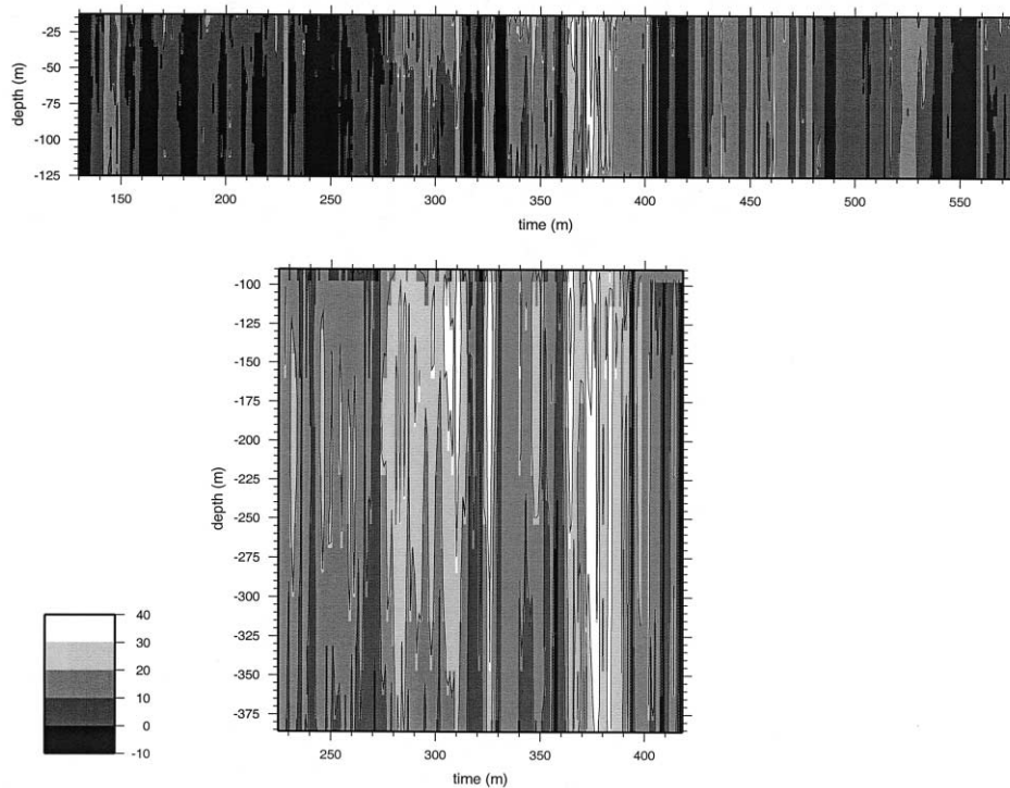
Figure 6. Time series of along-slope current from bottom mounted ADCP. (a) S140; (b) S400.
