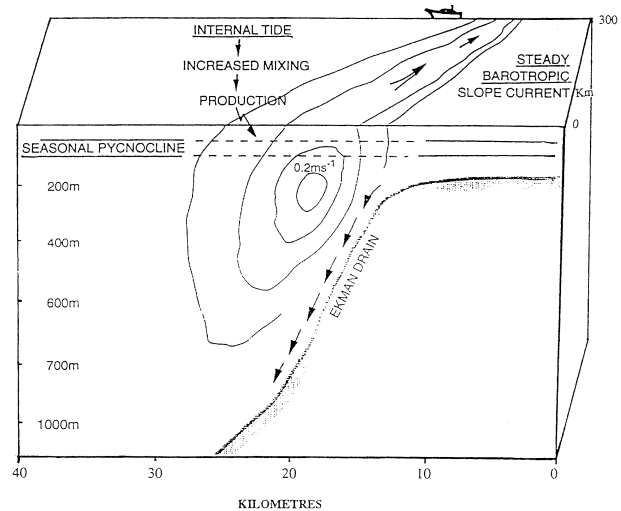
Figure 13. Schematic of the slope current, showing the principal features observed: the steady barotropic slope current and associated Ekman draining generated by the bottom stress of the current.
