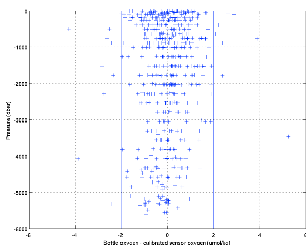
Figure 2.6: Offsets from the bottle oxygen minus calibrated CTD sensor oxygen. Vertical blue lines indicate a \pm 2 \mu\text{mol/kg} offset range.
