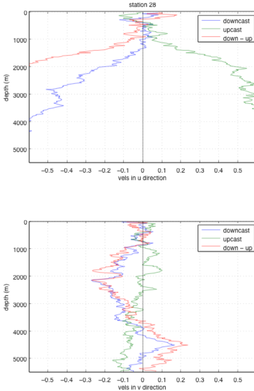
Figure 8.2: example output from shearcheck , for station 28. The upcast and downcast u velocities diverge markedly below 1000m. The behaviour of the v velocities is less obviously bad, but the divergence below 1000 m is still indicative of poor quality data, even though they converge at greater depth.
