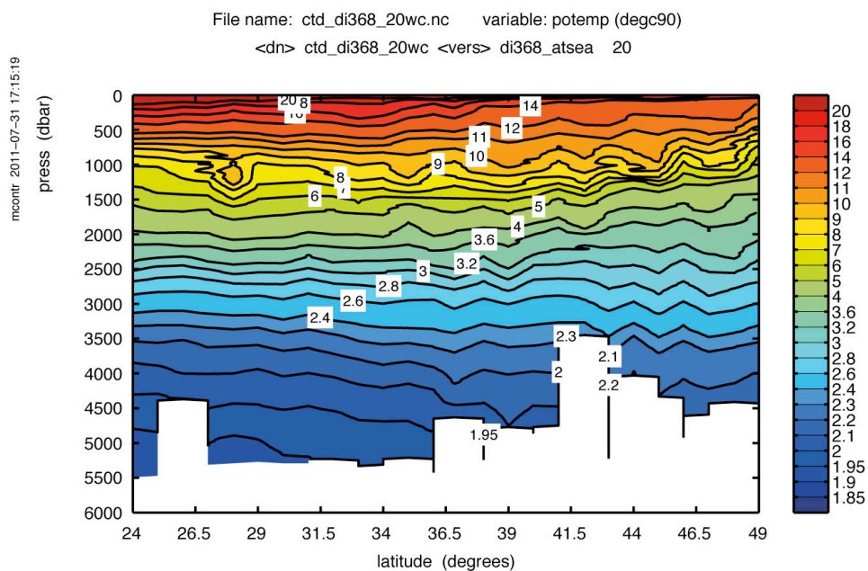
Figure 2.1 Potential Temperature for the A16N section of the survey (stations 2 to 28), recorded at 1° latitude spacing and binned in 20 dbar, white areas indicate where data were not collected.
