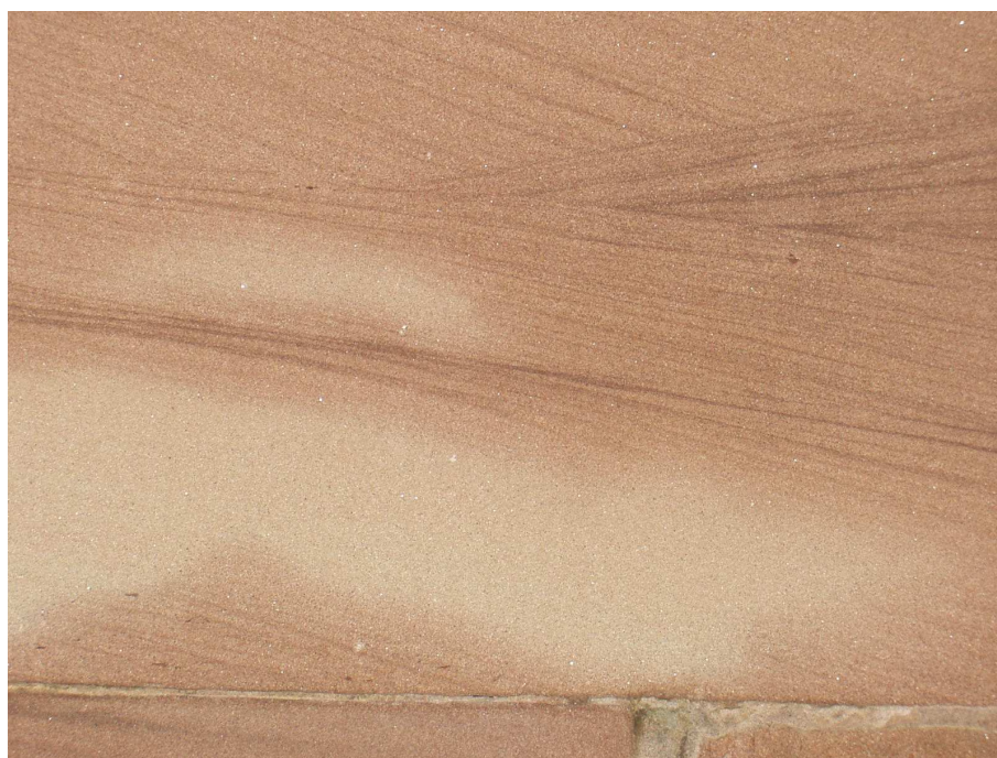
Figure 3.7. Detail of cross-bedding in the Sherwood Sandstone showing variation in iron-oxide concentration and possibly redox condition (red/yellow coloration) from a stone wall, Beckbury Church [SJ 764 016] (photograph: I. Neumann).
