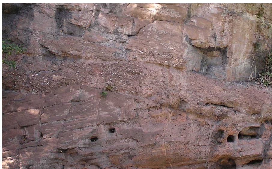
Figure 3.6. Outcrop showing detail of dune-bedded Bridgnorth Sandstone cross-bedded with fluvial Kidderminster Conglomerate [SO 733 959] (photograph: S. Brown).
