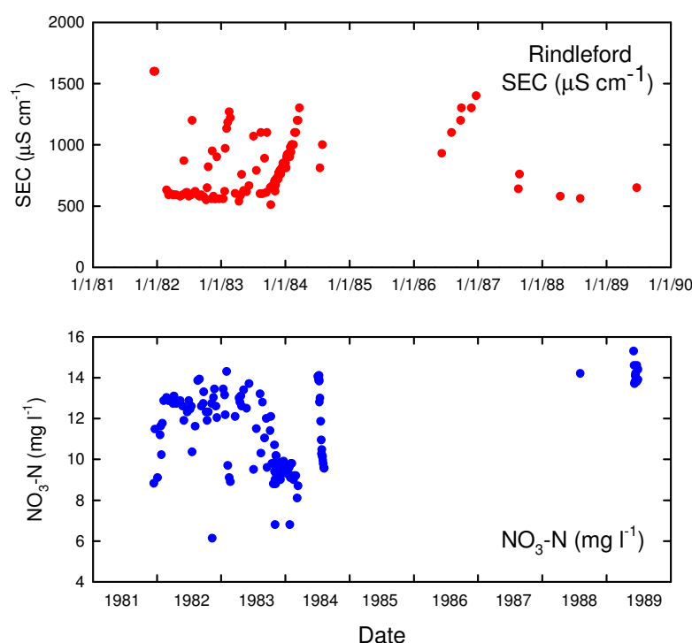
Figure 6.14. Temporal variation in SEC and NO 3 -N concentration in a borehole at Rindleford [SO 738 956].
