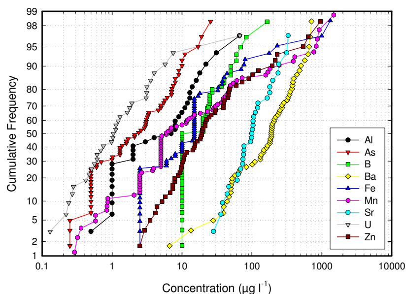
Figure 5.5. Cumulative-frequency plots for the minor constituents in groundwaters from the Shropshire Permo-Triassic Sandstone.
