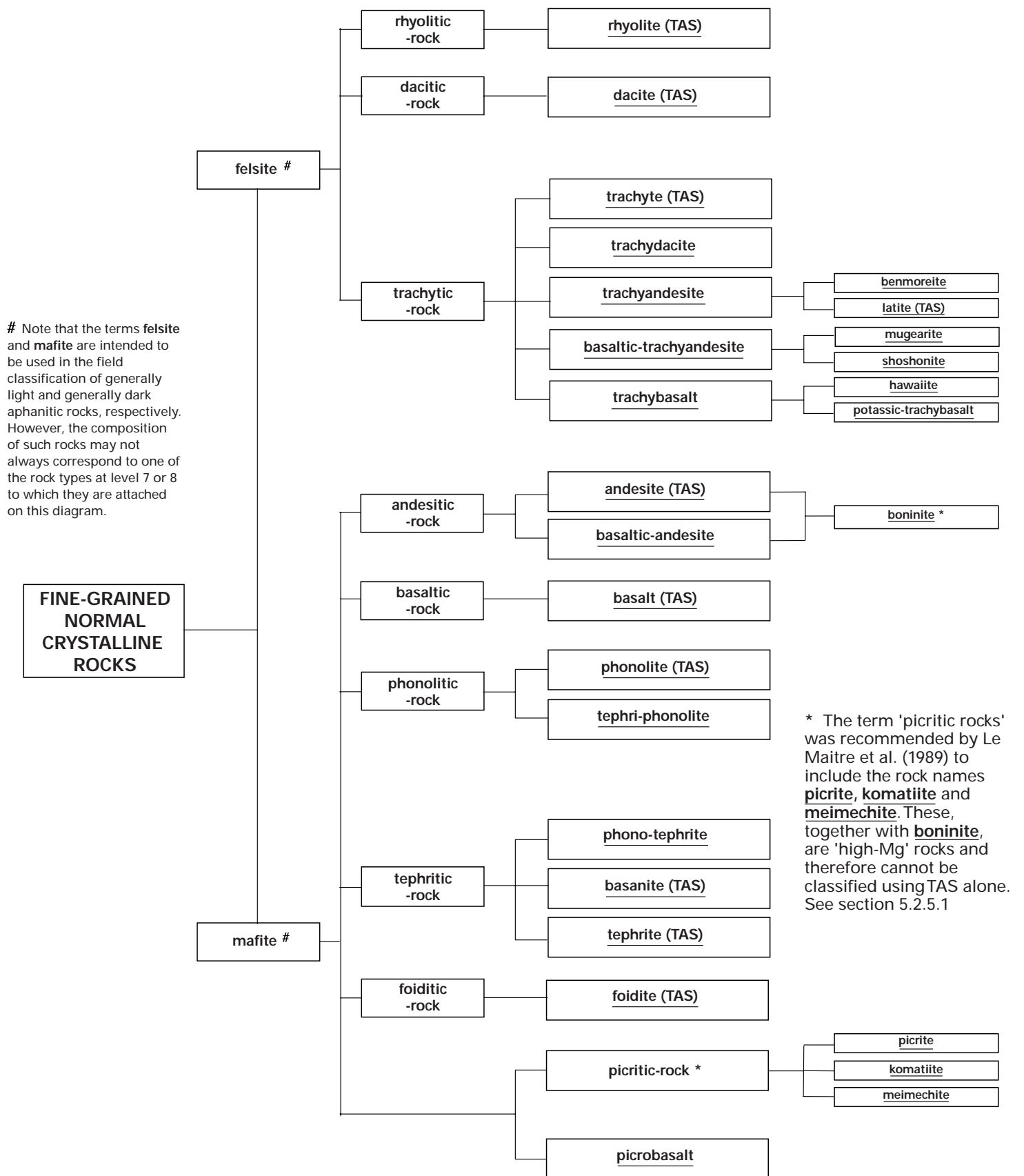
Figure 17b Hierarchical classification of fine-grained normal crystalline rocks with TAS classification at levels 8 and 9.
