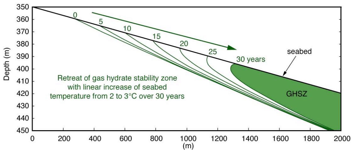
Aux Fig. 1. The retreat of the gas hydrate stability zone in response to a gradual increase of water-bottom temperature 1 °C over a 30 year period. Seabed: black. Boundary of the hydrate stability zone at 5-year intervals: green.
