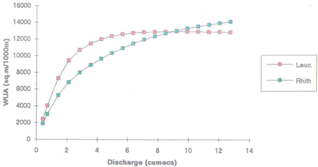
Figure 7.3 Habitat vs Discharge Relationships : River Hodder
