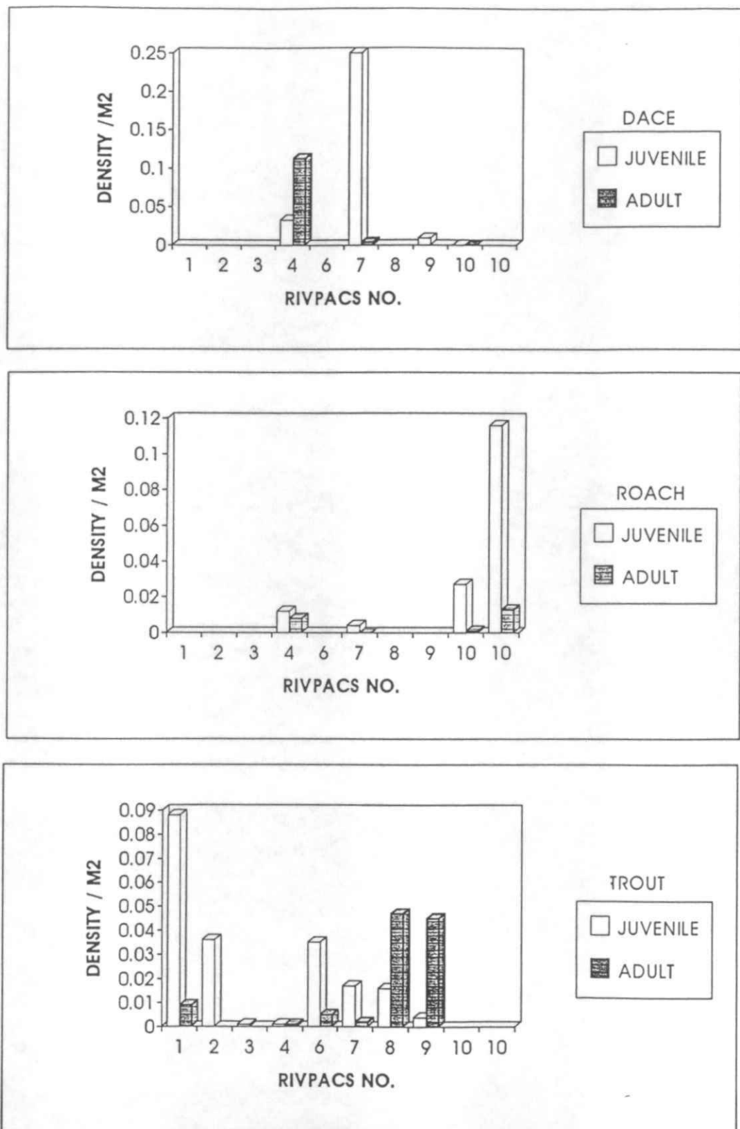
Figure 5 Densities of target fish species
