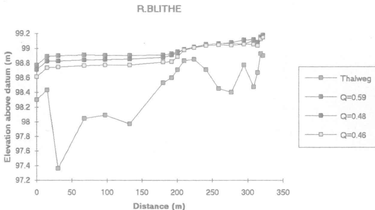
Figure C7 Observed Water Surface Profiles at Calibration Discharges: River Blithe
