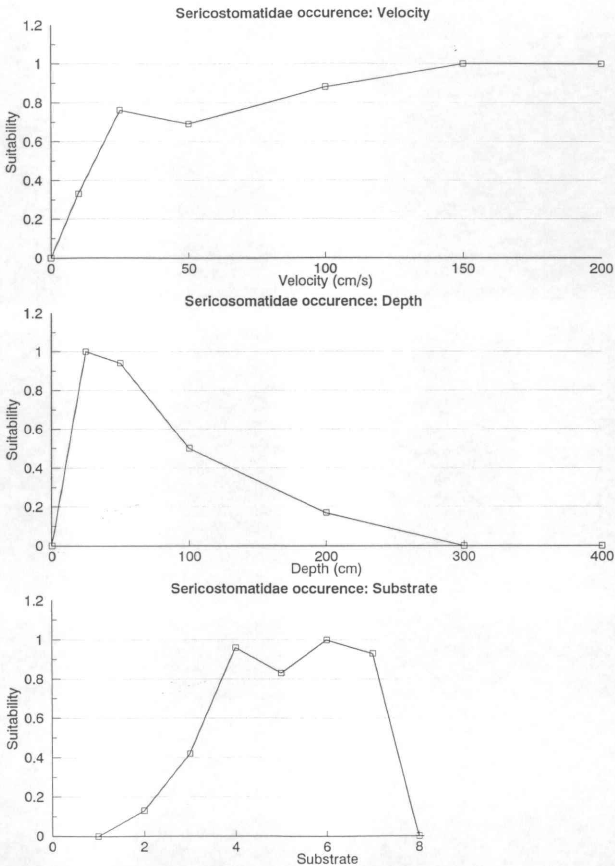
Figure B11 Habitat suitability curves: Sericostomatidae occurrence
