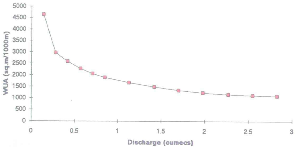
Figure 7.4 Habitat vs Discharge Relationships : River Blithe (contd.)
