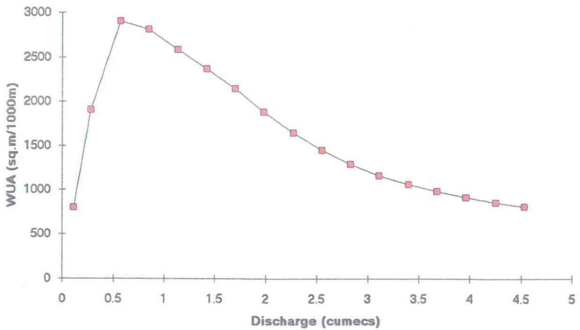
Figure 7.7 Habitat vs Discharge Relationships : Mill Stream (contd.)
