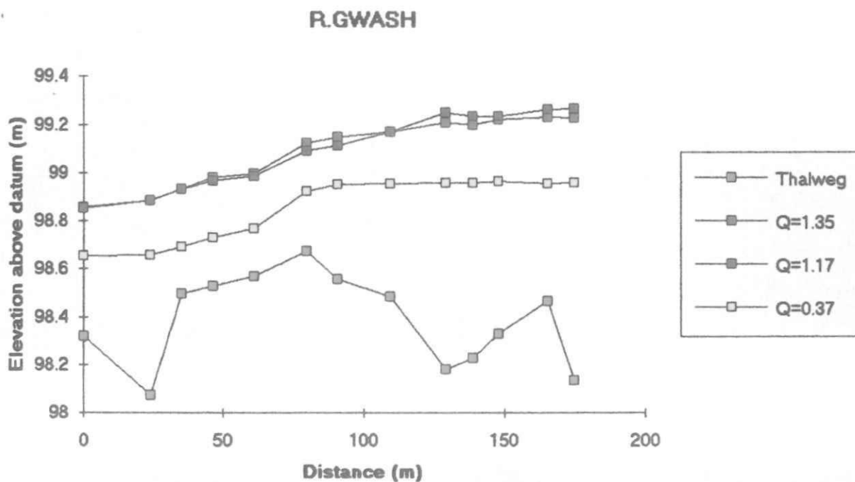
Figure C17 Observed Water Surface Profiles at Calibration Discharges: River Gwash
