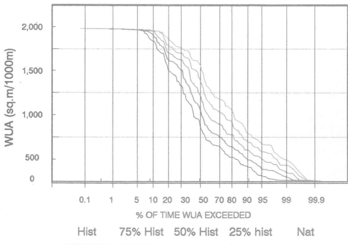
Figure 8.9 Duration Curves for WUA for juvenile/fry trout under alternative abstraction regimes, R.Allen downstream site. 1970-1991, summer months
