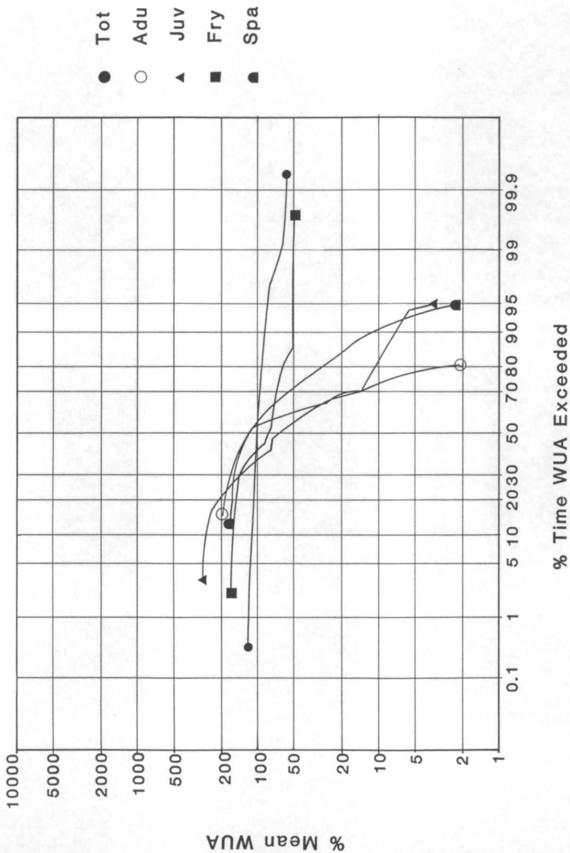
Figure 7.11 Weighted Usable Duration Curves : Dace, Mill Stream
