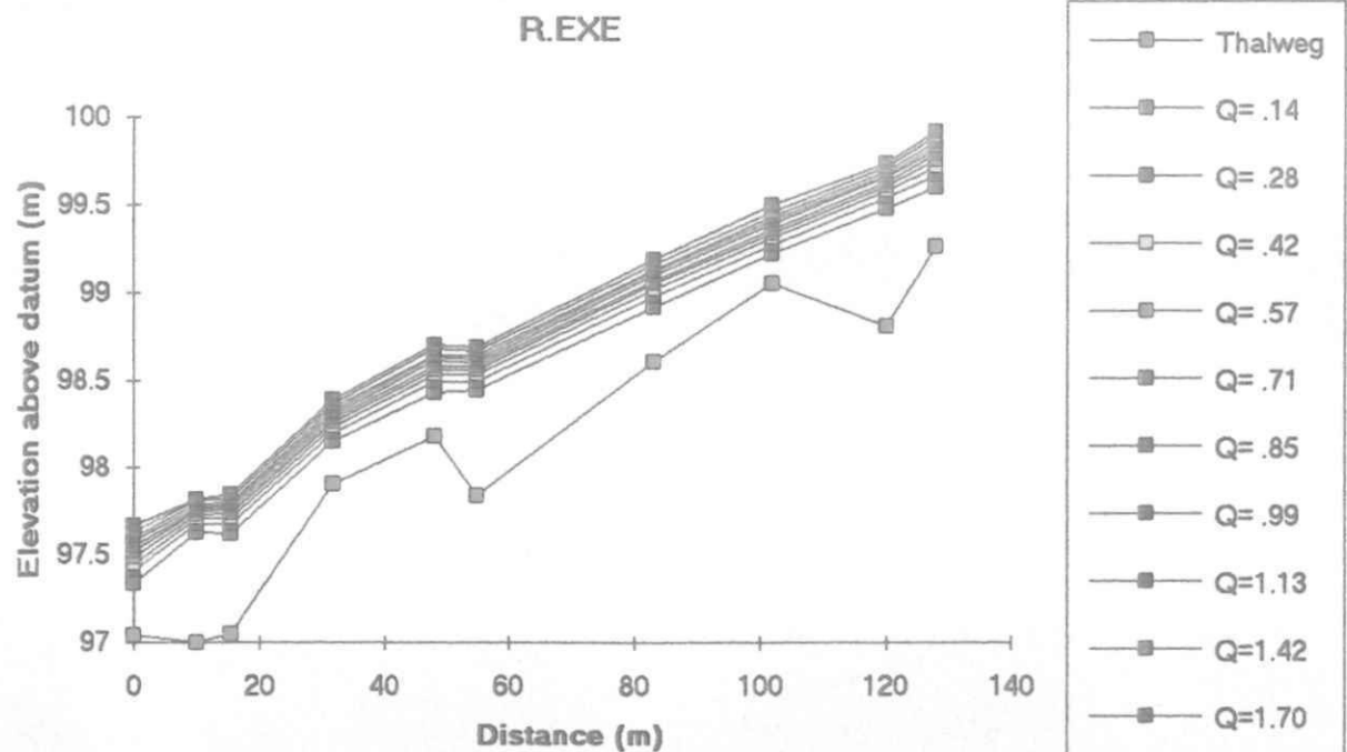
Figure C2 Predicted Water Surface Profiles at Simulation Discharges: River Exe
