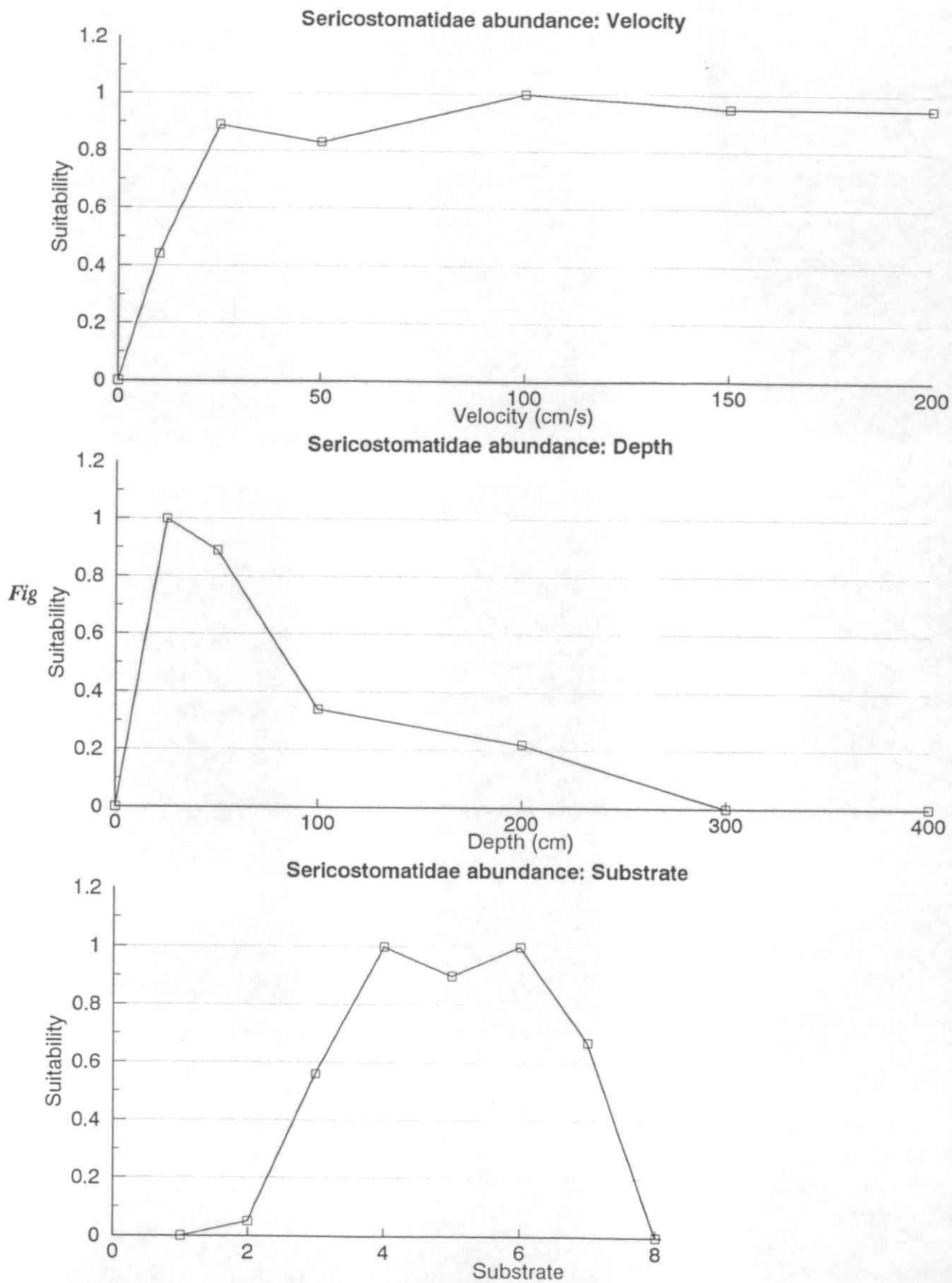
Figure B12 Habitat suitability curves: Sericostomatidae abundance
