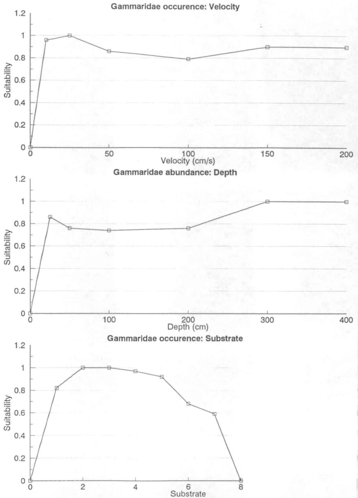
Figure B15 Habitat suitability curves: Gammaridae occurrence
