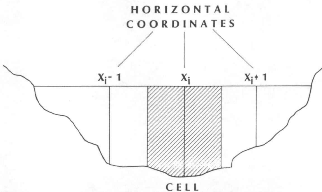
Figure 2.3 Cell areas defined by survey points placed across a transect
