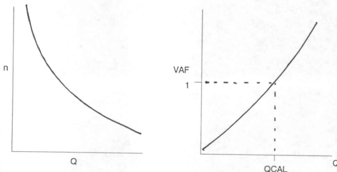
Figure 6.2 Theoretical Shape of n vs Q and VAF vs Q
