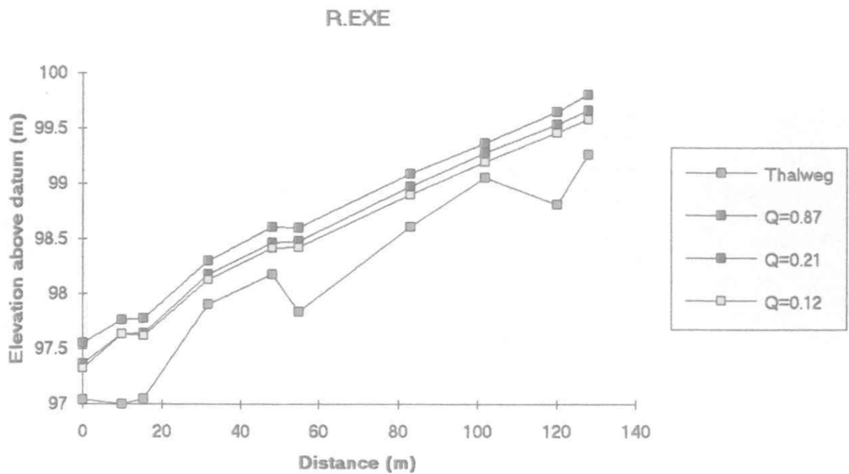
Figure C1 Observed Water Surface Profiles at Calibration Discharges: River Exe
