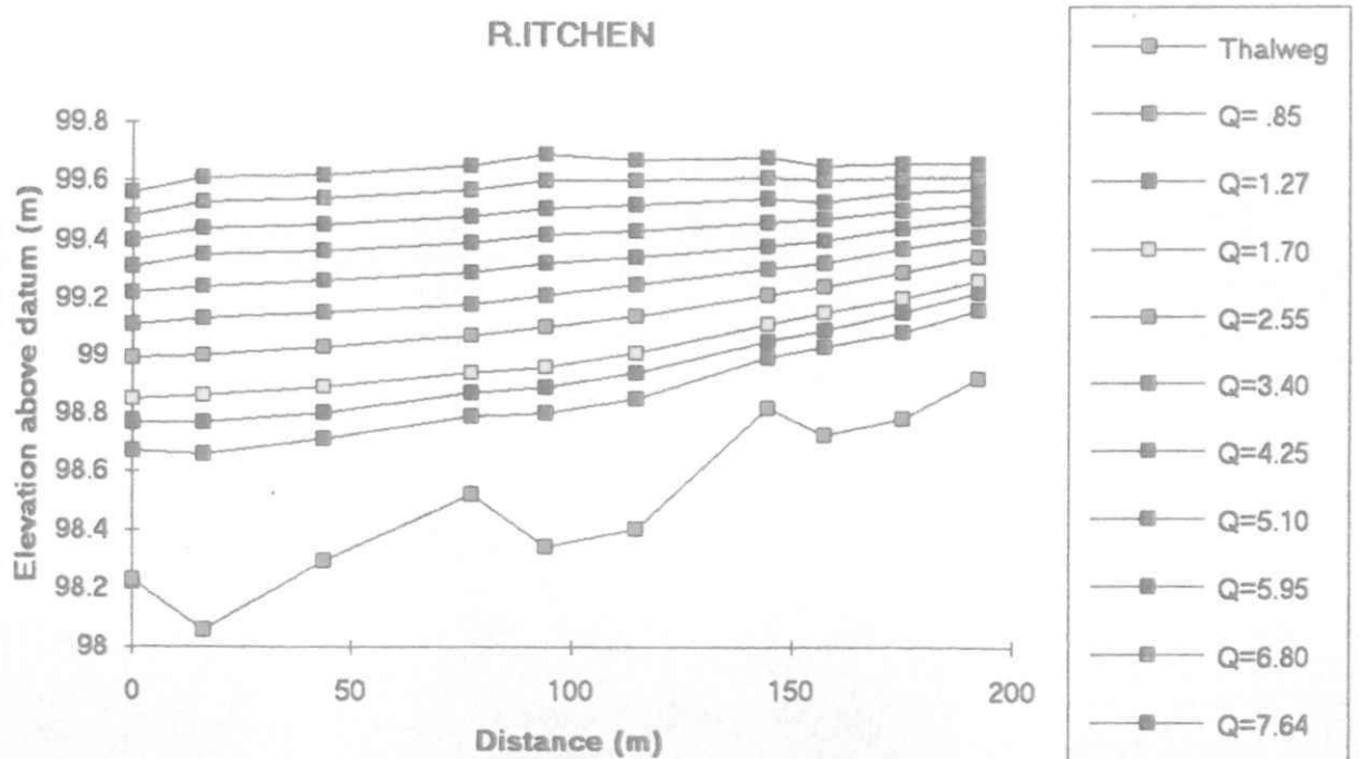
Figure C10 Predicted Water Surface Profiles at Simulation Discharges: River Itchen
