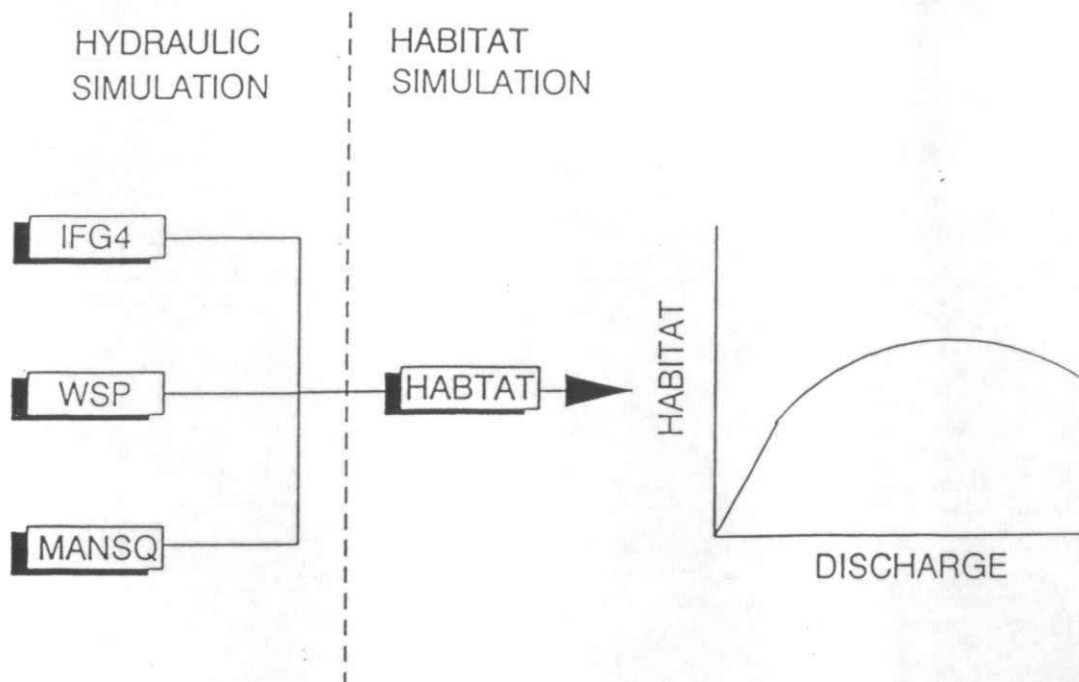
Figure 2.1 Flow of Information Through PHABSIM model
