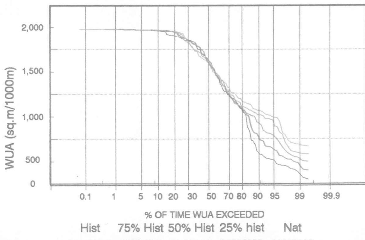
Figure 8.10 Duration Curves for WUA for juvenile/fry trout under alternative abstraction regimes, R.Allen downstream site. 1970-1991, winter months
