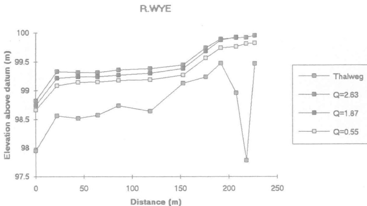
Figure C3 Observed Water Surface Profiles at Calibration Discharges: River Wye
