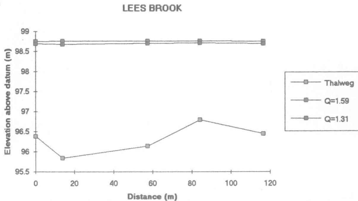
Figure C21 Observed Water Surface Profiles at Calibration Discharges: Lees Brook
