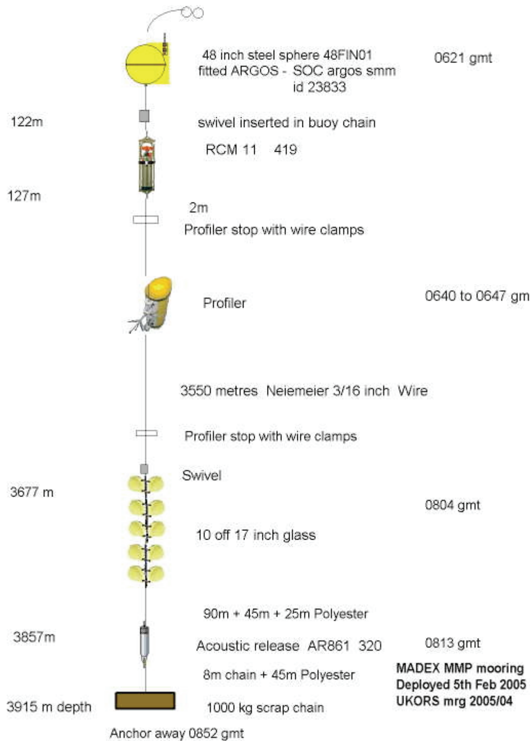
Figure 33 : Schematic for mooring UKORS 2005/04 (McLane Moored Profiler).
