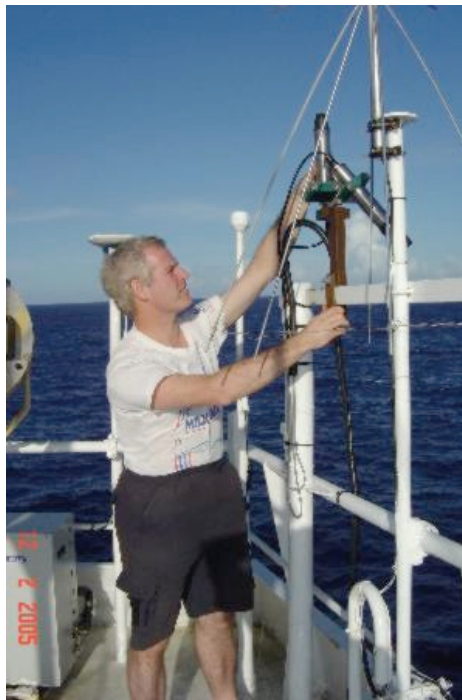
Figure 29 : Hyperspectral radiometers were attached to the starboard side of Monkey Island on RRS Discovery, giving the downward-looking one a clear view of the water ahead of the ship's wake.
