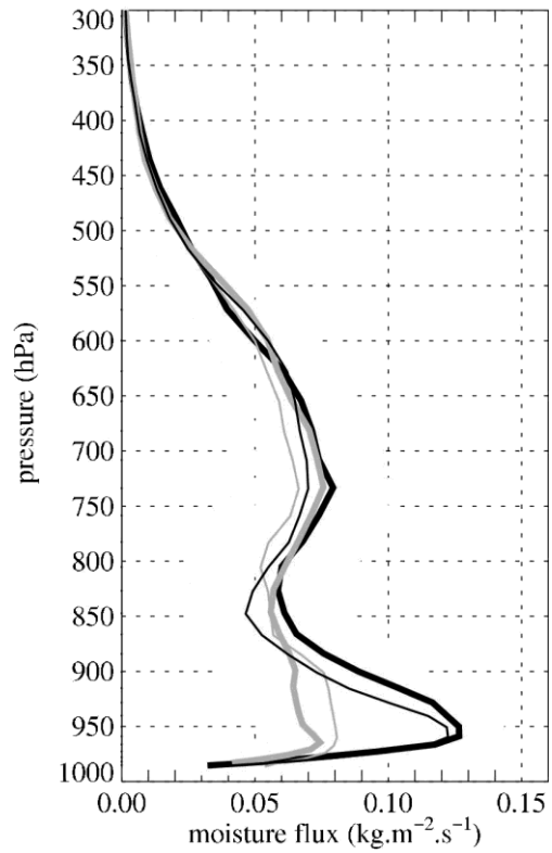
Fig. 9. Composite moisture flux V.q.p from all radiosonde profiles from Niamey for August 2006. Soundings at 12 UTC are represented by the thin/grey line, 18 UTC are bold/grey, 00 UTC are thin/black and 06 UTC are bold/black lines. Shading represents \pm standard deviation.
