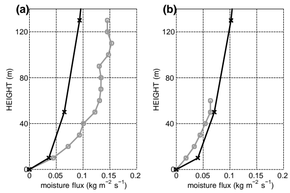
Fig. 8. Mean night time moisture flux ( \overline{V \cdot q \cdot \rho} ) comparisons in \text{kg m}^{-2} \text{s}^{-1} , from the evenings of 11 (a) and 18 (b) August 2005: observations in grey and UM in black.
