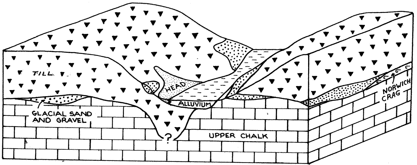
Fig.1. Idealised diagram showing relationships between the main lithostratigraphical units. Not to scale.
