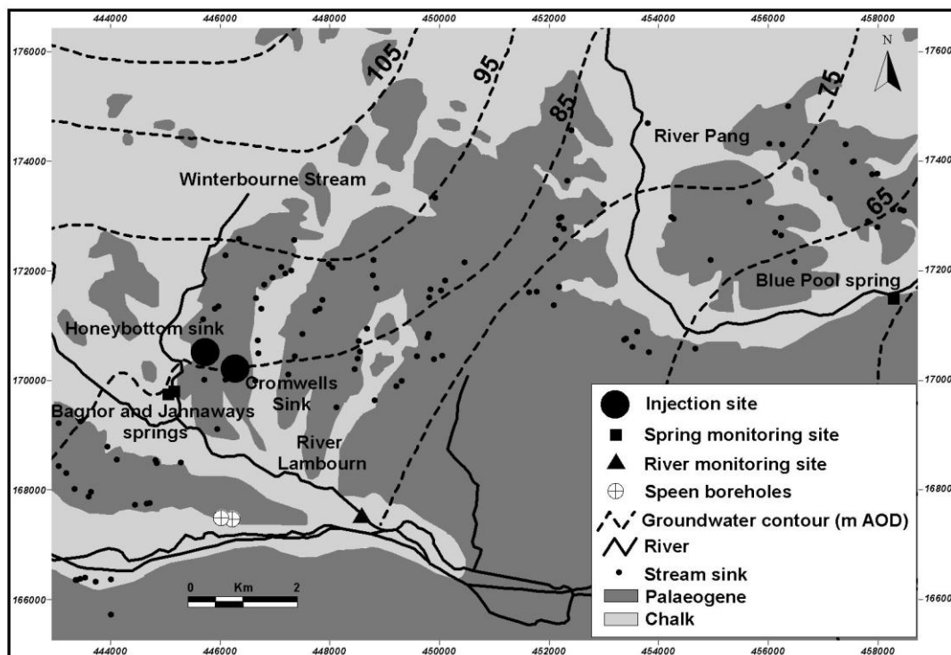
Figure 2: Tracer testing in the Winterbourne catchment
