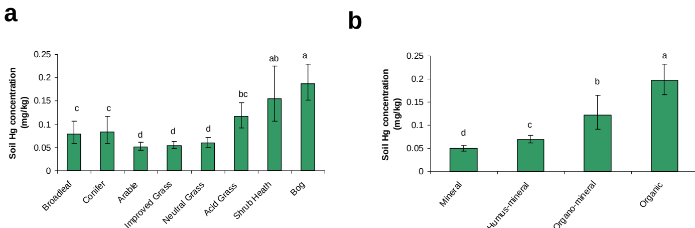
Figure 7.13: Measured soil Hg concentration (+/- 95% CIs) in soils (0-15 cm depth) within a) Broad Habitats, b) Soil LOI categories across Great Britain. Columns not sharing the same letter are significantly different at p < 0.05 level.
