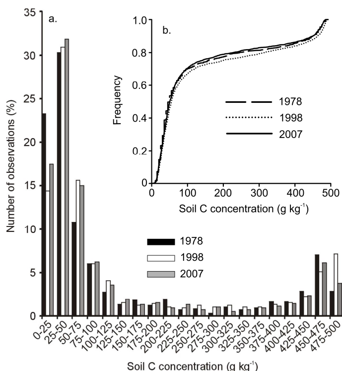
Figure 2.4: Distribution of Countryside Survey soil C concentration data (0-15cm) (a) Number of observations for 25 g kg -1 divisions, (b) Cumulative frequency.
