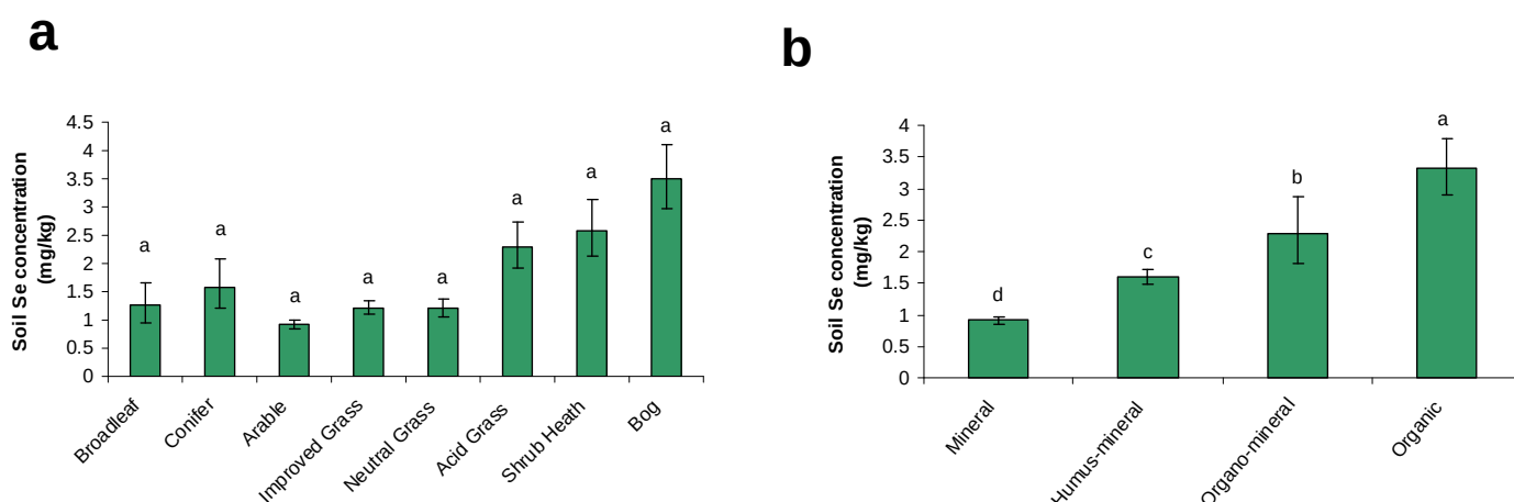
Figure 7.15: Measured soil Se concentration (+/- 95% CIs) in soils (0-15 cm depth) within a) Broad Habitats, b) Soil LOI categories across Great Britain. Columns not sharing the same letter are significantly different at p < 0.05 level.
