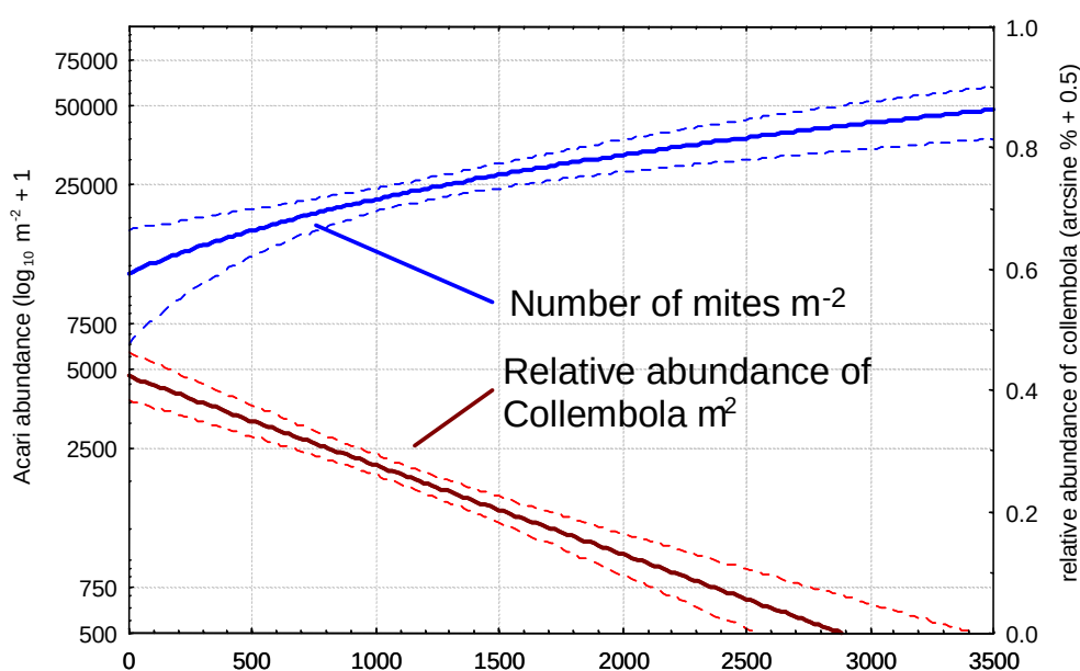
Figure 8.4: Mite abundance and relative abundance of Collembola in relation to mean annual precipitation. Trends (with 95% confidence intervals) are calculated based on data collected from 1097 Tullgren samples collected across GB in 1998.
