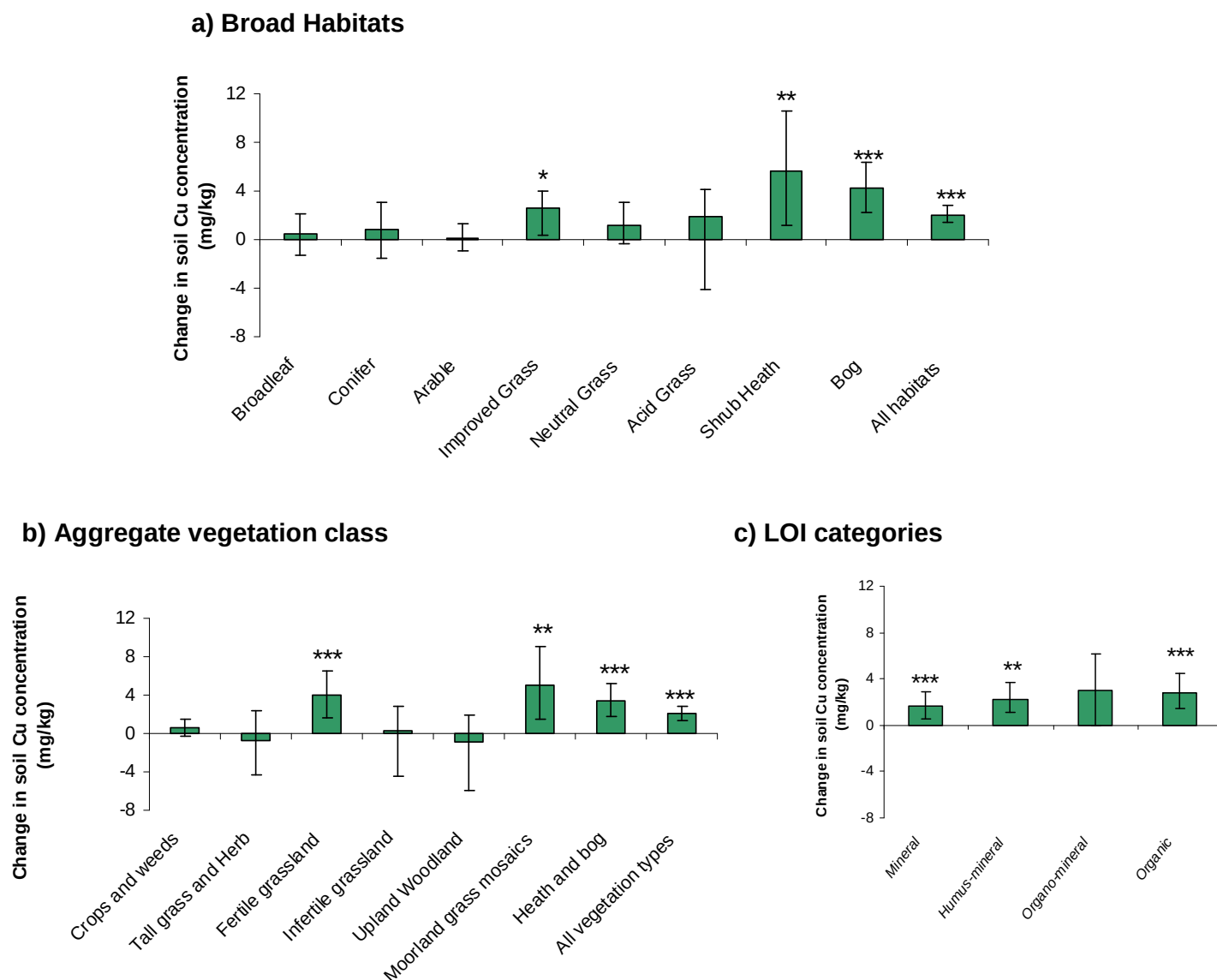
Figure 7.5: Changes (+/- 95% CIs) in measured soil Cu concentration in soils (0-15 cm depth) within a) Broad Habitats, b) Aggregate Vegetation Classes and c) Soil LOI categories across Great Britain. Standard errors are indicated. Significant differences * p < 0.05 , ** p < 0.01 , *** p < 0.001 are shown.
