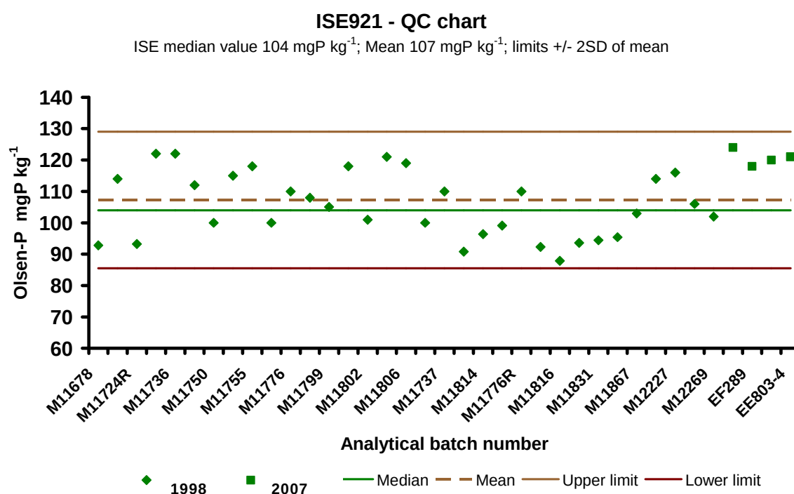
Figure 6.2: Shewhart QC chart for ISE standard reference soil ISE921 analysed with sample batches from CS in 1998 and Countryside Survey 2007.
