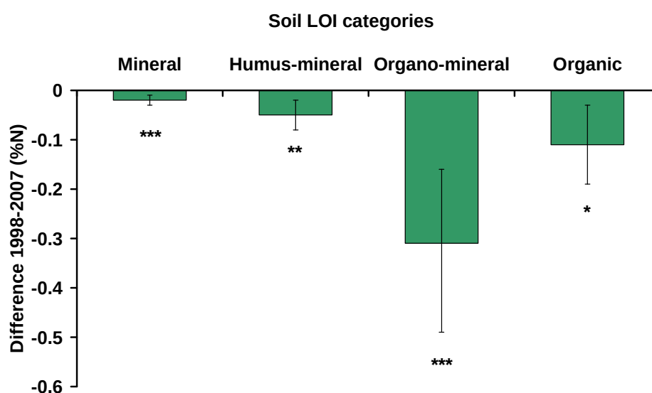
Figure 4.5: Change in soil (0-15 cm) N concentration across LOI categories in Great Britain between 1998 and 2007. Significant changes are shown as *** p < 0.001 ; ** p < 0.01 ; * p < 0.05 . 95% CI are shown for each bar.
