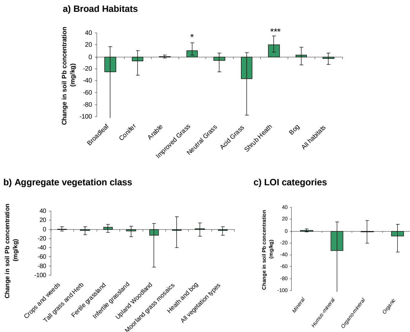
Figure 7.7: Changes (+/- 95% CIs) in measured soil Pb concentration in soils (0-15 cm depth) within a) Broad Habitats, b) Aggregate Vegetation Classes and c) Soil LOI categories across Great Britain. Standard errors are indicated. Significant differences * p < 0.05 , ** p < 0.01 , *** p < 0.001 are shown.
