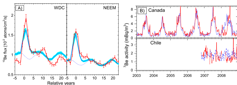
Fig. 30 Comparison of modelled and measured concentrations of beryllium isotopes for different time scales and conditions. Panel (A): Annual depositional fluxes of ^{10}\text{Be} at two sites analyzed for the period around 774 CE over the WDC (Antarctica) and NEEM (Greenland) stations. Red lines with error bars depict the measured data, while blue lines depict the modelled ^{10}\text{Be} flux. Years are given relative to the peak year (775 CE). Plot is modified after Sukhodolov et al. (2017) Panel (B): modelled and measured ^7\text{Be} concentrations in the near-ground air at the locations of four measurement stations in Canada and Chile. The measured and modelled data are shown as solid red and dashed blue curves, respectively. The plot is modified after Golubenko et al. (2021)
