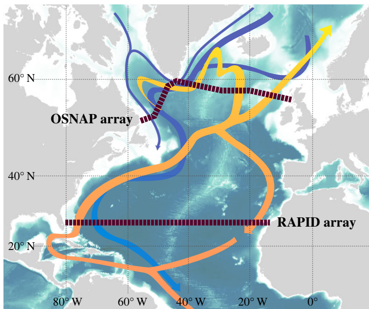
Figure 1. Highly simplified schematic of the overturning in the North Atlantic showing the location of the OSNAP and RAPID observing arrays. Orange and yellow colours depict the warm surface waters flowing north, while blue colours show the deep return flows.
