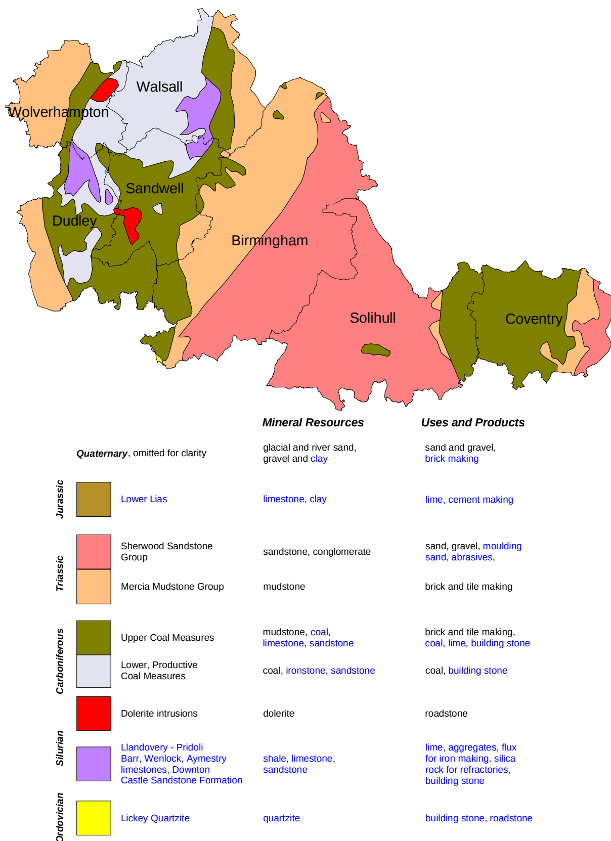
Figure 1 Simplified geological map of the former county of the West Midlands. Based on 1:625 000 Geological Survey Ten Mile Map, South Sheet (Solid) and 1:250 000 Mid-Wales and Marches Solid Geology. Commodities and their resources which are no longer worked are shown in blue text.
