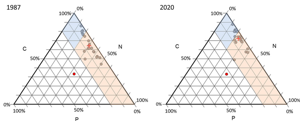
Figure 3. Ternary plots showing the relationships between C, N and P for all twenty sites (black circles) at the start (1987, left panel) and end (2020, right panel) of the monitoring period. The red cross indicates the mean of all twenty sites. The red point at the center of the plot marks the Redfield ratio (C:N:P 106:16:1) as a reference point. The pale orange trapezoid marks the region where P is depleted relative to N and/or C and the pale blue diamond marks where P and N are co-depleted relative to C (regions defined in Smith and others (2017) and Jarvie and others (2018)).
