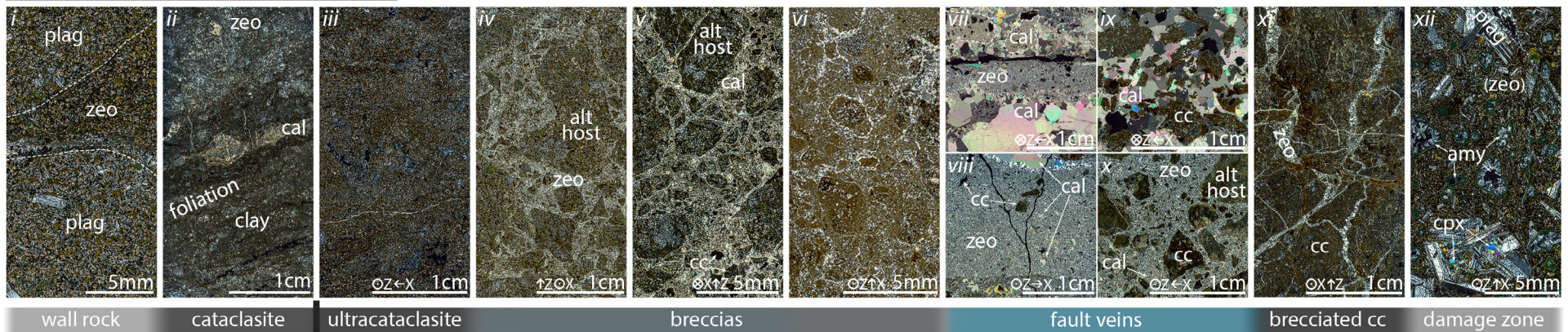
Figure 9. Microstructures as found along fault transects. 1. In the low displacement Í Botni (IBO) fault zone, slip surfaces separate mosaic (i) and chaotic (ii) breccias with partially altered matrix from a slip zone with strongly altered and cemented breccia (iii) as well as an unconsolidated gouge (iv). 2. Gøtugjógv (i) hanging wall damage zone with fractures delimiting an area of zeolitized host in otherwise unaltered host. (ii) Foliated hanging wall cataclasite from the slip zone with both clay- and zeolite-dominated matrix as opposed to (iii) thick, homogeneous ultracataclasite in the footwall. The footwall fault core contains lenses of chaotic breccia with altered host clasts in deformed zeolite (iv) or calcite (v) cement as well as (vi) reworked fault rock clasts and substantially more clay in the zeolitic cement. The fault core is also the site of significant veining (vii–x). Especially thick veins commonly host variable concentrations of wall-rock fragments (ix and x) but can also reactivate and rework older veins (vii). Their contacts are striated, and deformation is accommodated in a thin shear layer along the boundary (bottom of viii). (xi) Older cataclasite is reworked into a crackle breccia by irregular hydrofracture veins close to (xii) the essentially unaltered (minor matrix zeolitization) porphyritic damage zone basalt in the footwall. 3. Selatrað features highly altered and localized secondary faults in an otherwise weakly altered damage zone (i + right side of ii), similar to GOT xii. The slip zone is characterized by a homogeneous (ultra-) cataclasite with a clay-dominated matrix. Abbreviations: alt—altered, amy—amygdale, brec—breccia, cal—calcite, cc—cataclasite, plag—plagioclase, ucc—ultracataclasite, zeo—zeolite. See Figure 10 for textural details. All micrographs are in cross-polarized light.
