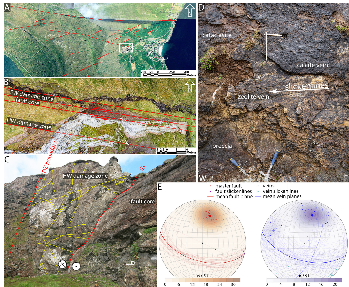
Figure 3. (A) The sinistral fault zone in Gøtugjógv ( 62^{\circ}11'11''\text{N} , 6^{\circ}45'47''\text{W} ) is surrounded by a wide array of small Riedel faults. (B) A diagonal transect from the hanging wall (HW) damage zone in the W to the footwall (FW) damage zone in the E is exposed in a disused quarry. The exposed footwall section, containing most of the fault core, is 50 m wide and up to 10 m high. (B and C) The exposed section is distinctly asymmetrical. The damage zone (DZ) is 10 m wide in the hanging wall as opposed to only 3 m in the footwall. The fault core, however, is mainly contained in the footwall, with a width of 2–3 m vs. 20–30 cm in the hanging wall. (C) The slip surface (SS) is strongly corrugated, exposing 3–4 marked asperities. The ruler for scale is 1 m long. (D) Large patch of fault-parallel veins that exploit the contact between two cataclasite lenses in the slip zone. The contact between the zeolite and calcite vein is smooth and heavily striated by sinistral slickenlines. Average orientation of slickenlines on the slip surface and veins is 104/08^{\circ} . Ruler is 40 \times 20 cm. (E) Average slip-surface orientation (red) is rather shallow for a strike-slip fault with 194/56^{\circ} and shows little scatter. The fault core hosts extensive veining (blue), which is predominantly parallel (74/91 veins) or orthogonal (17/91 veins) to the slip surface.
