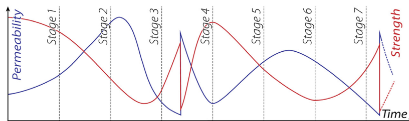
Figure 13. Hypothesized fault-parallel permeability (blue) and strength evolution (red). Stages are from Figure 12. Initial fracturing enhances permeability while strength is reduced (stages 1–2). Once a cataclastic slip zone is established, grain comminution and increasing clay concentration through alteration reduce permeability and lead to strain-hardening (stage 3), until eventually overpressurized, trapped fluids trigger hydrofracture. Cementation restrengthens the core and closes fluid pathways, quickly reducing permeability (stage 4). Reworking in the newly formed slip zone breaks up the cements, reducing strength, and initially increasing permeability (stages 5–6), until the reduced grain size, again, leads to strain-hardening and permeability loss (stage 7).
