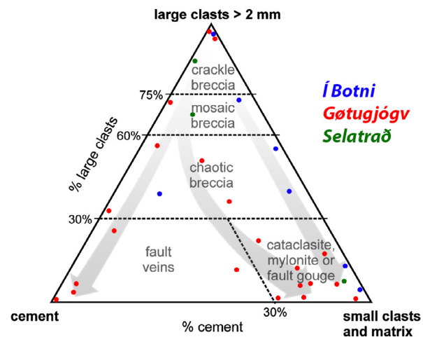
Figure 11. Plotting samples from all three fault zones in the fault rock classification diagrams by Woodcock and Mort (2008) shows that fault rock evolution roughly follows three trends: in the first phase of fault growth (Í Botni in blue), fault rocks are composed almost exclusively of host-rock clasts and comminuted matrix. In more mature faults (Gøtugjógv in red and Selatrað in green), the fault rocks range on a spectrum of cemented breccias spanning from crackle breccia to veins or diverge from this trend by accumulating fine-grained matrix through the cataclasis of clasts and cement from initial brecciation.
