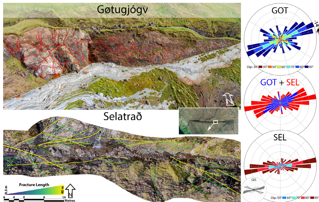
Figure 7. Comparison between secondary fault orientation in Gøtugjógv (GOT) and Selatrað (SEL). The Gøtugjógv rose plot was rotated 14° anticlockwise to match the E–W trend of Selatrað. The data plotted were measured in the field and on fault planes interpreted in the virtual outcrop models. They were given equal weight; i.e., half of the data are the field measurements, and the other half are virtual outcrop measurements. The pictures do not represent the plotted data but are rather examples of the general look of the fault zones. The Gøtugjógv data show a more balanced distribution between R, P, R', and X shears. Y shears are essentially absent because measurements from the slip surface were excluded. The Selatrað data are strongly dominated by Y and R shears, most likely because these are very prominent in the gorge, which introduces a bias in the field measurements. This becomes clear when comparisons are made to the lineament analysis performed in GIS (inset rose plot), which confirms R frequency recorded in the field and virtual outcrop but also has a similarly strong peak around the P orientation. In any case, we can see similar trends in both fault zones. R (and Y) shears are the dominant orientation with subordinate P shears and much less common high angle R' and X shears. Also see Figures 5F–5G for smaller scale structures.
