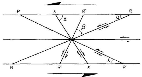
Figure 6. Typical Riedel shear (P, X, R', R, Y) configuration developed in simple shear (Logan, 1979).
