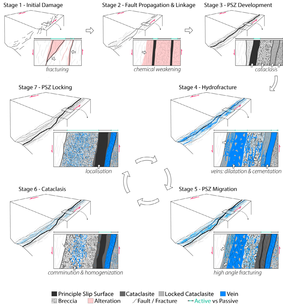
Figure 12. Simplified conceptual fault zone evolution in basaltic rock. (Stage 1, GOT i) Initial distributed damage leads to channeling of fluid flow and associated alteration and weakening of wall rock. (Stage 2, IBO i–iii) Fault strands linkage followed by slip localization into cataclastic principal slip zone (PSZ) increases permeability, initiating fluid-mediated alteration of fault rocks. (Stage 3, GOT iii and SEL i) Pervasive fault rock alteration leads to weakening and further slip localization and cataclasis. (Stage 4, GOT ix–xi) Progressive comminution and increasing clay concentration reduce PSZ permeability, culminating in fluid overpressure, hydrofracture, and mineralization/cementation. (Stage 5, GOT xi) The now-strengthened PSZ is abandoned, and slip migrates to a weaker part of the fault zone. (Stage 6, GOT v–vi) The abandoned fault rock is reworked by cataclasis in the vicinity of the newly localized slip zone and integrated into second generation breccia and cataclasite. (Stage 7) Similar to stage 3, cataclasis and alteration in the new PSZ, again, lead to a permeability drop, closing the cycle. (Second entry in parentheses refers to micrographs representing the respective stages in Fig. 9.)
