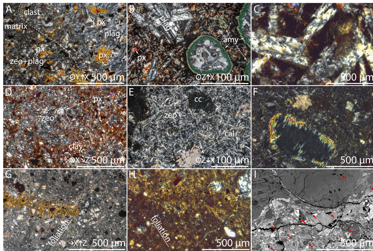
Figure 10. Photomicrographs of textural details: (A—IBO ii) Í Botni slip zone chaotic breccia with yet unaltered plagioclase in the clasts and partially zeolitized cataclastic matrix. (B—GOT xii) Gøtugjógv footwall damage-zone of relatively unaltered porphyritic basalt clast with zeolite-filled amygdalae and plagioclase phenocrysts in partially altered groundmass. (C—GOT iv) Botryoidal zeolite replaces plagioclase in a Gøtugjógv breccia clast. (D—GOT iii) Homogeneous footwall ultracataclasite from the Gøtugjógv slip surface. Shape-preferred orientation of zeolite crystals in veins (E—GOT viii) and cataclasite matrix (F—GOT ii) from Gøtugjógv. Also note the euhedral zeolite crystals growing into the calcite pocket in panel E. Foliation in zeolite (G—GOT iii) and clay-dominated (H—GOT ii) slip-surface ultracataclasite, Gøtugjógv. (I—GOT ii) Porosity in slip zone cataclasite from Gøtugjógv in scanning electron microscope—backscattered electron. Abbreviations: amy—amygdale, cal—calcite, cc—cataclastic, plag—plagioclase, px—pyroxene, zeo—zeolite. All micrographs except in panel I are in cross-polarized light.
