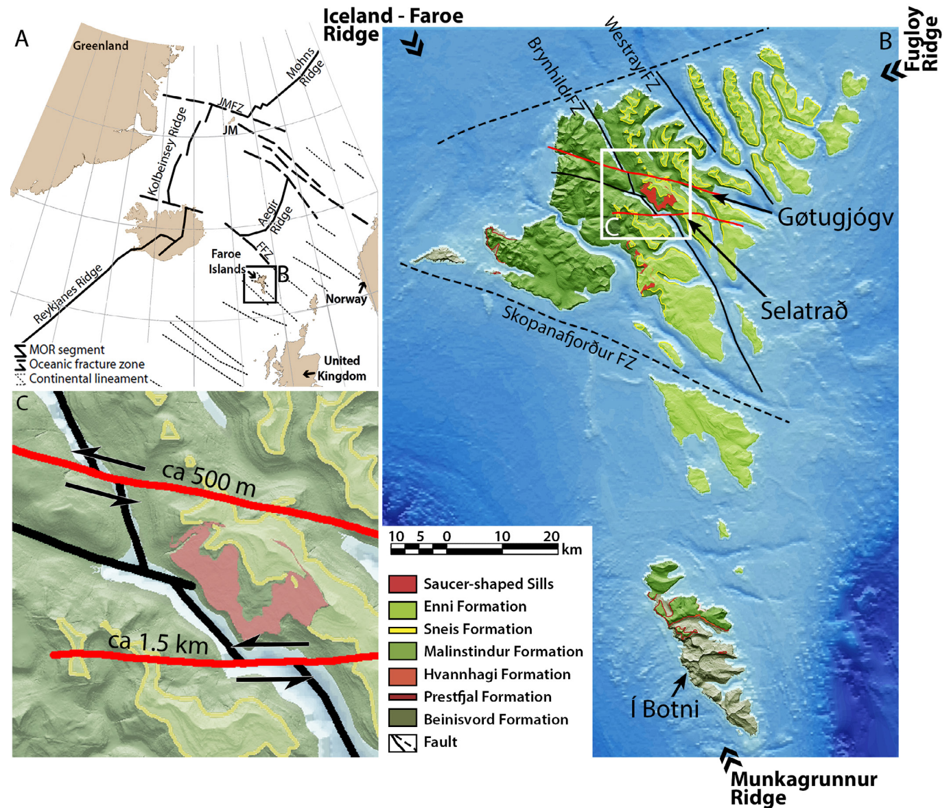
Figure 1. (A) Structural overview and geological setting of the Faroe Islands in the North Atlantic. (B) The archipelago sits at the intersection of three ocean ridges: the Iceland-Faroe Ridge to the NW, the Fugloy Ridge to the NE, and the Munkagrúnnur Ridge to the S (after Roberts and Walker, 2016). We focus on three fault zones in this paper: two large, sinistral strike-slip faults exposed in Gøtugjógv and Selatrað (Eysturoy) and a smaller normal fault exposed in Í Botni (on Suðuroy). (C) Close up of the fjord separating Eysturoy in the E from Streymoy in the W, which indicates the position of the major Brynhildr fault zone (FZ). It is offset by the Gøtugjógv and Selatrað fault zones, indicating potential displacements of 500 m and 1.5 km, respectively. FFZ—Faroes fracture zone, JM—Jan Mayen, JMFZ—Jan Mayen fracture zone, MOR—mid-oceanic ridge.
