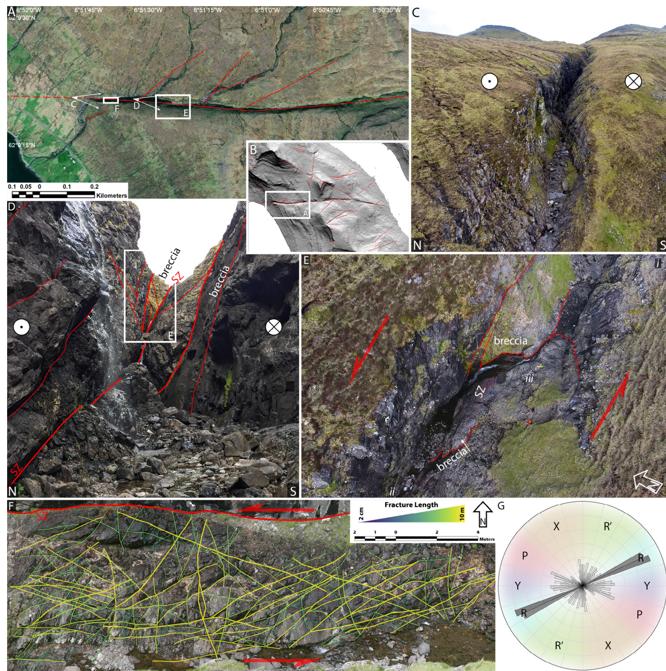
Figure 5. The sinistral Selatrað fault zone can be traced across (B) the entire southwestern peninsula of Eysturoy but is only exposed in two deep gorges on either coast. We focus on the western gorge (A and C, 62°9'19"N, 6°51'25"W). Smaller faults (in red) in the wider area follow Riedel orientation in (A) the direct vicinity but (B) are less organized farther away. (D) The overall topographic orientation of the gorge is 000/60° and is presumed to be indicative of fault zone orientation. Slip zone (SZ) and secondary faults mostly run parallel to this trend with a mean orientation of 000/71°. (D-E) The slip zone meanders through the fault zone, switching from (E) its southern edge on the upper tier exposed in the west to (D) the northern edge farther down. The slip zone and secondary faults bound lenses of fragmented, older fault rock. (F-G) Internal fracturing in these lenses is highly systematic and follows the typical Riedel orientation with a very strong dominance of R shears. Indices i-iii in panel E are locations of samples shown in Figure 9.
