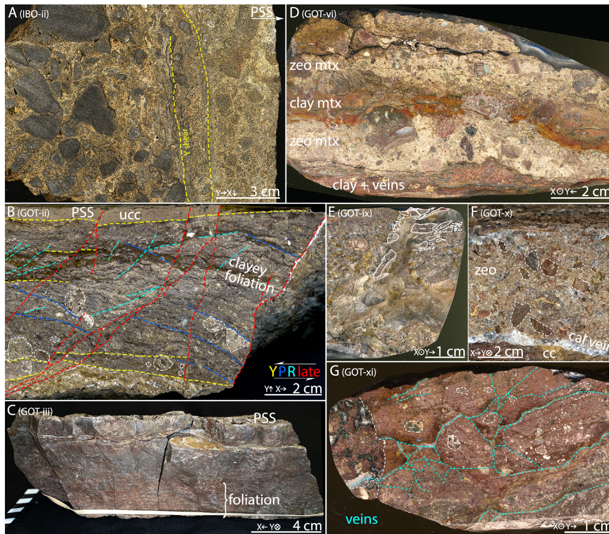
Figure 8. Specimen-scale structure of fault rocks: (A) transition from a coarse, chaotic breccia to finer breccia and protocataclasite a few centimeters away from the principle slip surface (PSS) in Í Botni. (B) The hanging wall slip zone (sinistral in picture) in Gøtugjógv (GOT) is defined by a thin layer of ultracataclasite (ucc) separated by Y shears (yellow) from a 5-cm-thick cataclasite with a clayey foliation along P (blue) and R (teal) shears. Both the foliation and the contact are transected by late-stage, high-angle shears (red). (C) The footwall slip surface, on the other hand, is a >5-cm-thick layer of homogeneous ultracataclasite with a very weak foliation on the far side, which is not distinguishable in thin sections. The boundary cutting across the sample parallel to the slip surface is a tabular zeolite-calcite vein. (D) Chaotic breccia of generally fine grained (<5 mm) clayey fault rock clasts in a zeolite or zeolite + clay matrix (zeo/clay mtx). (E–F) Hydrofractured, chaotic breccia with fault rock clasts (outlined in white) in (E) coarse, equant calcite or (F) fine acicular-bladed zeolite cement. (G) Red (ultra-) cataclasite hydrofractured into a crackle breccia with thin zeolite veins. Exemplary clasts are outlined in white.
