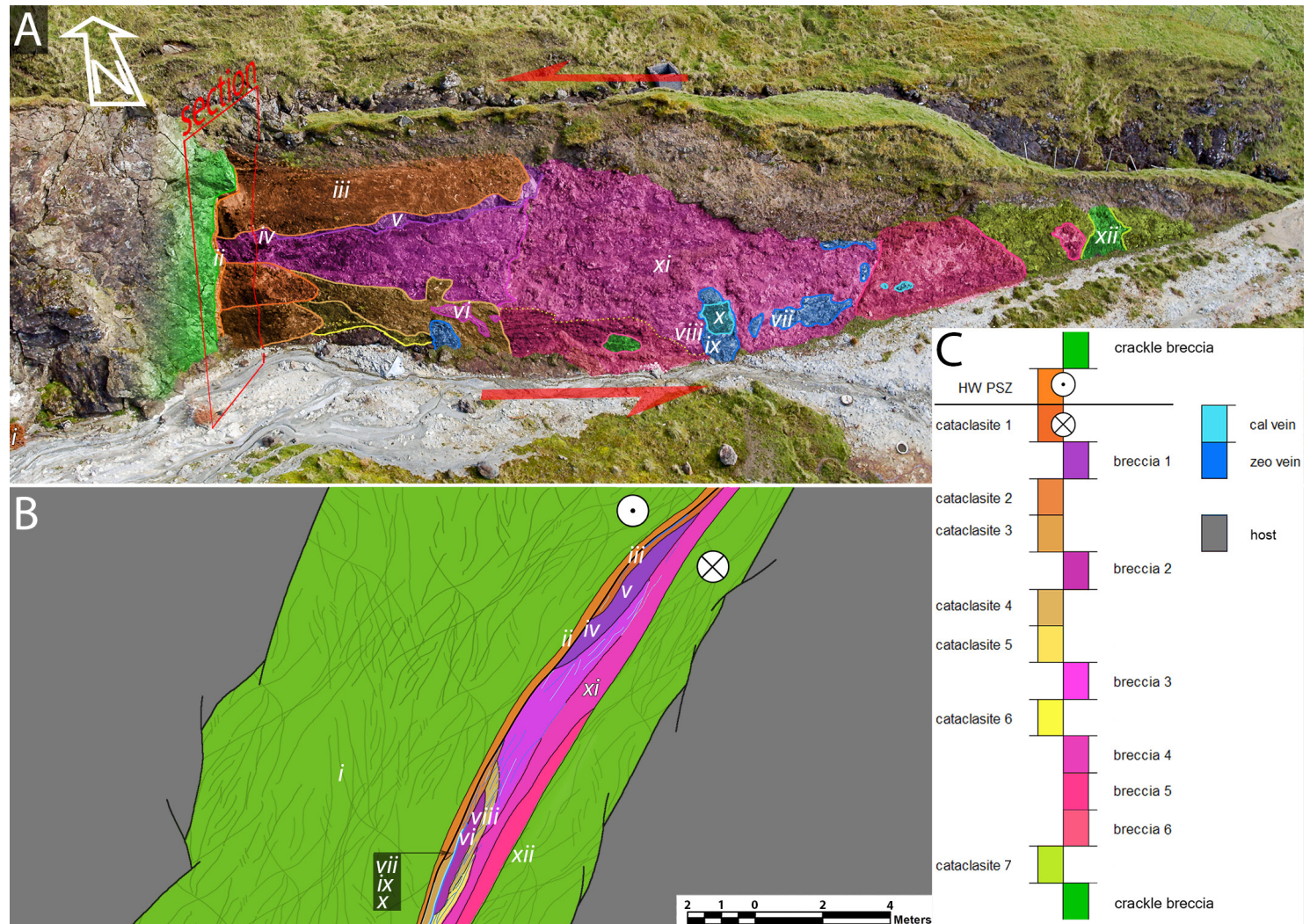
Figure 4. Fault rock distribution in the Gøtugjógv fault zone (A) in the field and (B, legend in C) in a stylized section. The damage zone is mainly composed of a coarse crackle breccia with unaltered host-rock clasts. This is contrasted by the highly altered and reworked fault core material that is composed of lenticular fault rock bodies separated by cataclastic shear bands and/or veins. Close to the principal slip zone, these fault rock lenses mostly contain cataclasite. Closer to the damage zone, breccias become more prevalent. They are almost exclusively the result of hydrofracture and are cemented by zeolite or calcite with a texture similar to that of vein cements. Indices i–xii refer to samples and micrographs in Figures 8 and 10. HW—hanging wall, PSZ—principal slip zone.
