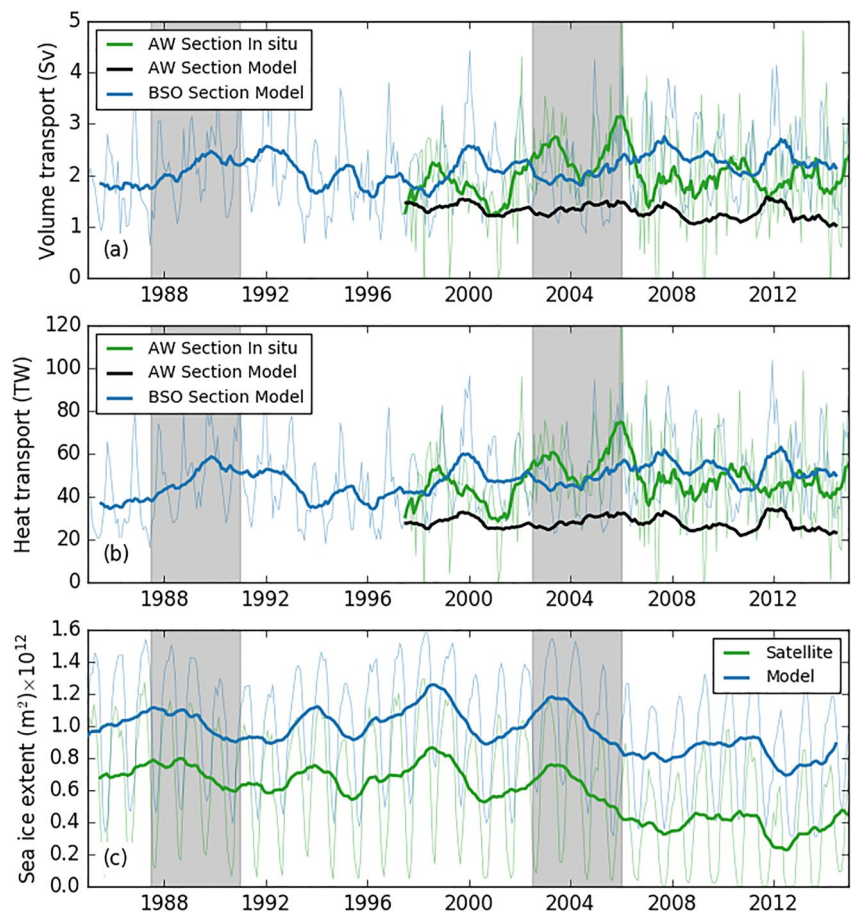
Figure 3. (a) Volume and (b) heat transport through the Barents Sea Opening (Fugløyaa–Bear Island section along 20.0°E). The green line shows the observations of Atlantic Water transport ( T > 3^{\circ}\text{C} and depth > 50 m) across the black dashed line in Figure 1, the black line shows the model estimate using the same Atlantic Water definition (See Section 2.3), the blue line shows model estimate across the Barents Sea Opening (Barents Sea Opening, blue line in Figure 1) with depth > 50 m but without a temperature criteria. (c) Sea ice extent within the Barents Sea ( 68^{\circ}\text{N} – 80^{\circ}\text{N} and 10^{\circ}\text{E} – 65^{\circ}\text{E} ) for model and satellite observations (white line in Figure 1). In all cases, thin line show monthly data and thick lines show 12-month running means. The gray bars highlight periods of interest July 1987 to December 1991 and July 2002 to December 2005 events.
