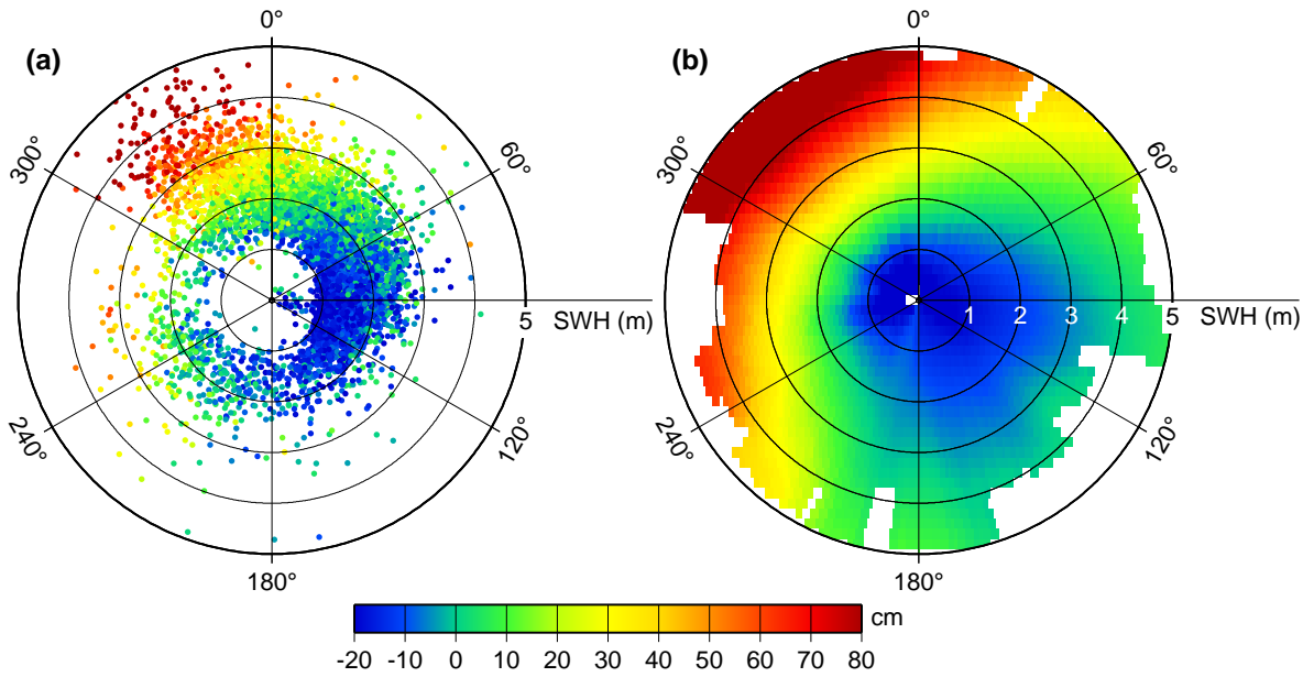
Fig. 5 (a) Color-coded sea-level differences between tide gauge and altimetry plotted as a function of swell wave height and direction. Each point represents one daily observation. The zero level for the sea level is arbitrarily set so that the mean sea-level difference is zero. (b) Gridded and smoothed version of the data in panel (a). This two-dimensional function of swell height and direction can act as an empirical model of wave setup at the tide gauge.
