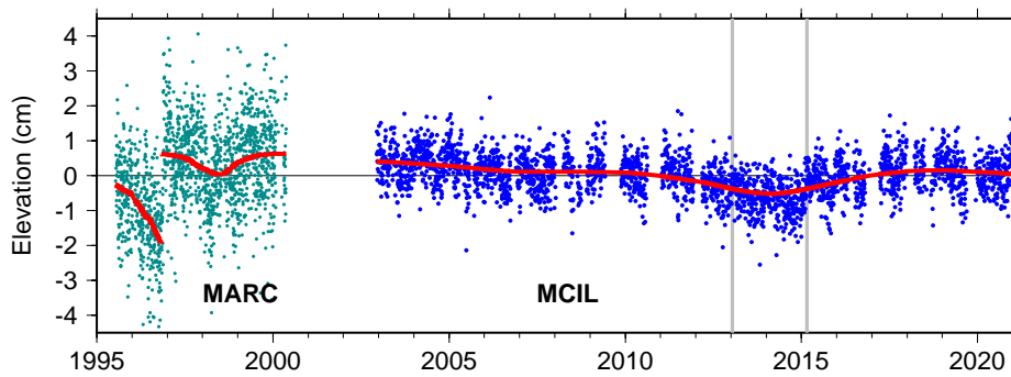
Fig. B1 Daily vertical elevations from two GNSS stations at Minamitorishima, as determined by Blewitt et al. (2018). The time series from each receiver has been demeaned. Heavy red lines are the result of a loess smoother applied to the daily data, with the break in late 1996 subjectively chosen. Grey vertical lines mark times of equipment change for the MCIL station. The MARC station employed older, now obsolete, equipment, which likely contributes to the much larger scatter.
