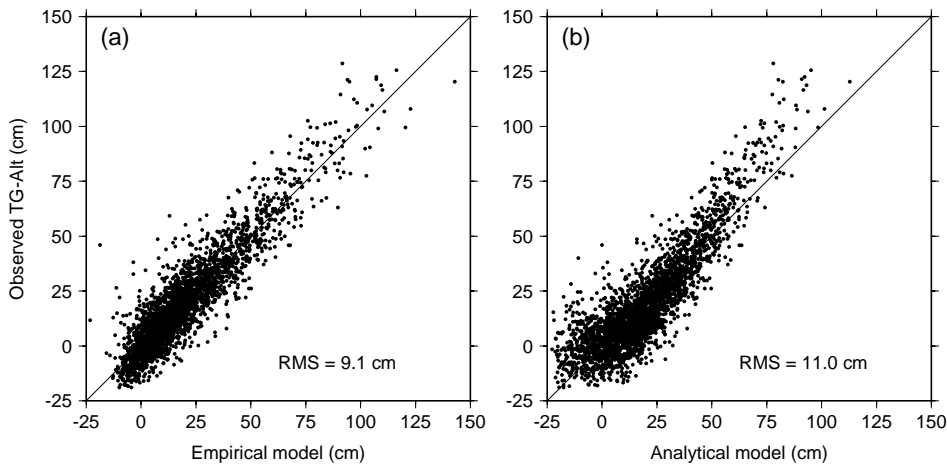
Fig. 9 Scatter diagrams of predicted wave setup versus observed daily tide-gauge/altimeter sea-level differences, based on (a) the empirical model of Section 5.1 and (b) the semi-analytical model of Section 5.2. Both panels are limited to swell directions within 90^\circ of 308^\circ , because model (b) is applicable only in that range.
