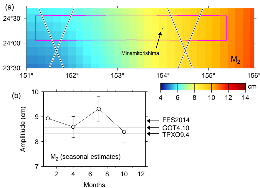
Fig. C1 (a) Ground tracks of the Topex-Jason satellites near Minamitorishima, shown over a color background of the M_2 tidal amplitudes according to global model TPXO9.4 (S. Y. Erofeeva, personal communication). (b) Mean quarterly estimates of the M_2 tide derived from all Topex-Jason data falling within the magenta box of the top panel. The tide and its spatial gradients were computed, with the latter used to interpolate to the island location. At right are the amplitudes from several widely-used global models, showing generally consistent agreement and larger than the mean tide reported at the tide gauge at its old position (Figure 10).
