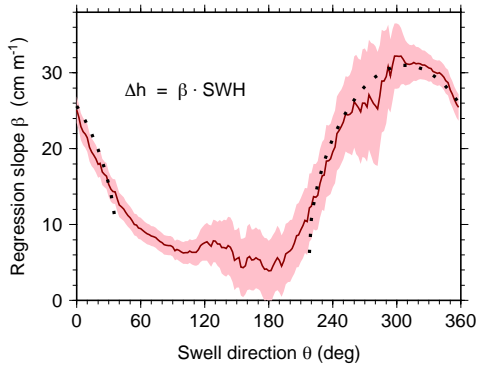
Fig. 6 Estimated linear relationship between setup anomalies and significant wave height (SWH) of swell, based on the data shown in Figure 5a. Shaded background marks uncertainties in the slope estimates; they have been roughly scaled to account for serial correlation in the data, based on the autocorrelation (approximately 0.83) of the entire daily tide gauge series. The dotted line represents a functional dependence on direction \theta according to [\cos(\theta - 308^\circ)]^{1/2} , valid only where the cosine is positive. This functional form follows Eq. (2), but here with slightly larger exponential (1/2 rather than 2/5).
