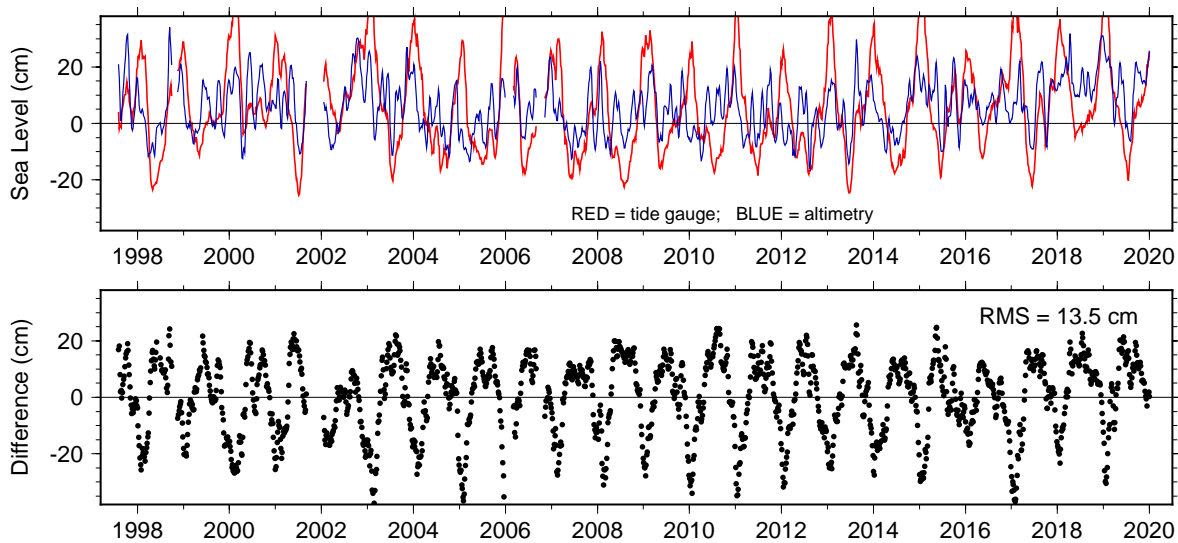
Fig. 2 (Top) Comparison of altimetric sea level measurements (from DUACS DT-2018; Taburet et al. (2019)) with daily mean sea levels from the Minamitorishima tide gauge (adjusted as described in Appendix A and smoothed to match approximately the temporal smoothing in the gridded altimetry). Relative bias is arbitrary. (Bottom) Difference in the sense altimeter minus tide gauge.
