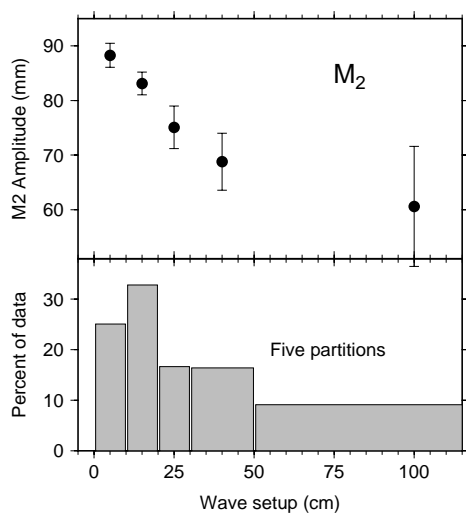
Fig. 11 Estimated amplitudes of the M_2 tide at Minamitorishima, from the western location, after breaking the hourly water-level time series into five partitions according to the wave setup at time of each measurement and subjecting each partition to independent tidal analysis. (Wave setup was determined by using our empirical model.) Bottom panel shows percentage of data falling into each partition, with their setup bounds in cm. The estimated amplitudes of M_2 decay with increasing wave setup. We conjecture that in reality the tide gauge is observing tidal variations in wave setup, which acts to suppress the measured tide as setup increases from offshore swell.
