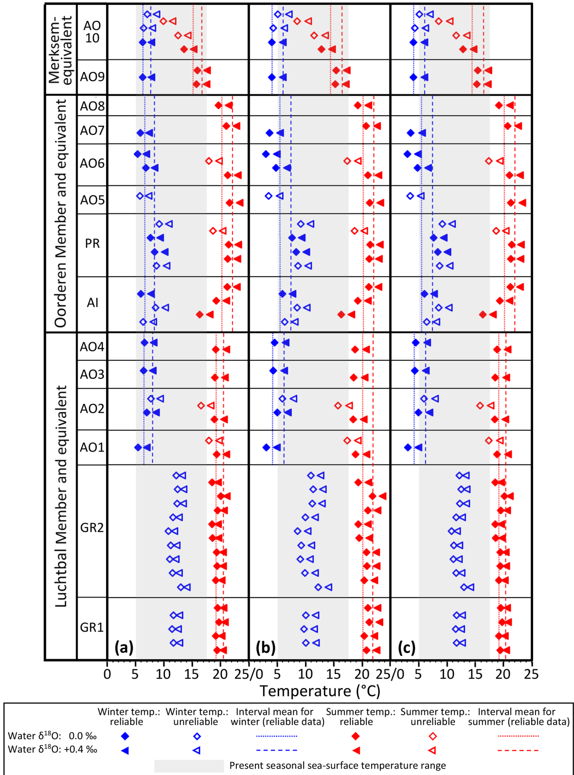
Figure 9. Winter and summer sea surface temperatures, calculated as in Fig. 8, using the same equations for (a), (b), and (c) but with a 3 °C supplement to Luchtbal and Oorderen summer temperatures in recognition of thermal stratification (see text, Sect. 6.1.3, for explanation). Interval means calculated as in Fig. 8. The indicated present-day seasonal sea surface temperature range (4.7–17.1 °C) is for 53° N, 03° E. Note that the Luchtbal and Oorderen ranges, as indicated by the separation of dotted or dashed lines for each interval, are larger than the present-day range (see text, Sect. 6.1.3, for more detailed discussion).
