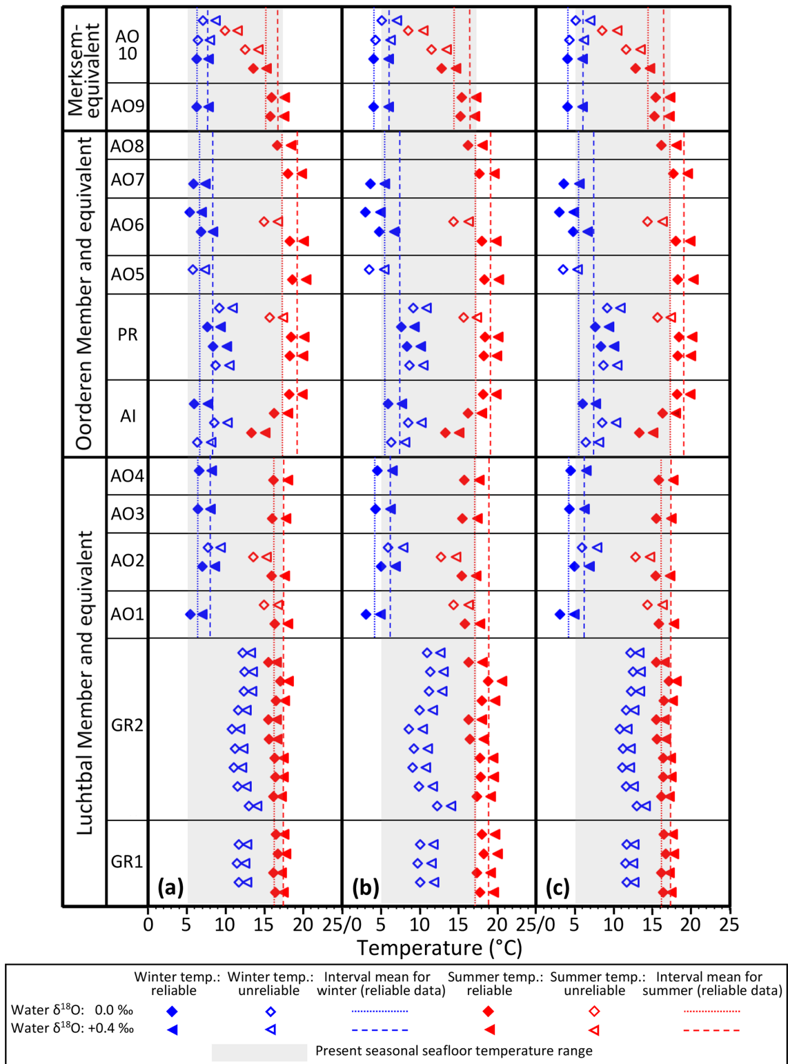
Figure 8. Winter and summer sea floor temperatures, calculated from the seasonal extreme \delta^{18}\text{O} values indicated in Figs. 6 and 7, using water \delta^{18}\text{O} values of 0.0‰ and +0.4‰ and various equations. (a) Equation of Royer et al. (2013) for GR, of O’Neil et al. (1969) for AO and of Grossman and Ku (1986) for AI and PR; (b) equation of Grossman and Ku (1986) for GR, AI, and PR and of Bemis et al. (1998) for AO; (c) equation of Royer et al. (2013) for GR, of Bemis et al. (1998) for AO, and of Grossman and Ku (1986) for AI and PR. Interval means are for reliable seasonal temperatures (see Sect. 6.1.1) from the Luchtbal Member and equivalent, Oorderen Member and equivalent, and Merksem-equivalent strata. The indicated present-day seasonal sea floor temperature range (4.7–16.9°C) is for 25 m depth at 53° N, 03° E.
